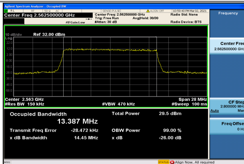
Band7-15MHz-16QAM-21375-75RB#0-13.387
