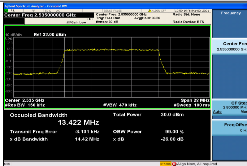
Band7-15MHz-16QAM-21100-75RB#0-13.422
