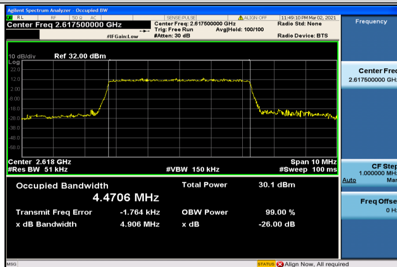
Band38-5MHz-QPSK-38225-25RB#0-4.4706
