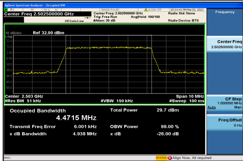
Band7-5MHz-16QAM-20775-25RB#0-4.4715
