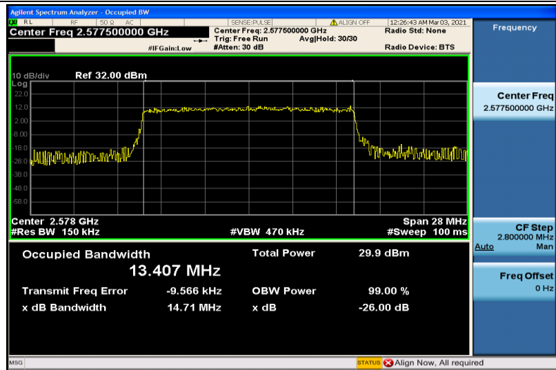
Band38-15MHz-16QAM-37825-75RB#0-13.407
