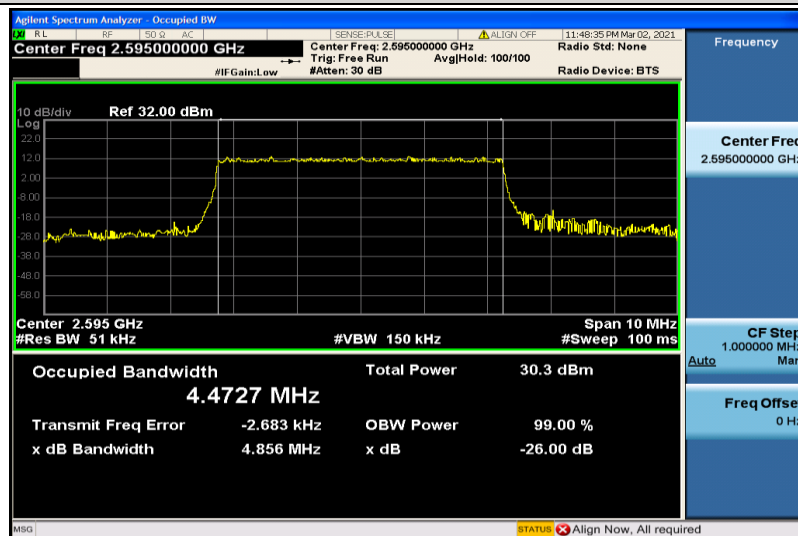
Band38-5MHz-QPSK-38000-25RB#0-4.4727
