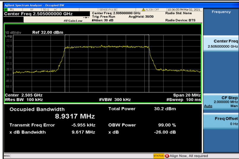
Band7-10MHz-16QAM-20800-50RB#0-8.9317
