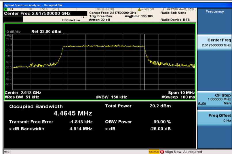
Band38-5MHz-16QAM-38225-25RB#0-4.4645
