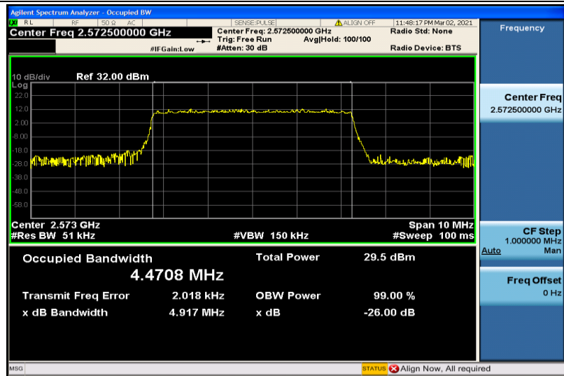
Band38-5MHz-16QAM-37775-25RB#0-4.4708
