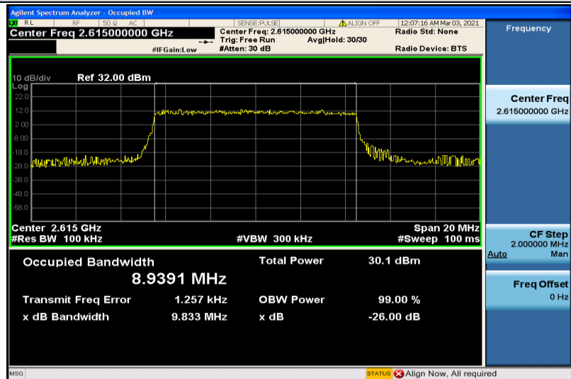
Band38-10MHz-QPSK-38200-50RB#0-8.9391
