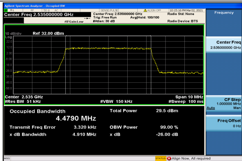
Band7-5MHz-16QAM-21100-25RB#0-4.4790
