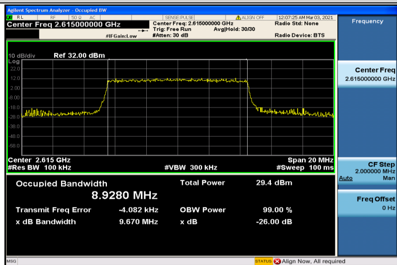
Band38-10MHz-16QAM-38200-50RB#0-8.9280
