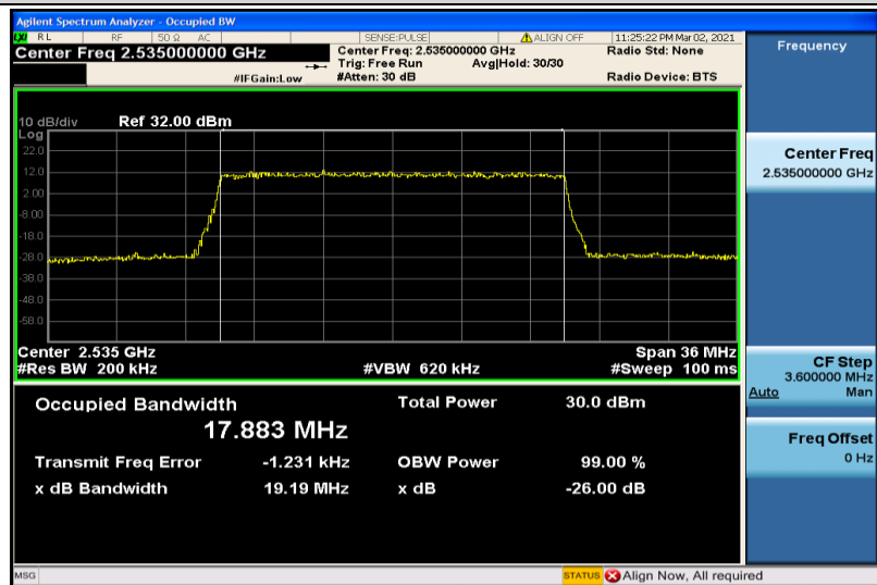
Band7-20MHz-16QAM-21100-100RB#0-17.883
