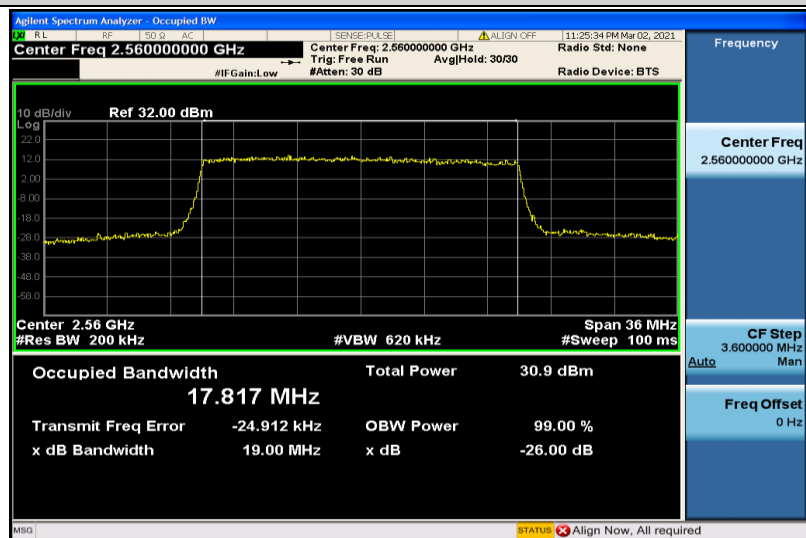
Band7-20MHz-QPSK-21350-100RB#0-17.817
