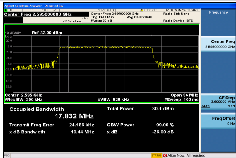
Band38-20MHz-16QAM-38000-100RB#0-17.832
