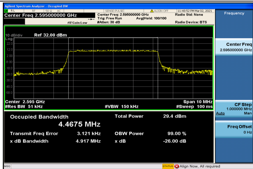
Band38-5MHz-16QAM-38000-25RB#0-4.4675
