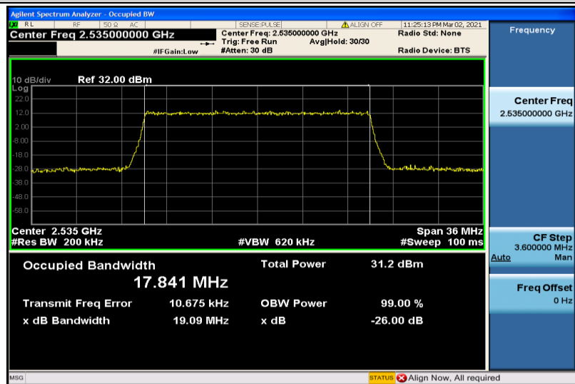
Band7-20MHz-QPSK-21100-100RB#0-17.841
