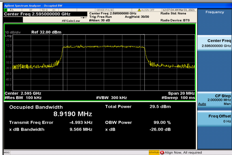
Band38-10MHz-16QAM-38000-50RB#0-8.9190
