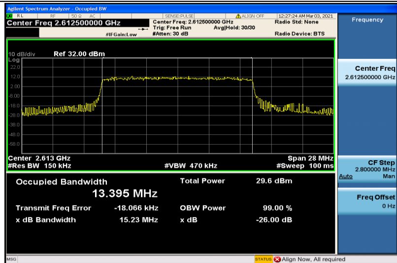
Band38-15MHz-16QAM-38175-75RB#0-13.395
