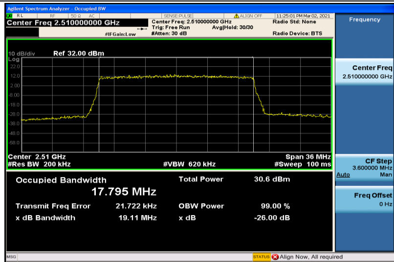
Band7-20MHz-16QAM-20850-100RB#0-17.795
