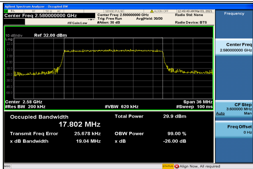
Band38-20MHz-16QAM-37850-100RB#0-17.802
