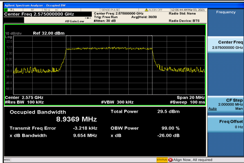
Band38-10MHz-16QAM-37800-50RB#0-8.9369
