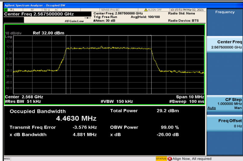
Band7-5MHz-16QAM-21425-25RB#0-4.4630
