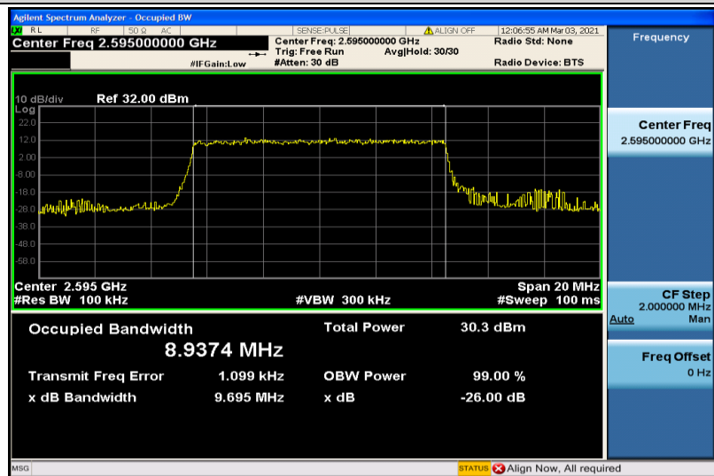
Band38-10MHz-QPSK-38000-50RB#0-8.9374
