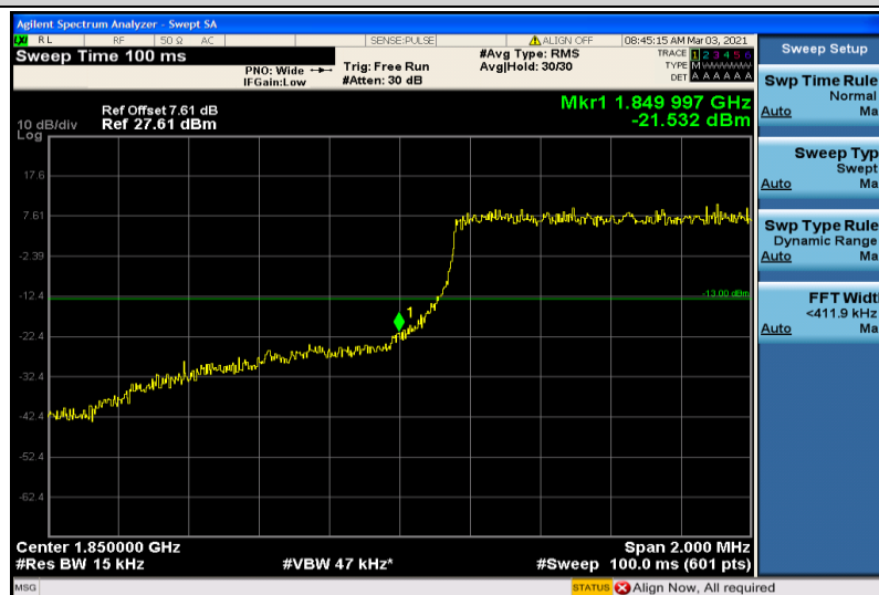
Band2-1.4MHz-QPSK-18607-6RB#0
