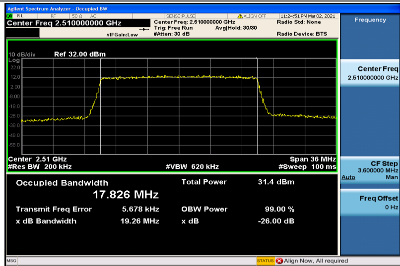
Band7-20MHz-QPSK-20850-100RB#0-17.826
