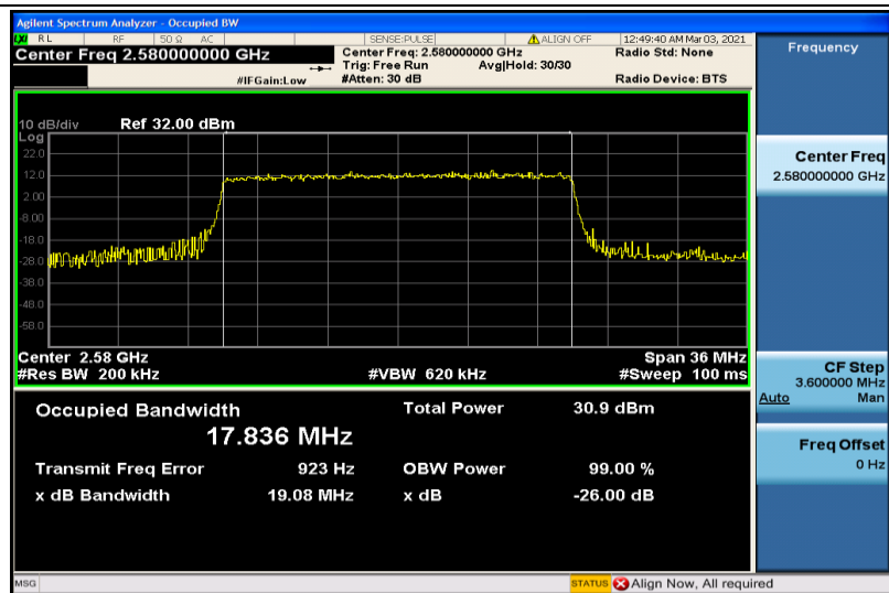
Band38-20MHz-QPSK-37850-100RB#0-17.836
