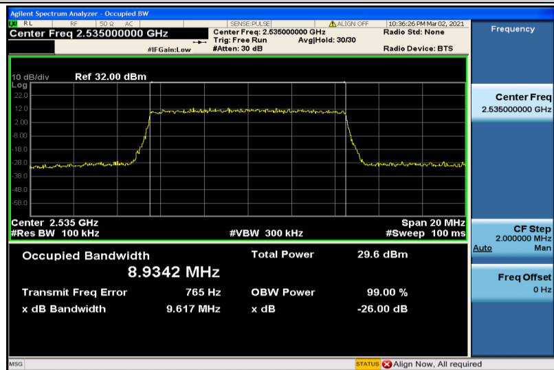
Band7-10MHz-16QAM-21100-50RB#0-8.9342
