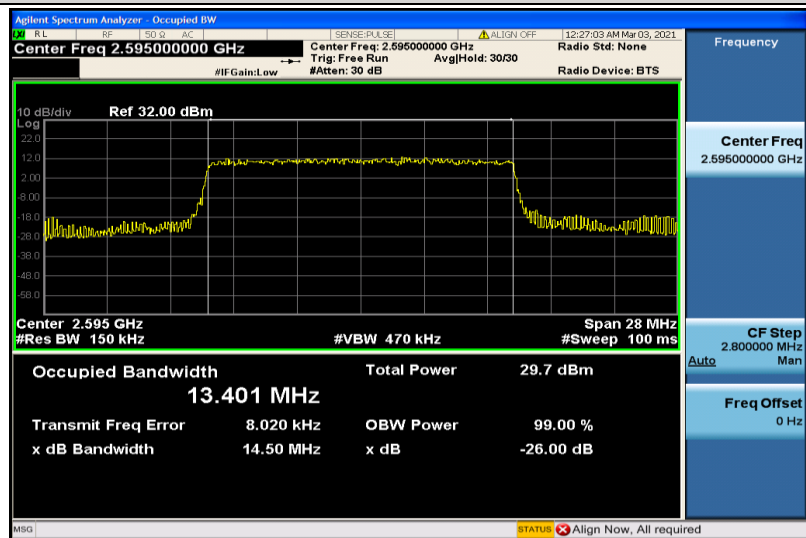
Band38-15MHz-16QAM-38000-75RB#0-13.401
