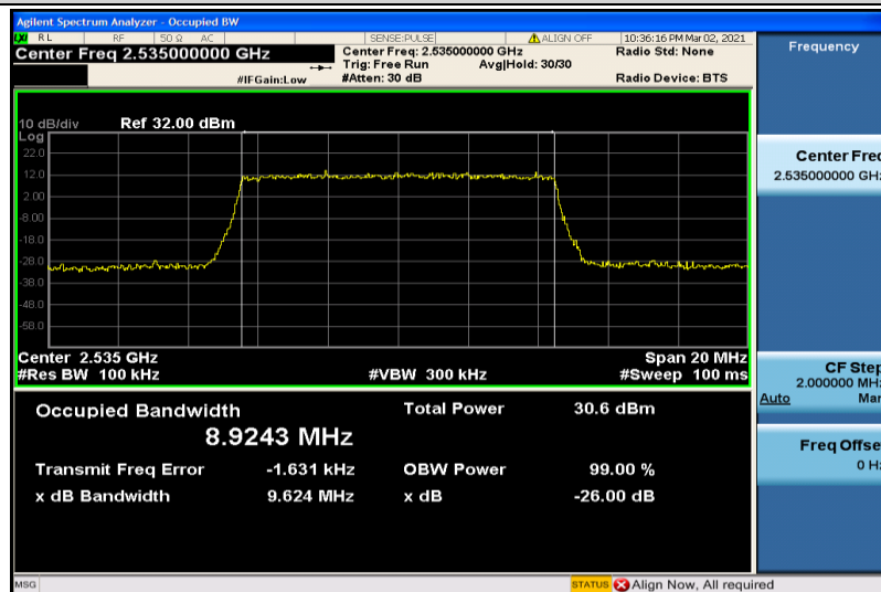
Band7-10MHz-QPSK-21100-50RB#0-8.9243
