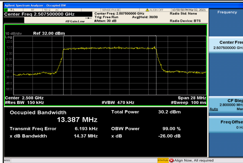
Band7-15MHz-16QAM-20825-75RB#0-13.387
