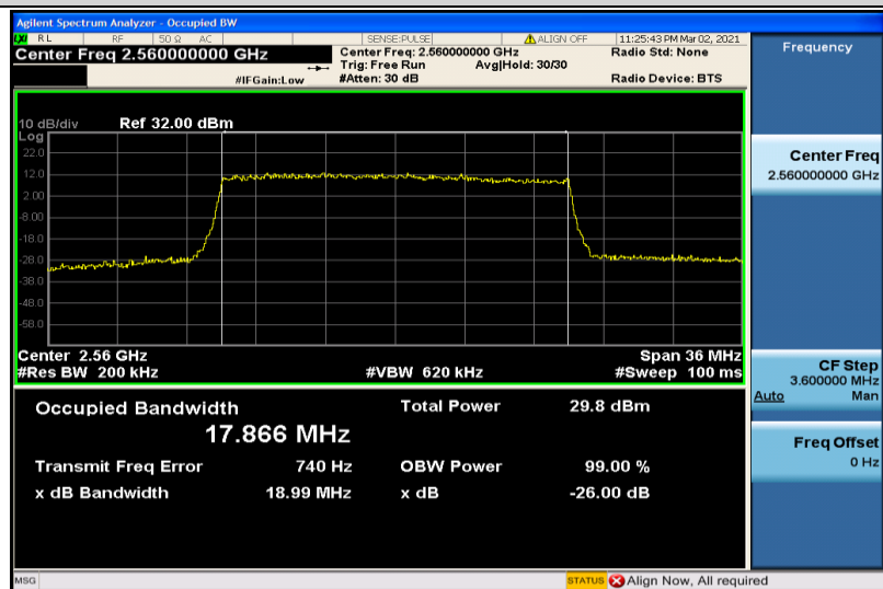
Band7-20MHz-16QAM-21350-100RB#0-17.866
