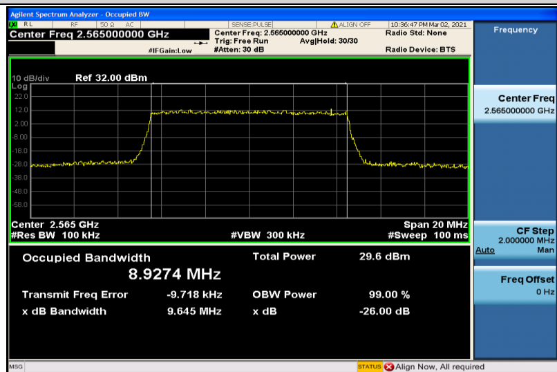
Band7-10MHz-16QAM-21400-50RB#0-8.9274
