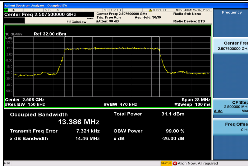
Band7-15MHz-QPSK-20825-75RB#0-13.386
