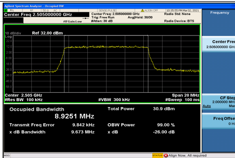
Band7-10MHz-QPSK-20800-50RB#0-8.9251
