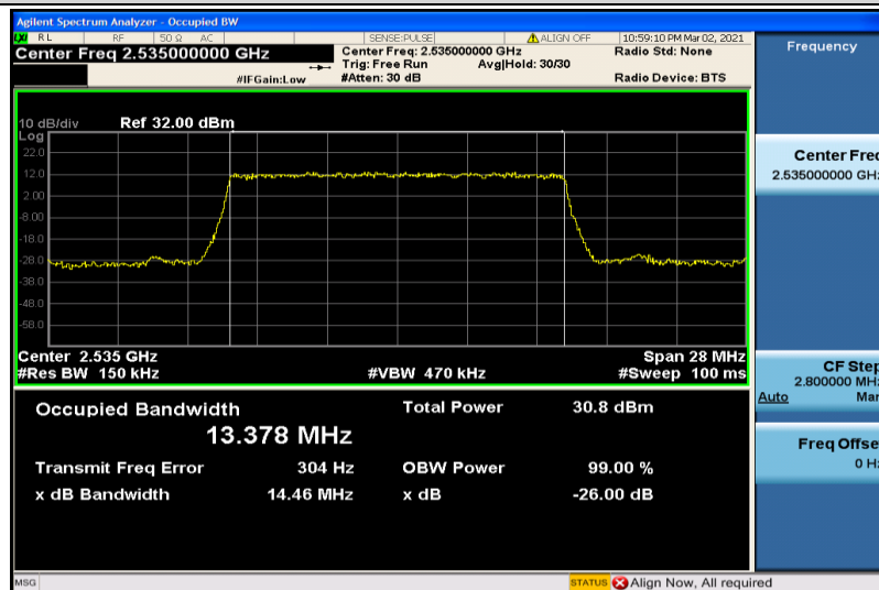
Band7-15MHz-QPSK-21100-75RB#0-13.378
