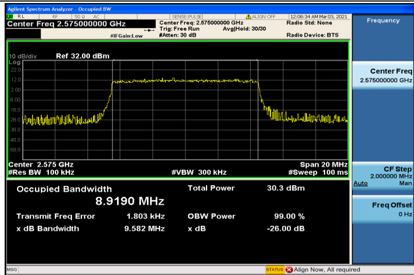
Band38-10MHz-QPSK-37800-50RB#0-8.9190
