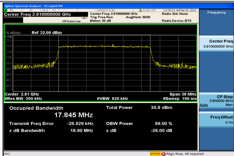
Band38-20MHz-QPSK-38150-100RB#0-17.845
