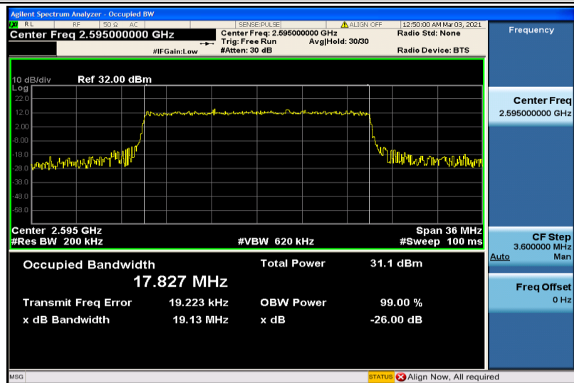
Band38-20MHz-QPSK-38000-100RB#0-17.827
