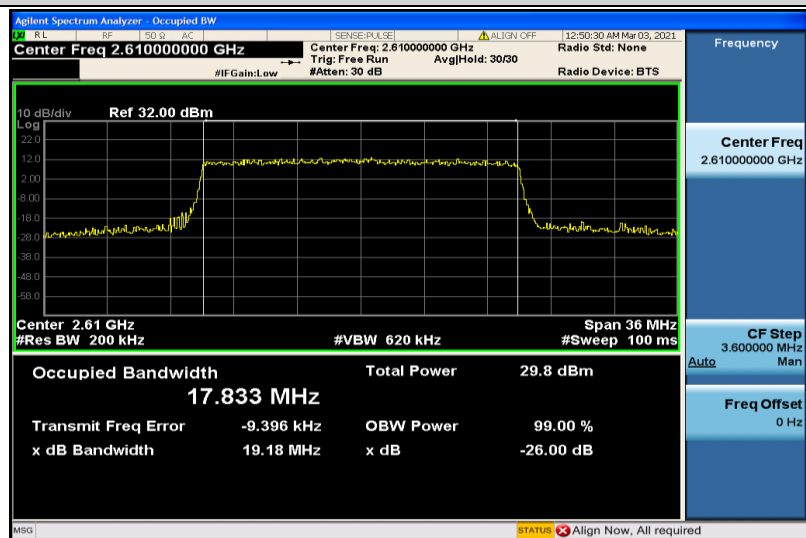
Band38-20MHz-16QAM-38150-100RB#0-17.833
