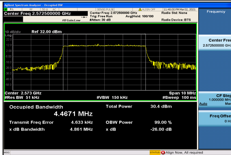
Band38-5MHz-QPSK-37775-25RB#0-4.4671
