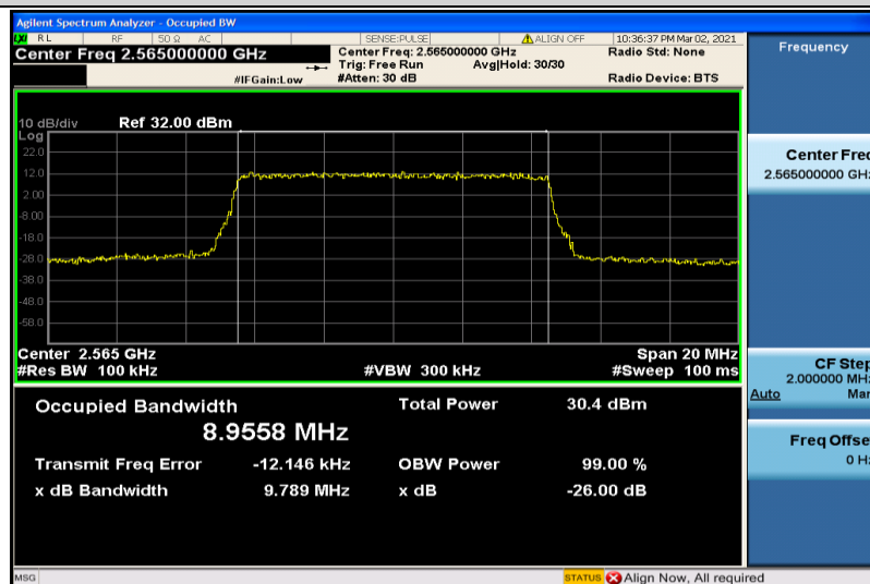
Band7-10MHz-QPSK-21400-50RB#0-8.9558
