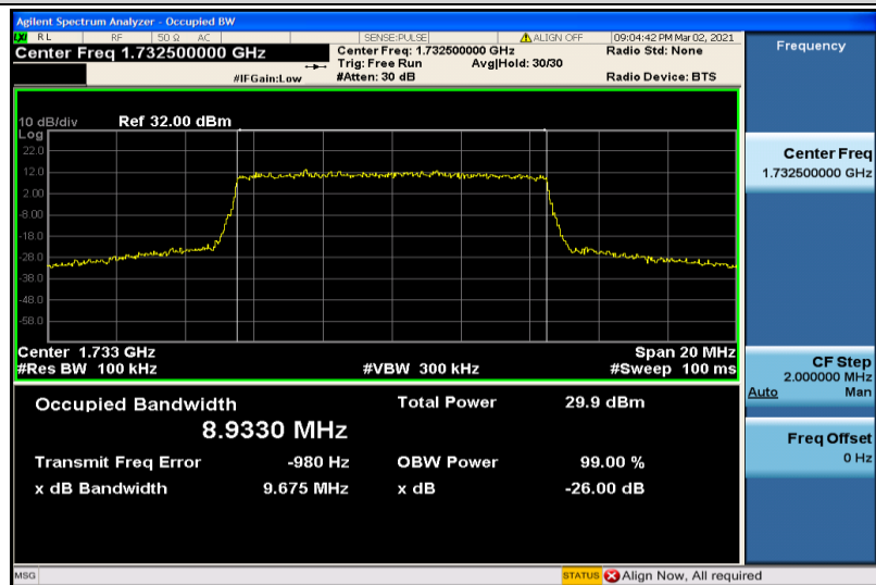
Band4-10MHz-16QAM-20175-50RB#0-8.9330
