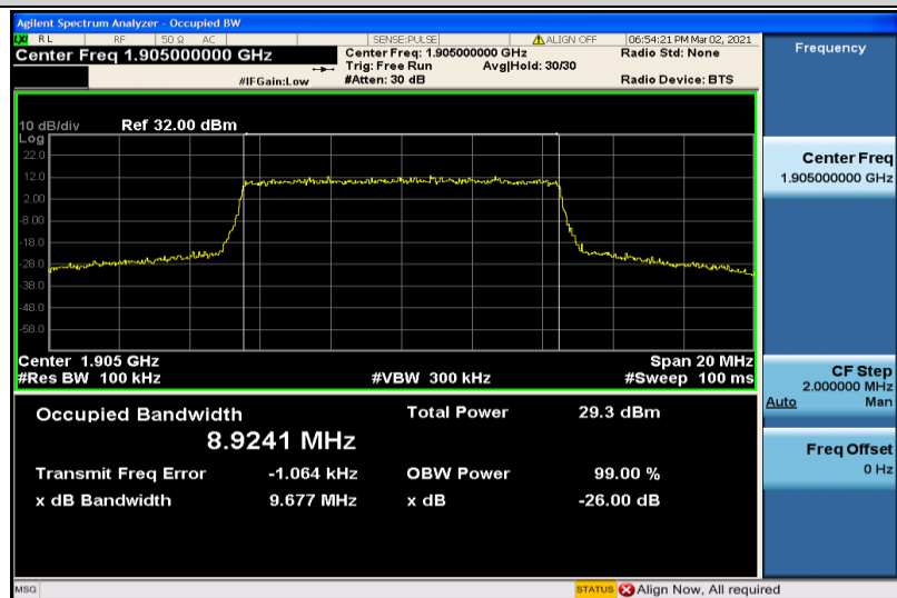
Band2-10MHz-QPSK-19150-50RB#0-8.9241
