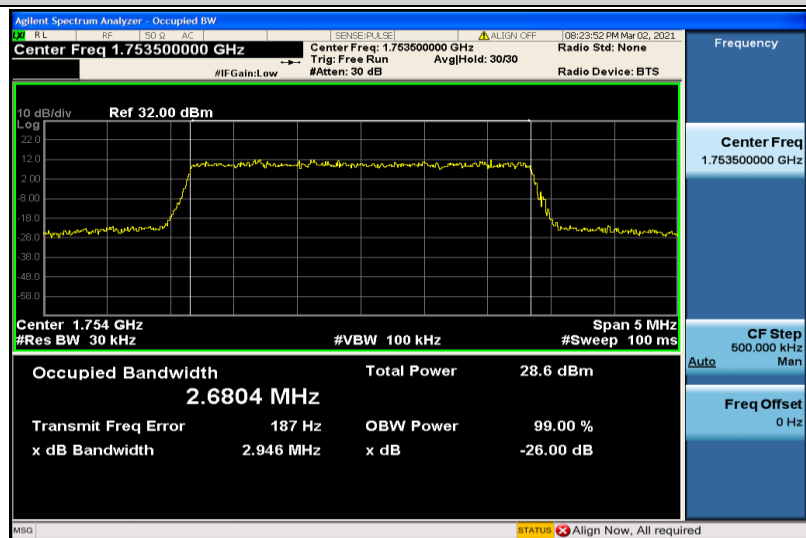
Band4-3MHz-16QAM-20385-15RB#0-2.6804
