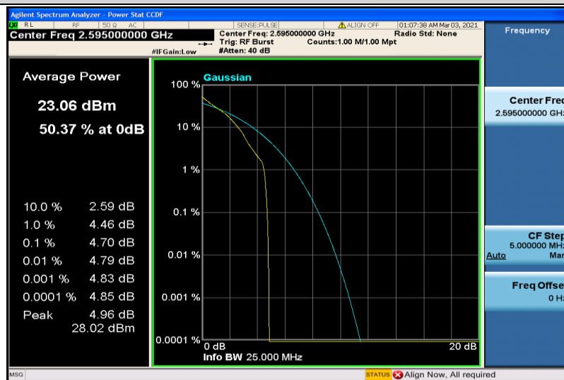
Band38-20MHz-QPSK-38000-1RB#0
