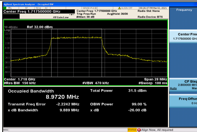
Band4-15MHz-QPSK-20025-75RB#0-8.9720
