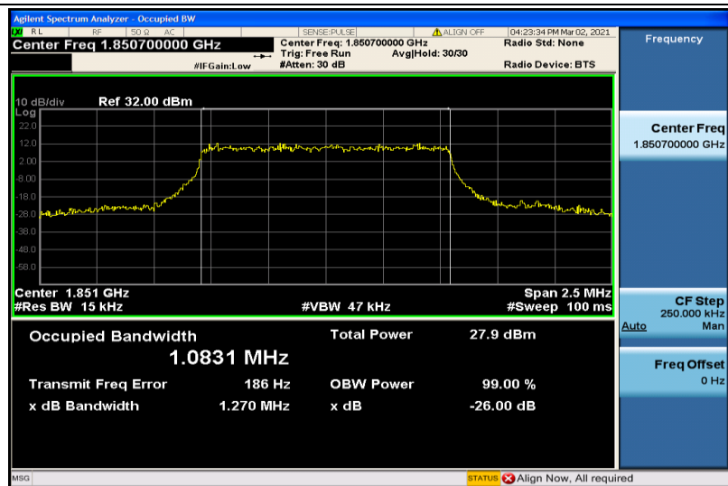
Band2-1.4MHz-16QAM-18607-6RB#0-1.0831
