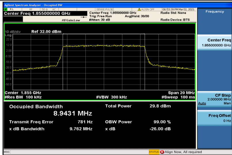
Band2-10MHz-QPSK-18650-50RB#0-8.9431
