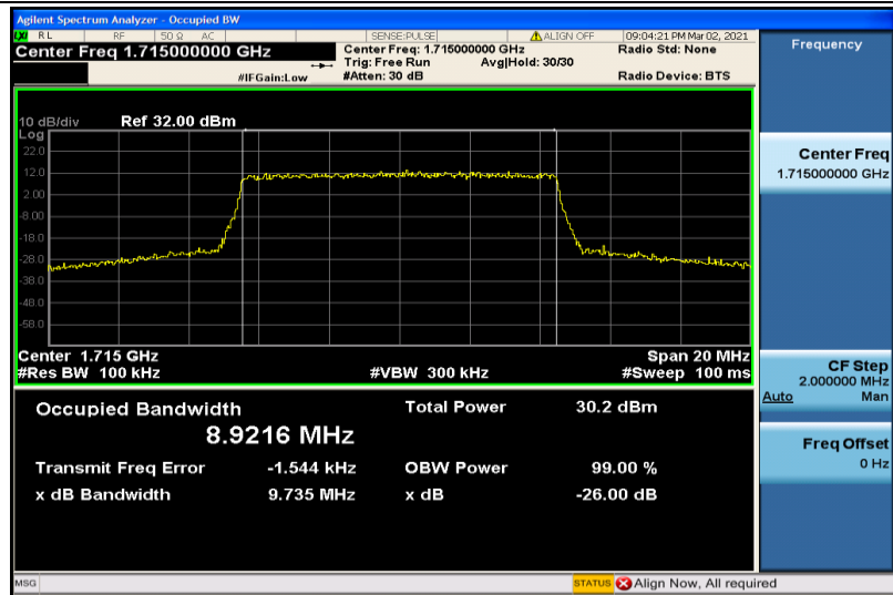
Band4-10MHz-16QAM-20000-50RB#0-8.9216
