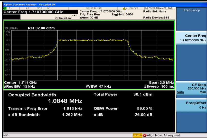
Band4-1.4MHz-QPSK-19957-6RB#0-1.0848
