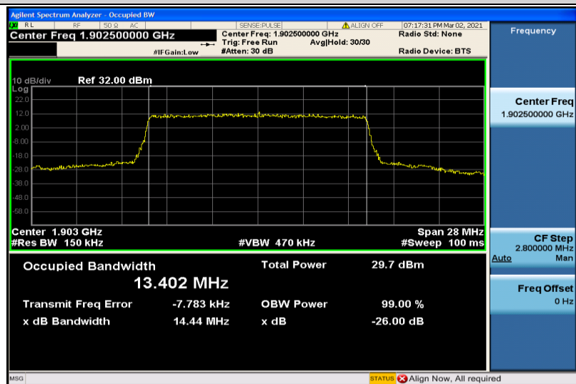
Band2-15MHz-QPSK-19125-75RB#0-13.402
