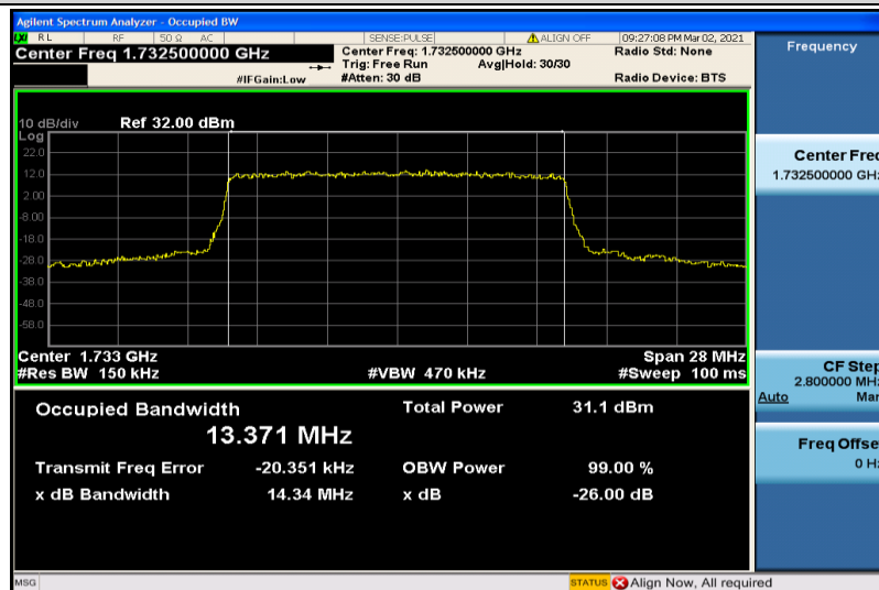
Band4-15MHz-QPSK-20175-75RB#0-13.371
