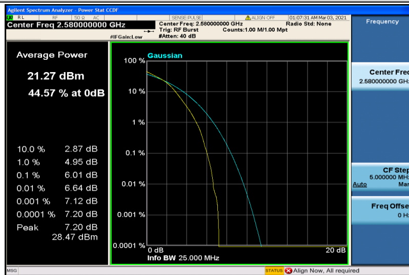
Band38-20MHz-16QAM-37850-100RB#0
