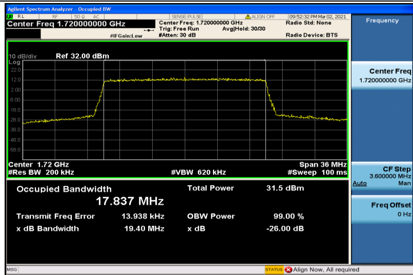
Band4-20MHz-QPSK-20050-100RB#0-17.837
