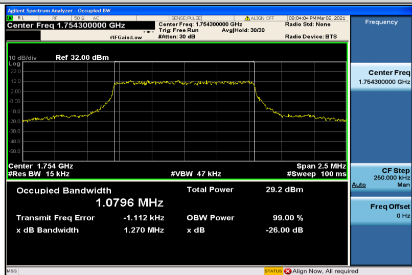
Band4-1.4MHz-QPSK-20393-6RB#0-1.0796
