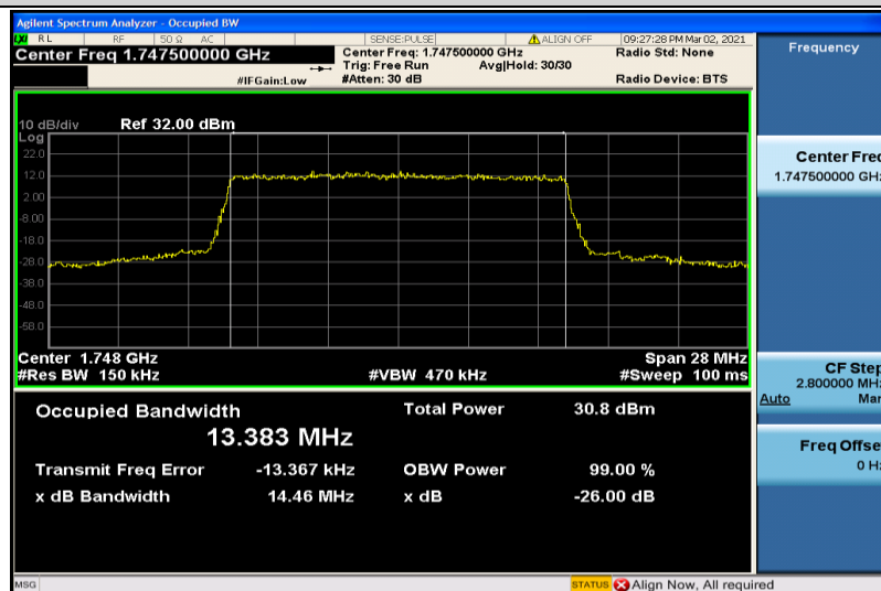
Band4-15MHz-QPSK-20325-75RB#0-13.383
