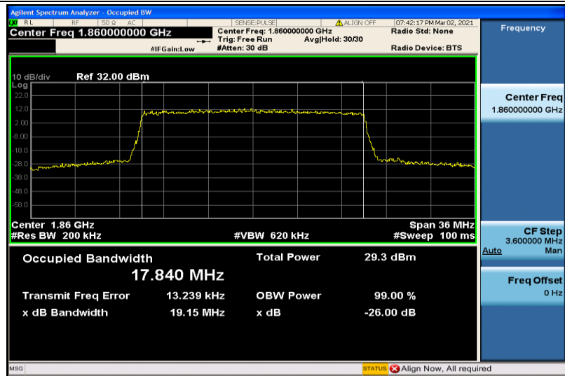
Band2-20MHz-16QAM-18700-100RB#0-17.840
