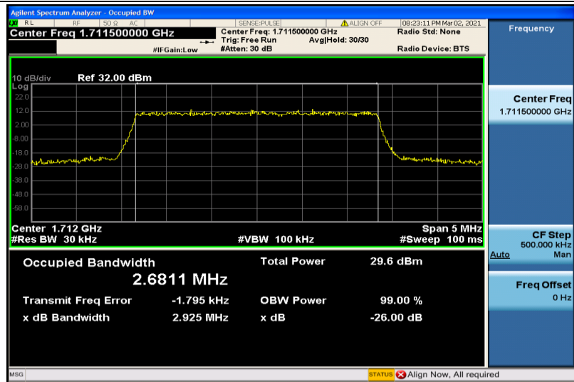
Band4-3MHz-16QAM-19965-15RB#0-2.6811
