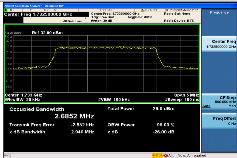
Band4-3MHz-16QAM-20175-15RB#0-2.6852
