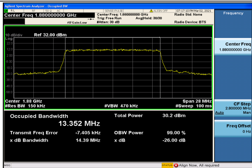
Band2-15MHz-QPSK-18900-75RB#0-13.352
