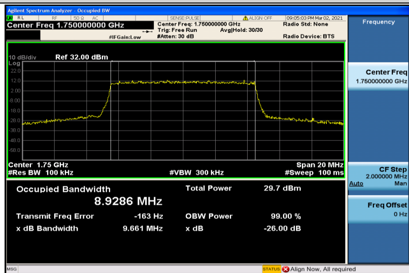
Band4-10MHz-16QAM-20350-50RB#0-8.9286
