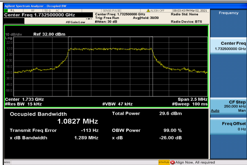
Band4-1.4MHz-QPSK-20175-6RB#0-1.0827
