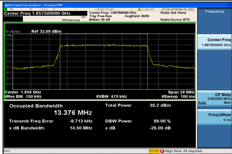
Band2-15MHz-QPSK-18675-75RB#0-13.376
