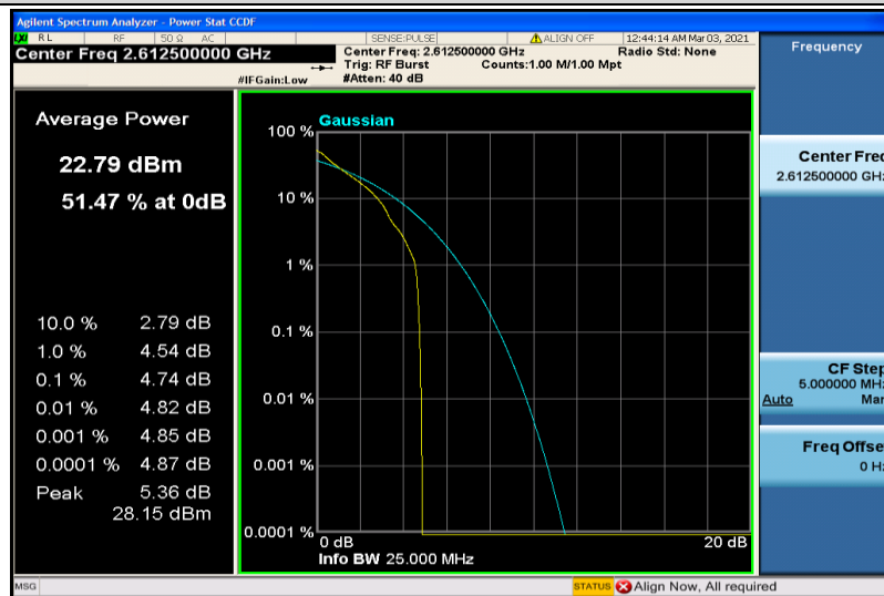
Band38-15MHz-QPSK-38175-1RB#0
