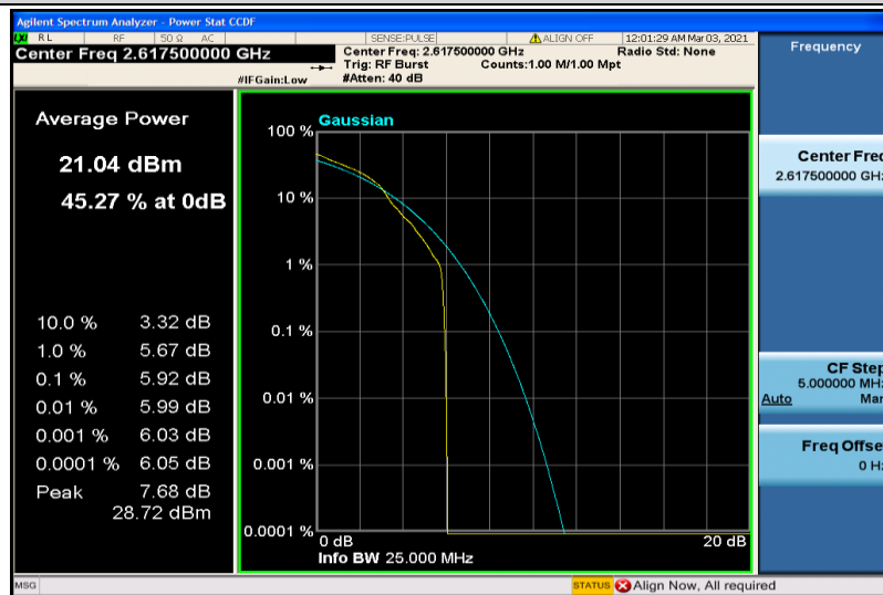
Band38-5MHz-16QAM-38225-1RB#0
