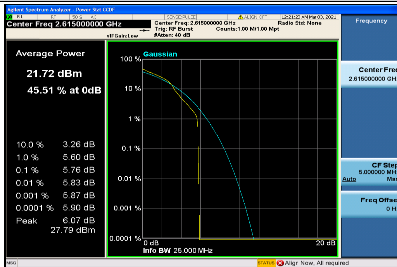
Band38-10MHz-16QAM-38200-1RB#0
