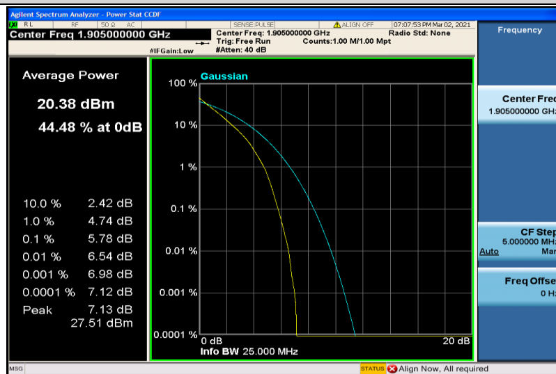
Band2-10MHz-QPSK-19150-50RB#0
