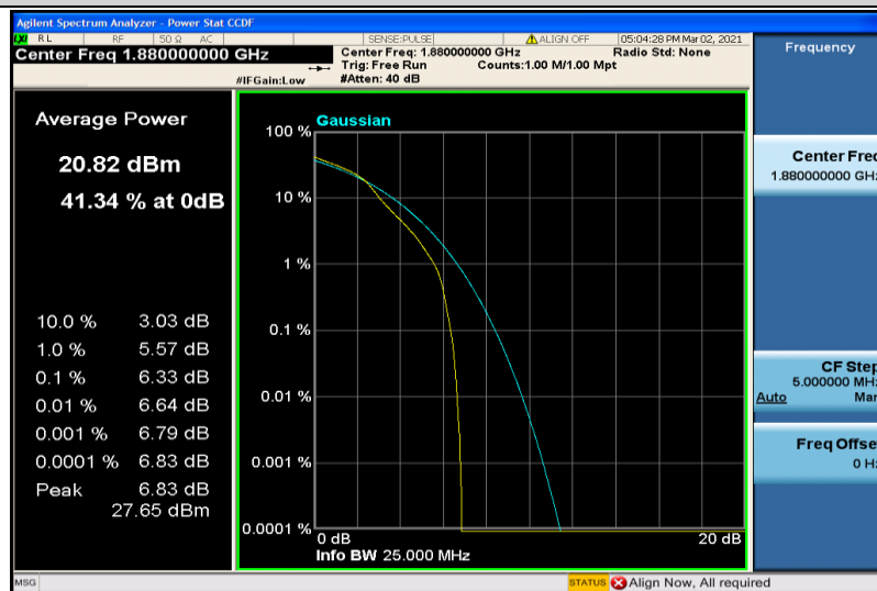
Band2-3MHz-16QAM-18900-1RB#0
