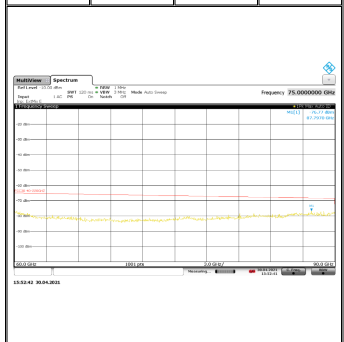
Plot# 39 Radiated Emission 60-90GHz
