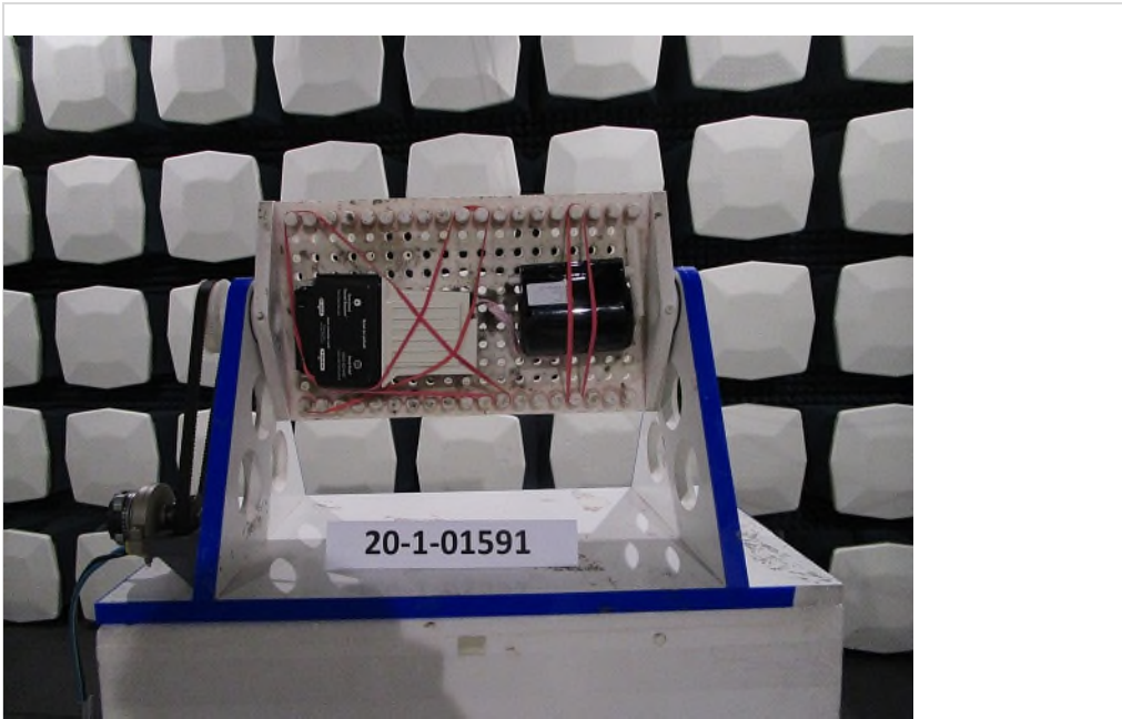
Photograph 3: EUT test setup in the fully anechoic chamber, close up view
