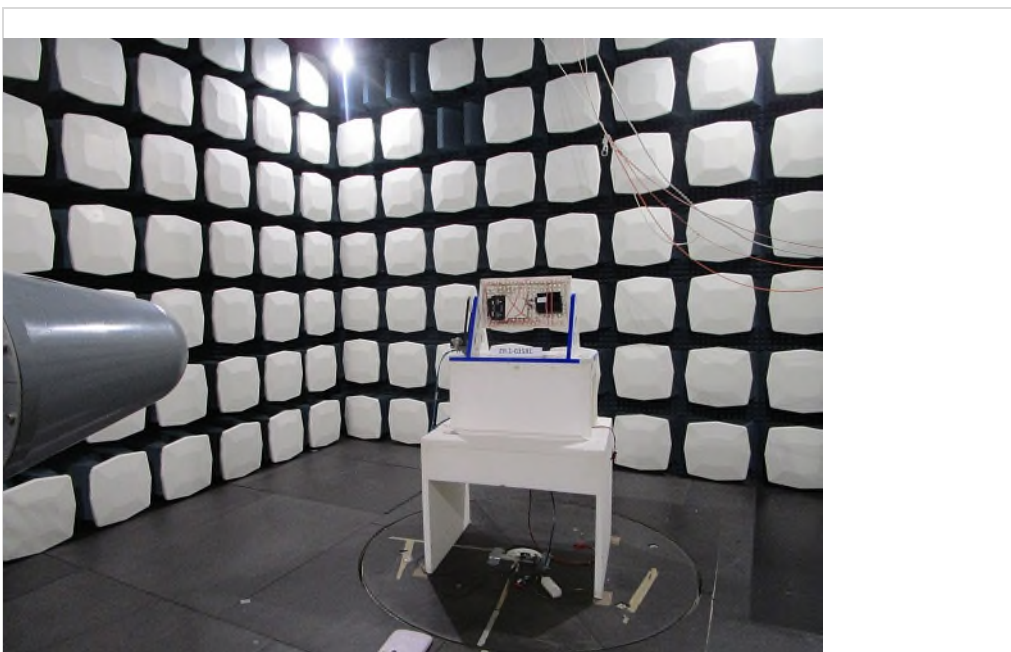
Photograph 4: EUT test setup in the fully anechoic chamber, overview
