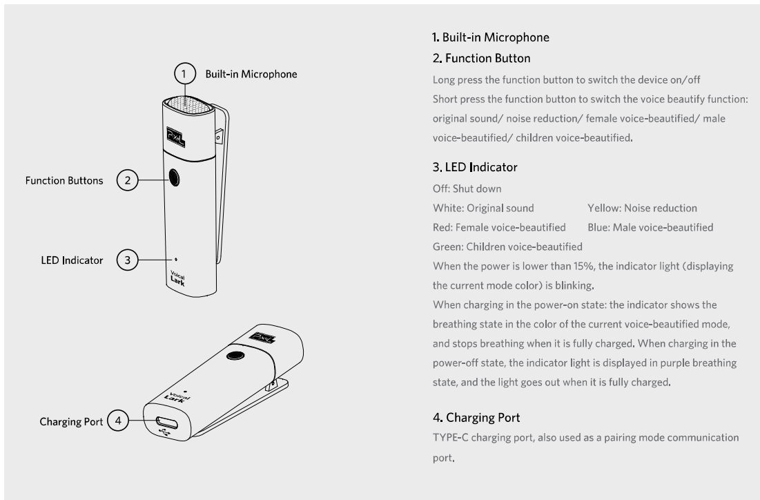
Transmitter
