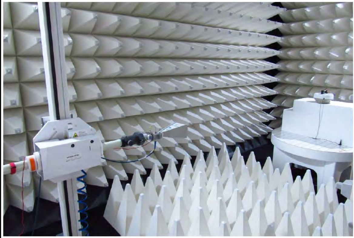
Setup 8 - 18 GHz B
