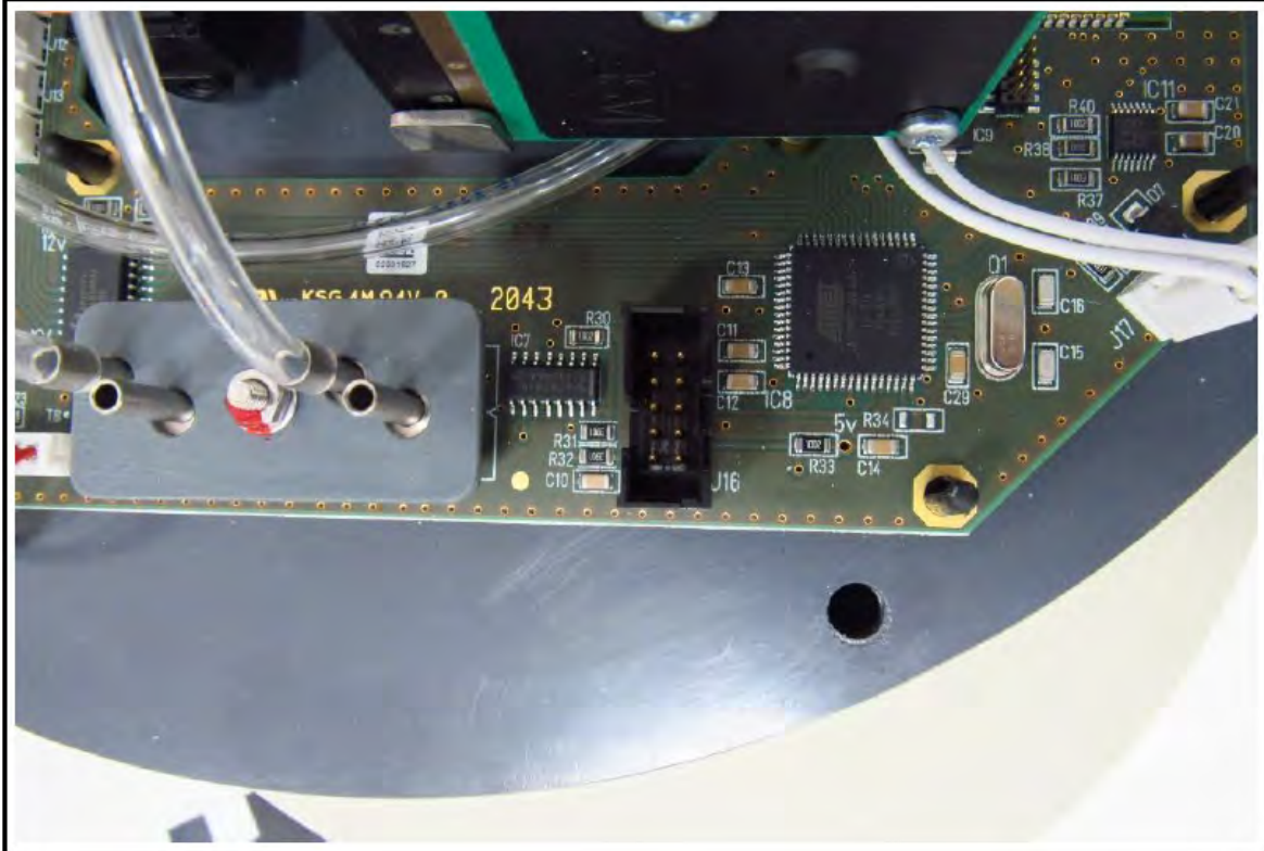
PCB top view B
