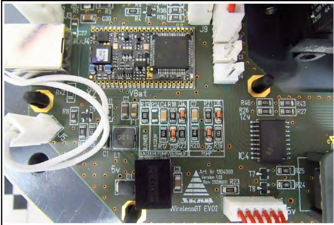
PCB top view C
