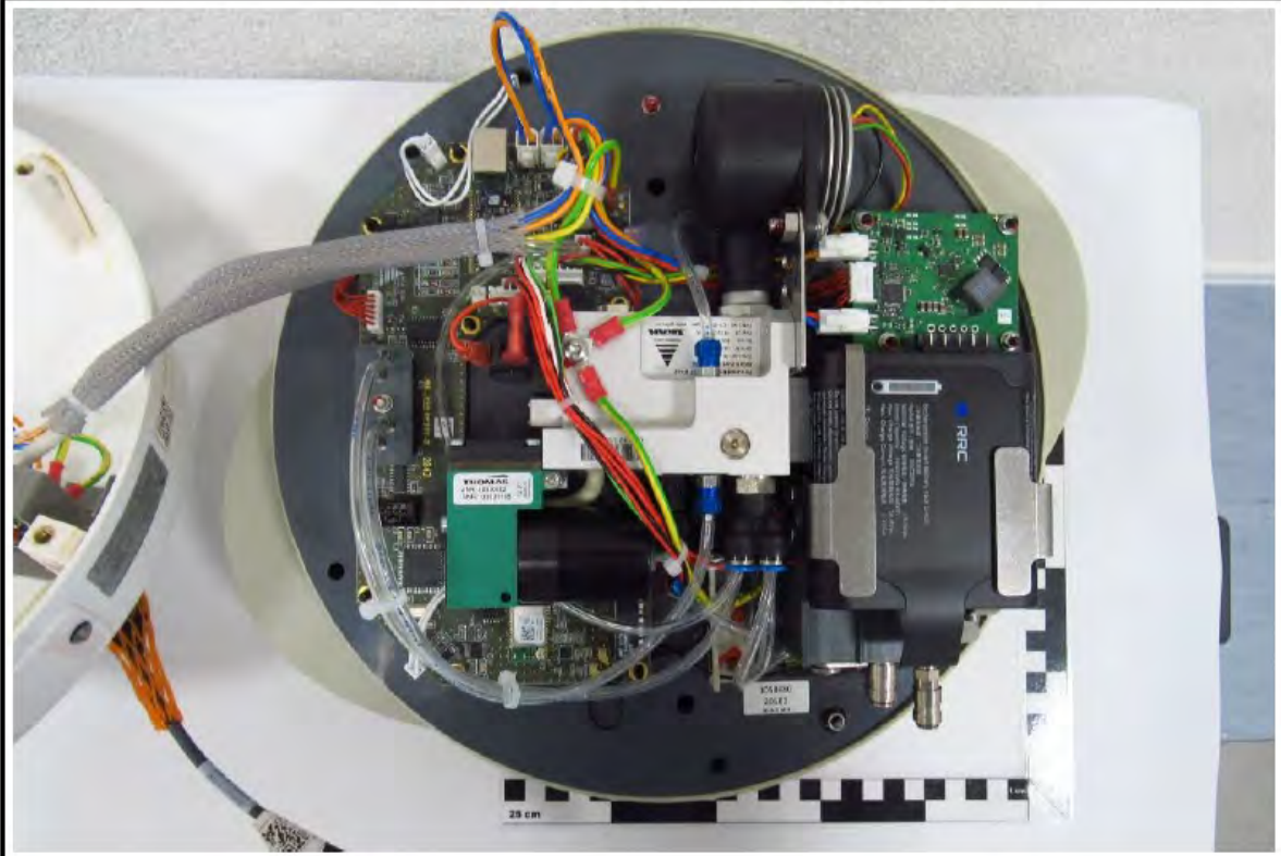
Interior view A
