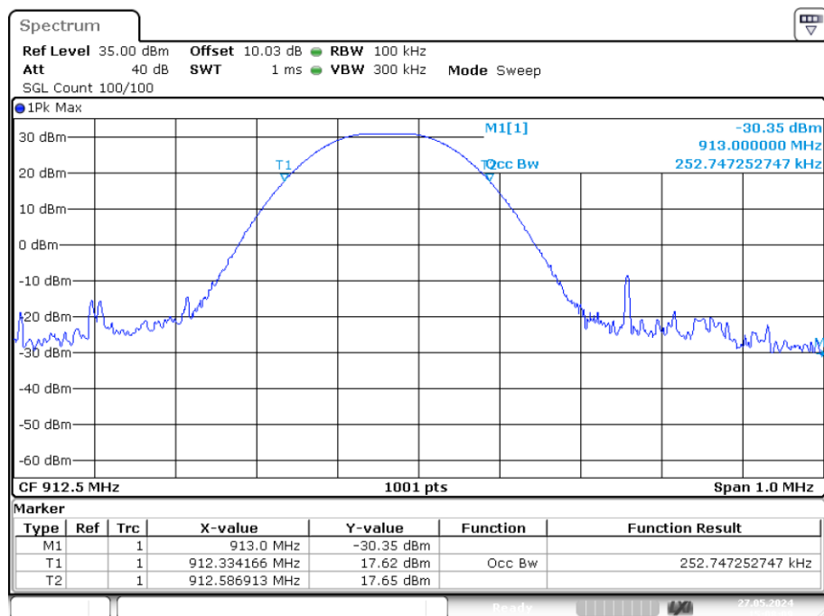
OBW NVNT user 912.5MHz Ant1
