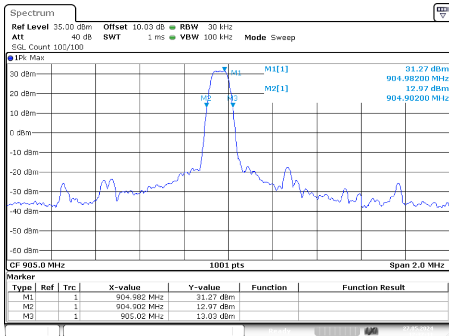
-20dB Bandwidth NVNT user 905MHz Ant1
