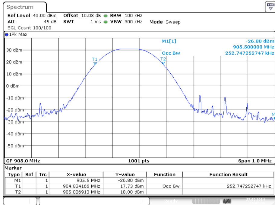
OBW NVNT user 905MHz Ant1
