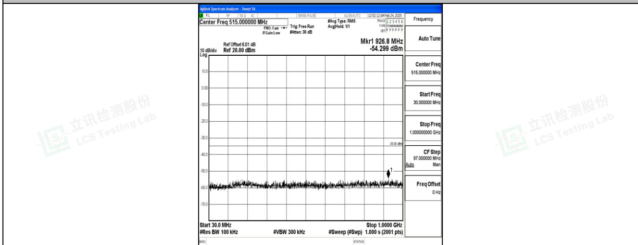
Band7_20MHz_QPSK_20850_1RB#0_30~1000_30~1000
