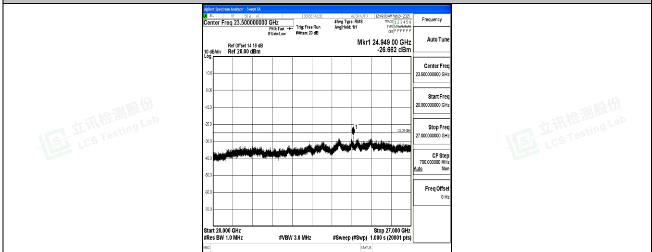
Band7_15MHz_16QAM_21375_1RB#0_20000~27000_20000~27000
