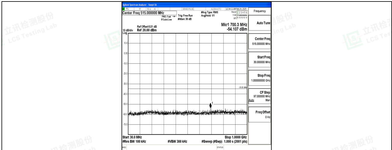
Band7_5MHz_QPSK_21100_1RB#0_30~1000_30~1000
