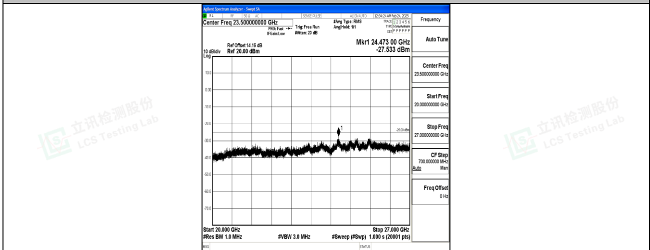
Band7_5MHz_QPSK_21100_1RB#0_20000~27000_20000~27000
