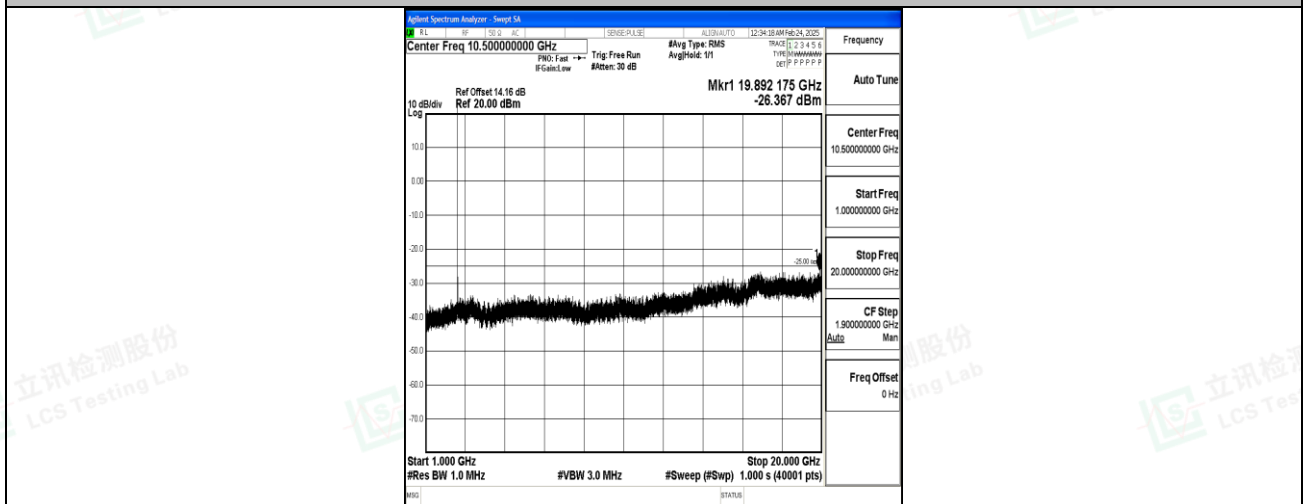
Band7_5MHz_QPSK_21100_1RB#0_1000~20000_1000~20000
