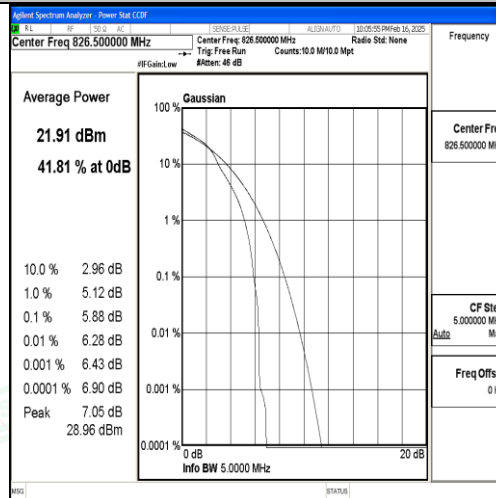
Band5-5MHz-16QAM-20425-1RB#0-PASS
