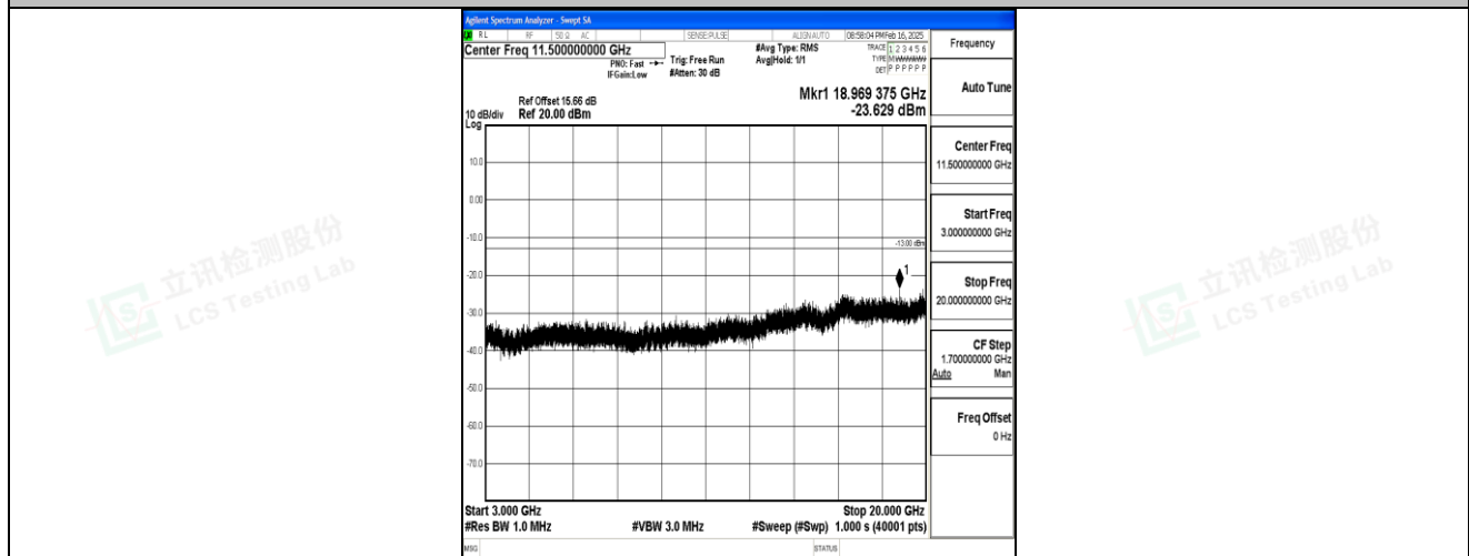
Band4_20MHz_16QAM_20050_1RB#0_3000~20000_3000~20000
