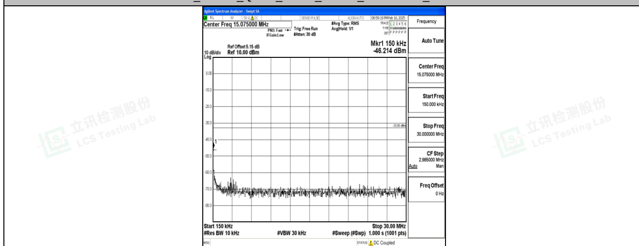
Band4_20MHz_QPSK_20300_1RB#0_0.15~30_0.15~30
