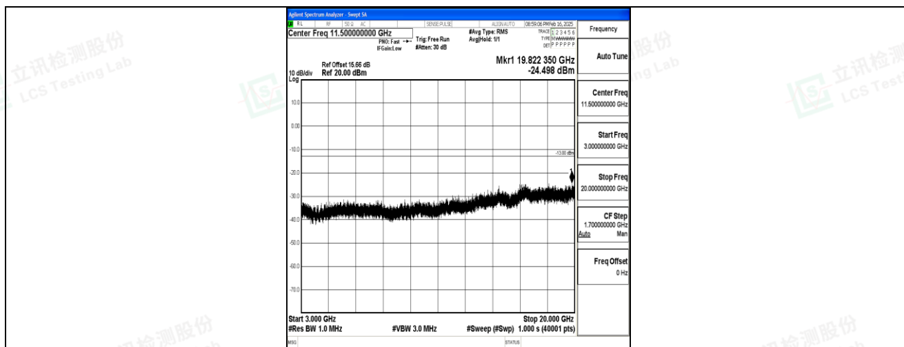
Band4_20MHz_16QAM_20175_1RB#0_3000~20000_3000~20000
