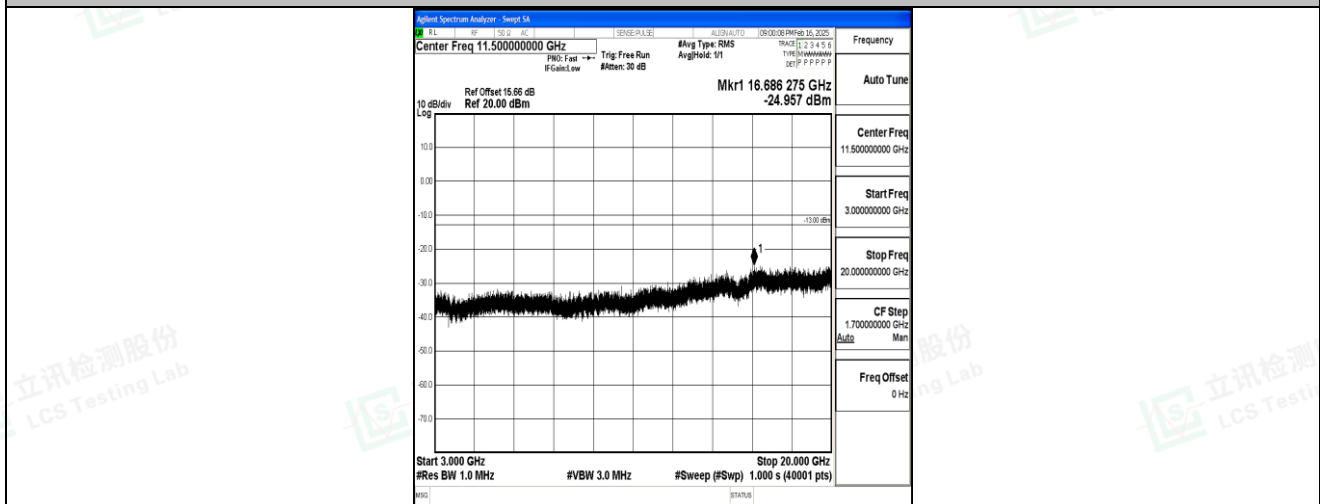
Band4_20MHz_16QAM_20300_1RB#0_3000~20000_3000~20000
