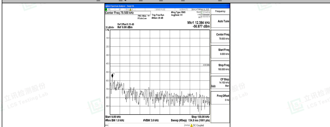
Band4_15MHz_16QAM_20025_1RB#0_0.009~0.15_0.009~0.15
