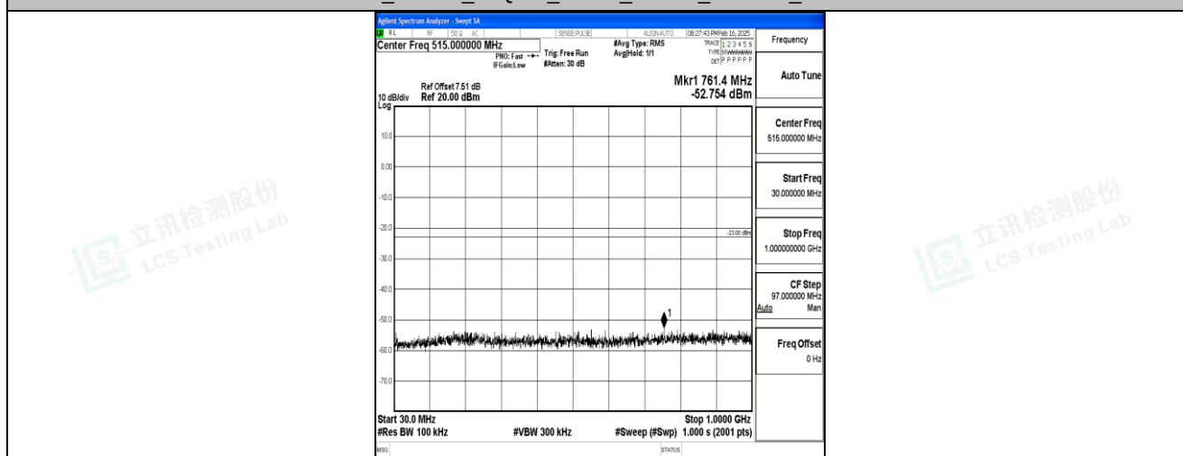
Band4_10MHz_16QAM_20350_1RB#0_30~1000_30~1000
