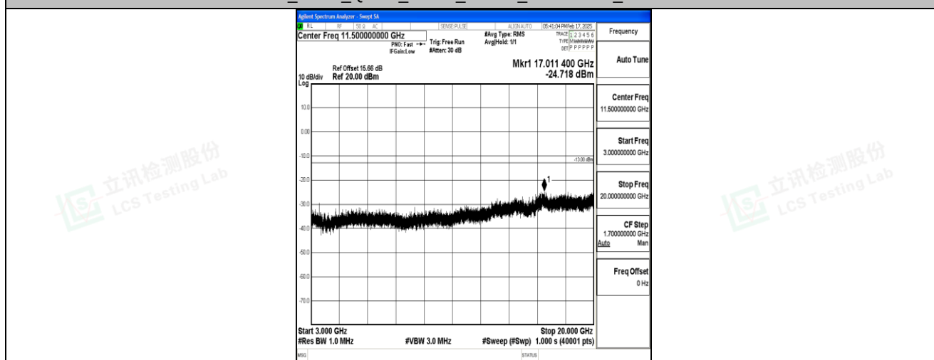
Band4_3MHz_QPSK_20385_1RB#0_3000~20000_3000~20000
