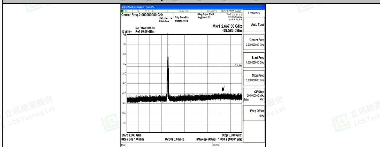
Band4_10MHz_16QAM_20000_1RB#0_1000~3000_1000~3000
