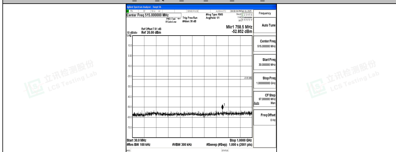
Band4_5MHz_QPSK_20175_1RB#0_30-1000_30-1000
