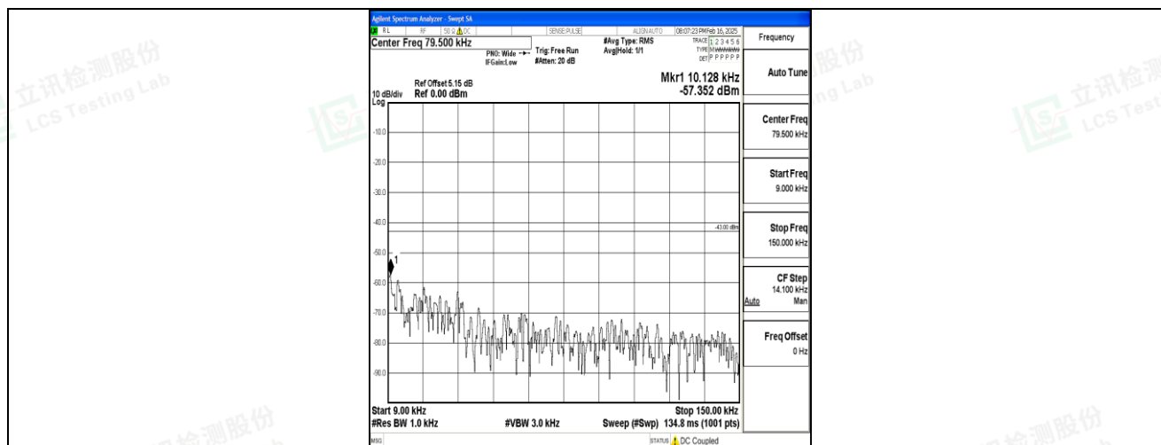
Band4_5MHz_QPSK_19975_1RB#0_0.009-0.15_0.009-0.15
