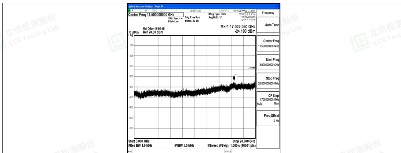
Band4_3MHz_16QAM_20175_1RB#0_3000~20000_3000~20000
