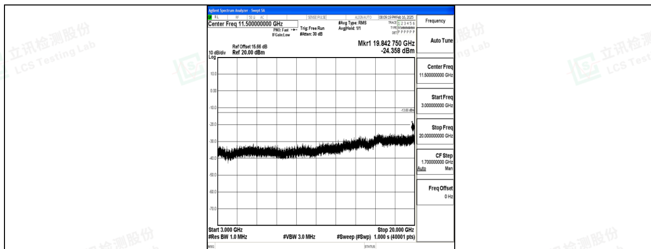
Band4_5MHz_16QAM_20175_1RB#0_3000~20000_3000~20000
