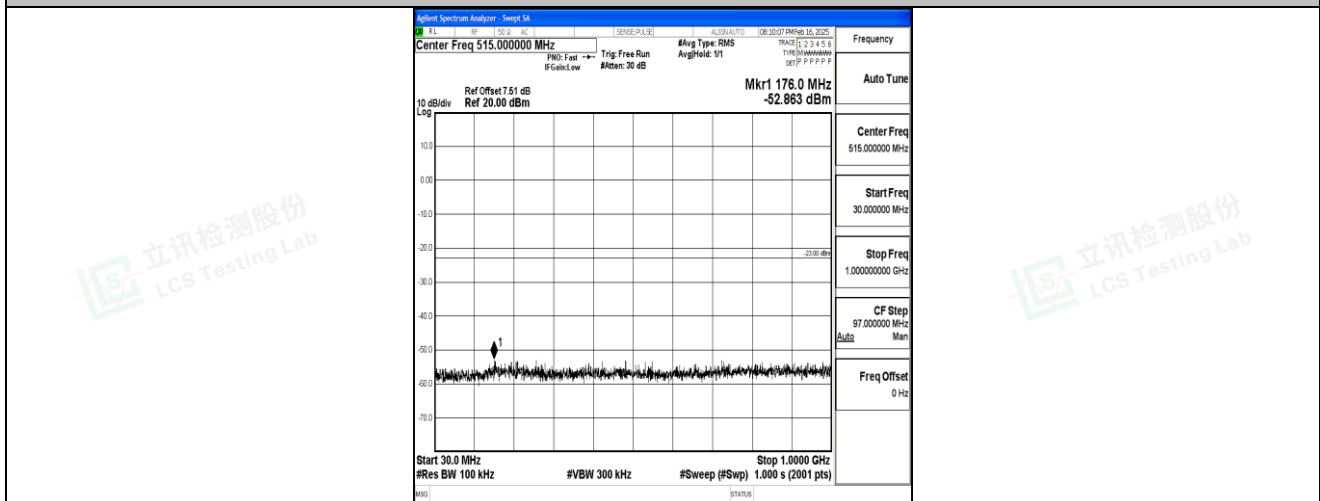
Band4_5MHz_16QAM_20375_1RB#0_30~1000_30~1000
