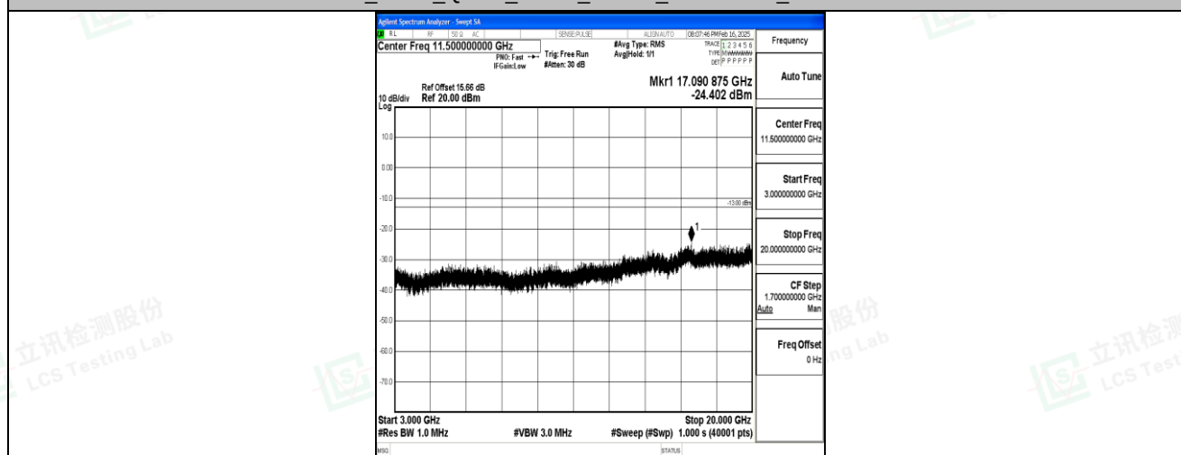
Band4_5MHz_QPSK_19975_1RB#0_3000~20000_3000~20000
