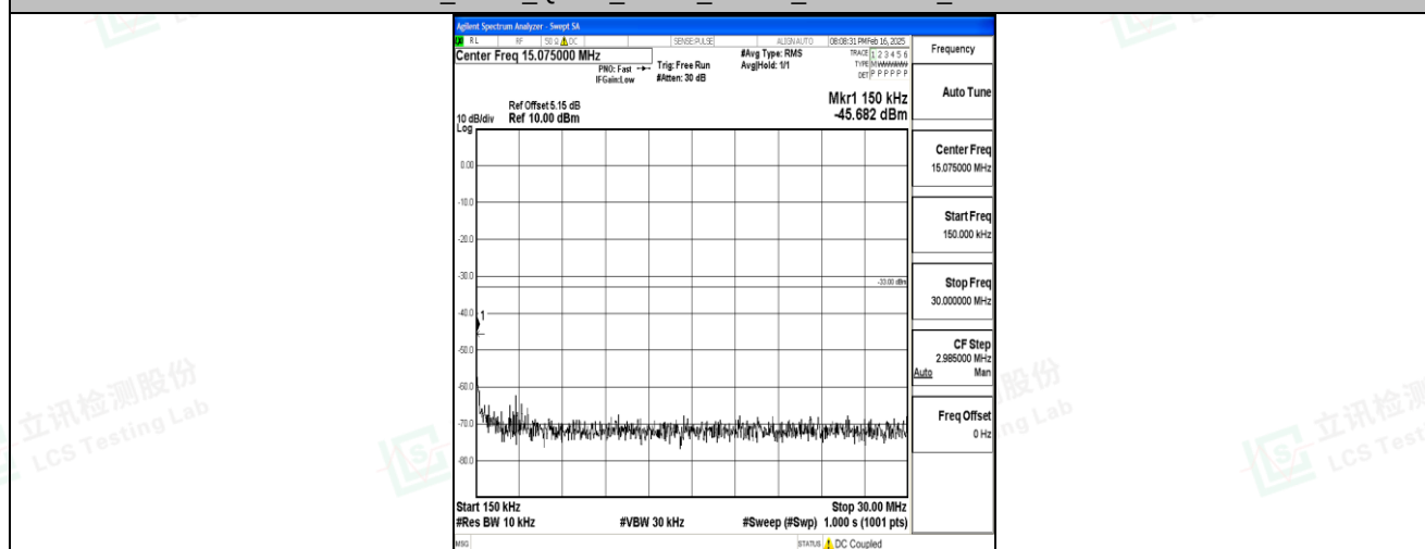
Band4_5MHz_QPSK_20175_1RB#0_0.15-30_0.15-30
