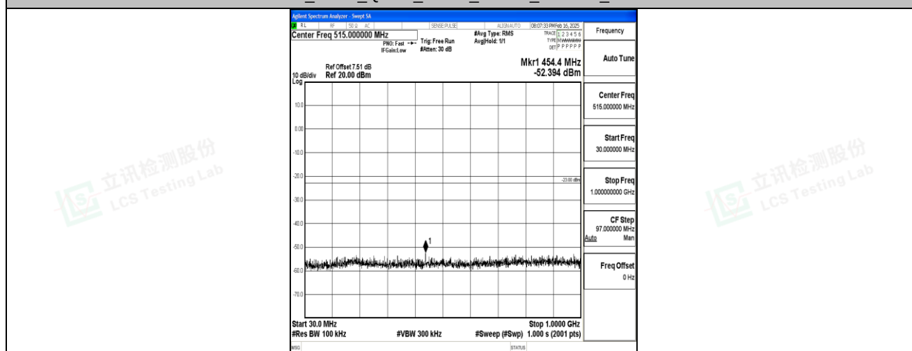
Band4_5MHz_QPSK_19975_1RB#0_30-1000_30-1000
