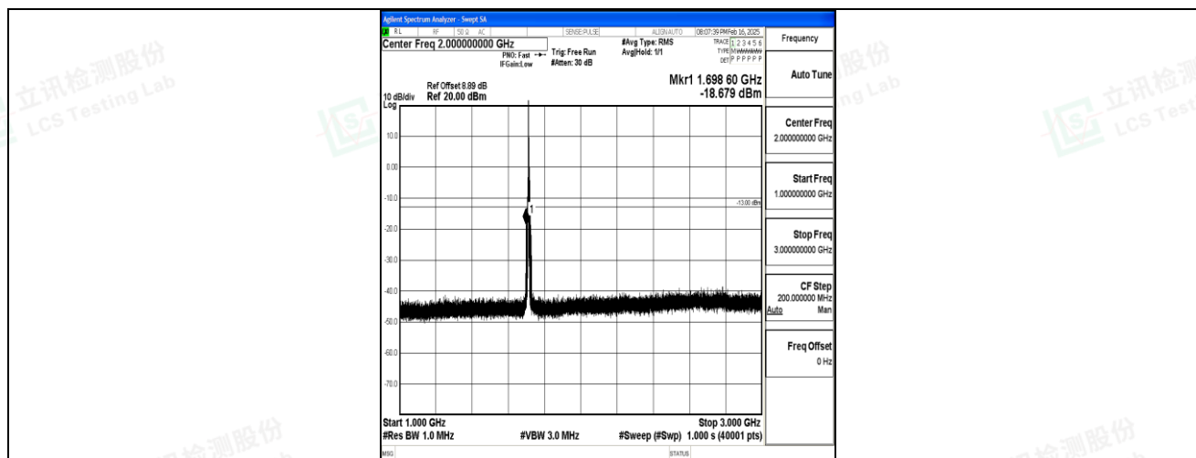
Band4_5MHz_QPSK_19975_1RB#0_1000~3000_1000~3000
