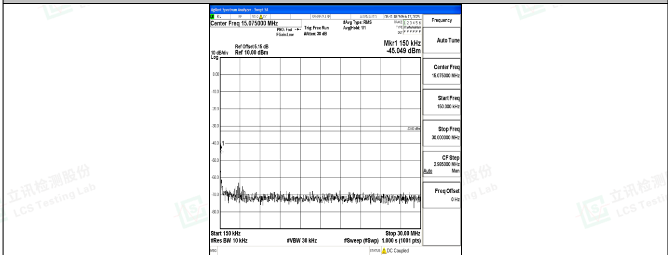
Band4_3MHz_16QAM_20385_1RB#0_0.15~30_0.15~30
