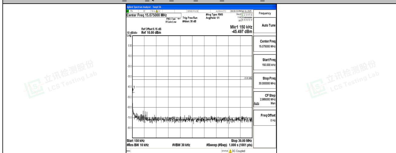
Band4_5MHz_QPSK_20375_1RB#0_0.15~30_0.15~30
