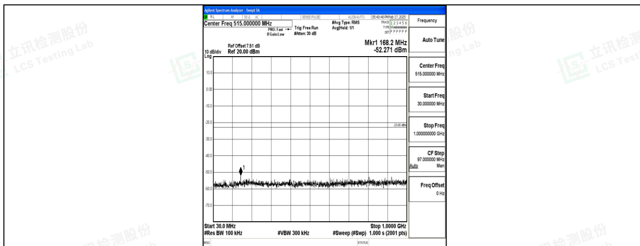
Band4_3MHz_QPSK_20385_1RB#0_30~1000_30~1000
