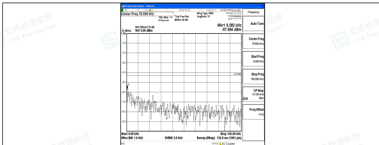
Band4_5MHz_QPSK_20175_1RB#0_0.009-0.15_0.009-0.15
