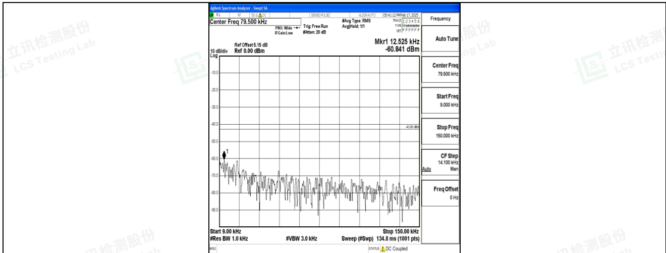
Band4_3MHz_16QAM_20385_1RB#0_0.009~0.15_0.009~0.15
