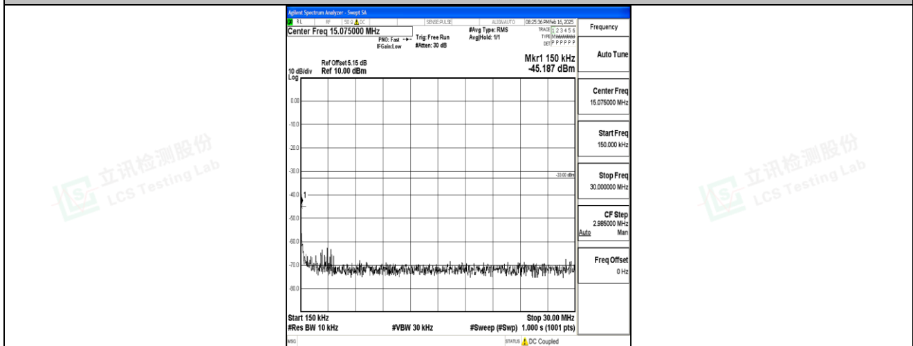
Band4_10MHz_16QAM_20000_1RB#0_0.15~30_0.15~30
