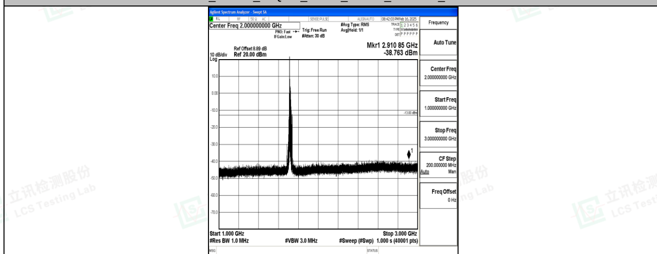
Band4_15MHz_16QAM_20025_1RB#0_1000~3000_1000~3000
