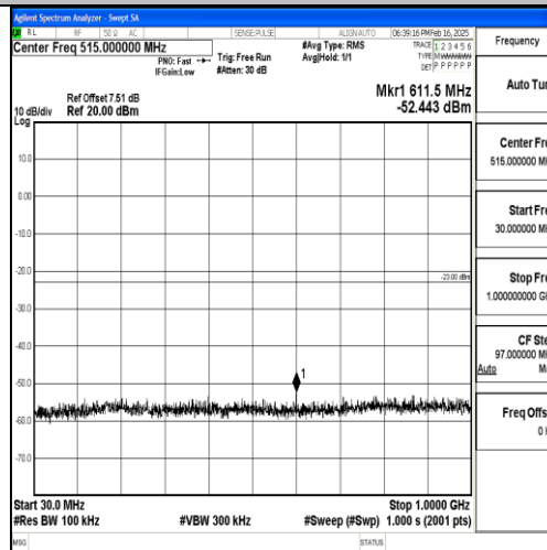
Band2_10MHz_16QAM_19150_1RB#0_30~1000_30~1000
