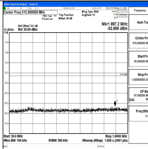
Band2_3MHz_QPSK_19185_1RB#0_30~1000_30~1000
