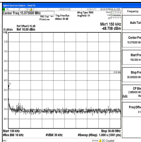
Band2_5MHz_16QAM_18900_1RB#0_0.15~30_0.15~30
