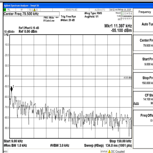
Band2_15MHz_QPSK_18675_1RB#0_0.009~0.15_0.009~0.15
