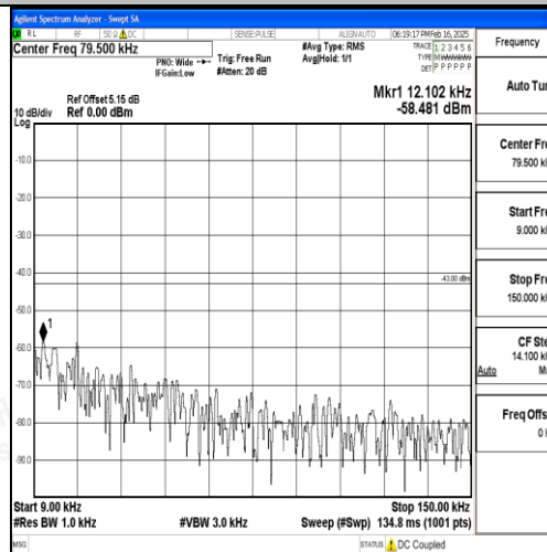
Band2_5MHz_16QAM_18625_1RB#0_0.009~0.15_0.009~0.15
