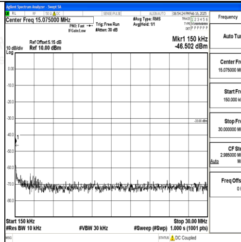
Band2_15MHz_16QAM_18900_1RB#0_0.15~30_0.15~30
