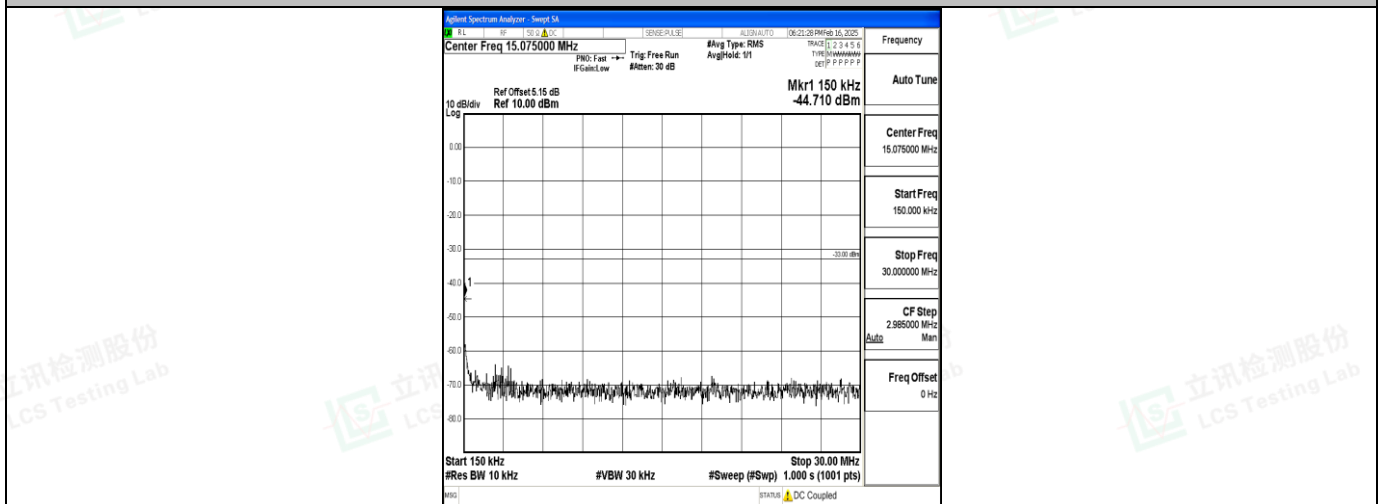
Band2_5MHz_16QAM_19175_1RB#0_0.15~30_0.15~30
