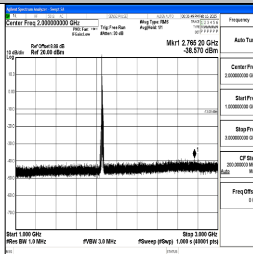
Band2_10MHz_QPSK_18650_1RB#0_1000~3000_1000~3000
