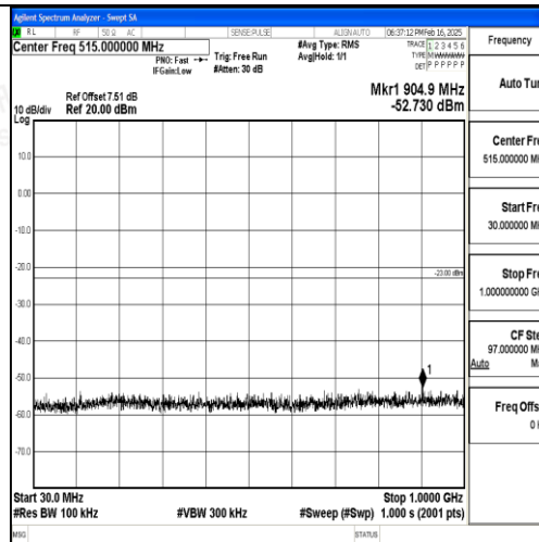
Band2_10MHz_16QAM_18650_1RB#0_30~1000_30~1000
