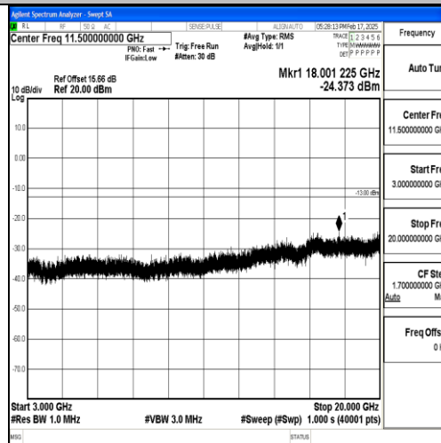
Band2_3MHz_QPSK_19185_1RB#0_3000~20000_3000~20000
