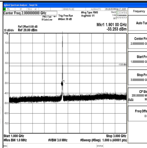
Band2_3MHz_QPSK_19185_1RB#0_1000~3000_1000~3000
