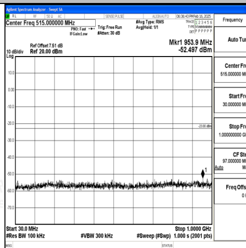
Band2_10MHz_QPSK_18650_1RB#0_30~1000_30~1000
