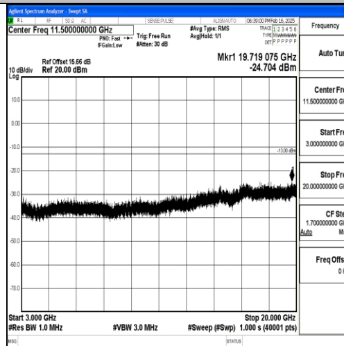
Band2_10MHz_QPSK_19150_1RB#0_3000~20000_3000~20000
