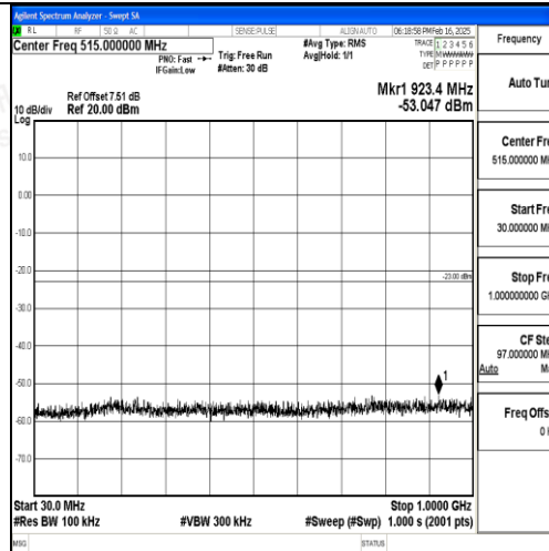
Band2_5MHz_QPSK_18625_1RB#0_30~1000_30~1000
