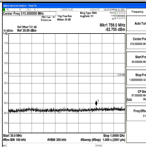
Band2_5MHz_16QAM_18900_1RB#0_30~1000_30~1000
