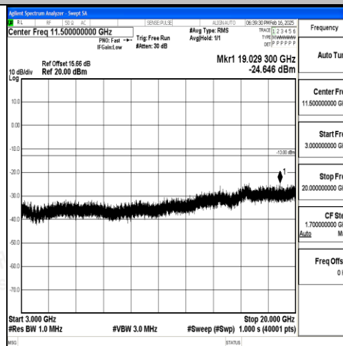
Band2_10MHz_16QAM_19150_1RB#0_3000~20000_3000~20000
