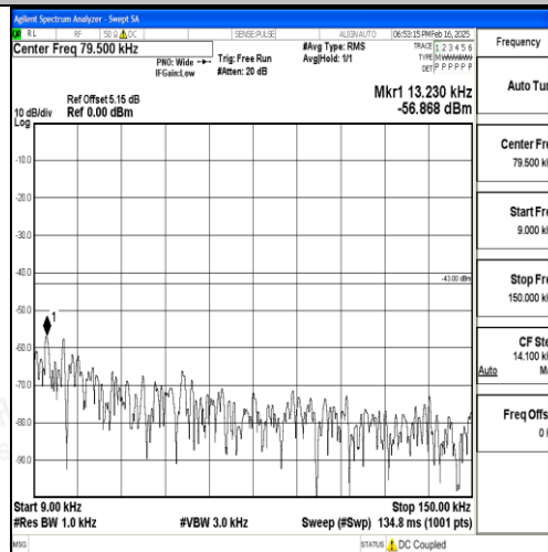
Band2_15MHz_16QAM_18675_1RB#0_0.009~0.15_0.009~0.15
