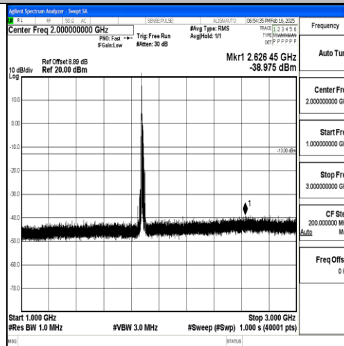
Band2_15MHz_16QAM_18900_1RB#0_1000~3000_1000~3000
