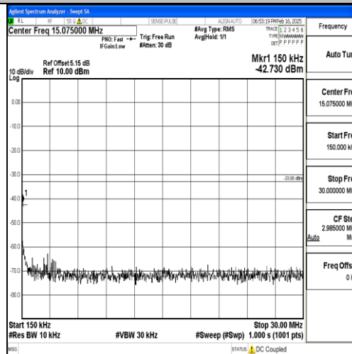
Band2_15MHz_16QAM_18675_1RB#0_0.15~30_0.15~30
