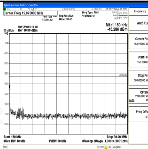
Band2_3MHz_16QAM_19185_1RB#0_0.15~30_0.15~30
