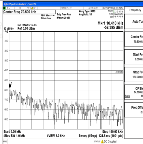
Band2_10MHz_16QAM_19150_1RB#0_0.009~0.15_0.009~0.15
