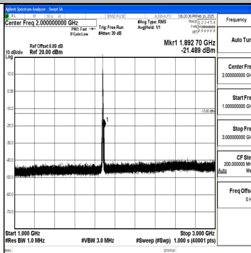
Band2_5MHz_16QAM_18900_1RB#0_1000~3000_1000~3000
