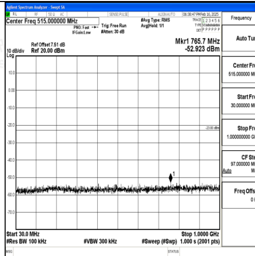
Band2_10MHz_QPSK_19150_1RB#0_30~1000_30~1000
