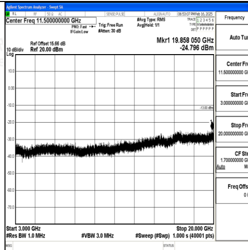
Band2_15MHz_QPSK_18675_1RB#0_3000~20000_3000~20000
