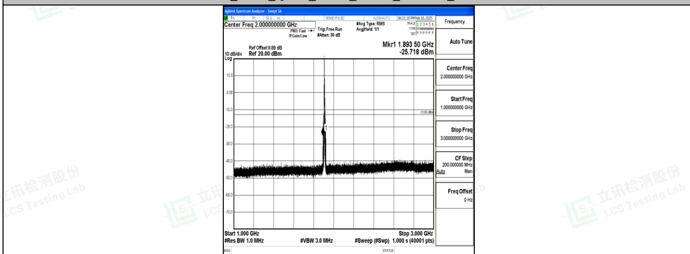
Band2_5MHz_QPSK_19175_1RB#0_1000~3000_1000~3000
