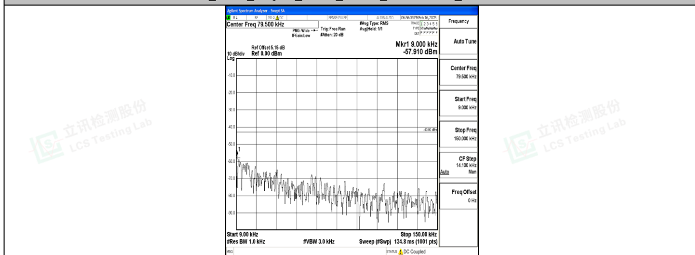
Band2_10MHz_QPSK_18650_1RB#0_0.009~0.15_0.009~0.15
