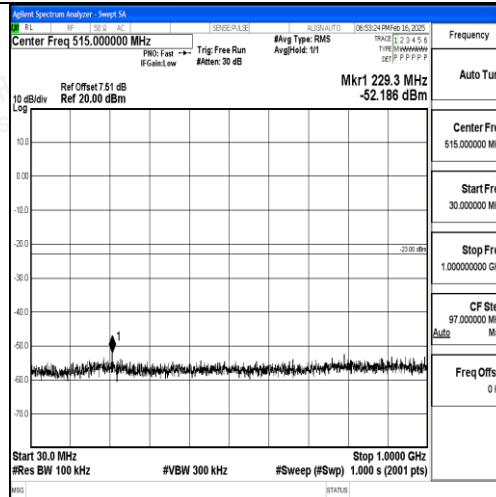
Band2_15MHz_16QAM_18675_1RB#0_30~1000_30~1000
