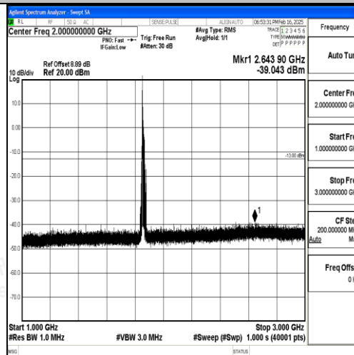
Band2_15MHz_16QAM_18675_1RB#0_1000~3000_1000~3000
