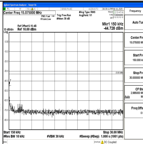
Band2_10MHz_16QAM_19150_1RB#0_0.15~30_0.15~30
