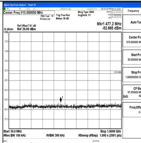
Band2_15MHz_16QAM_18900_1RB#0_30~1000_30~1000
