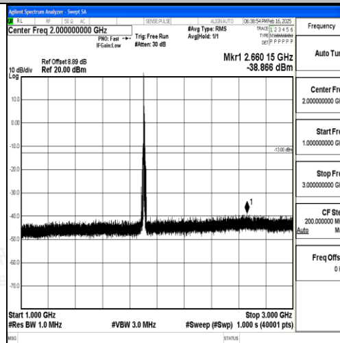
Band2_10MHz_QPSK_19150_1RB#0_1000~3000_1000~3000
