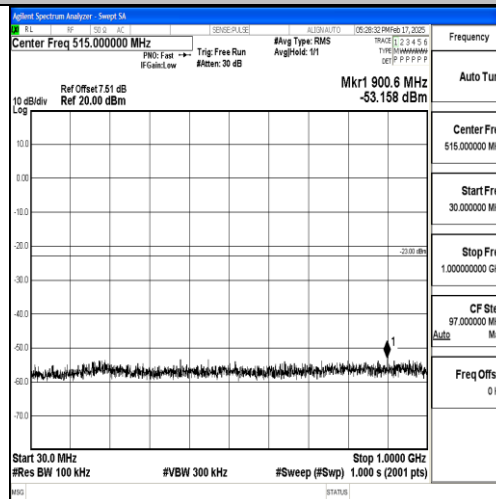
Band2_3MHz_16QAM_19185_1RB#0_30~1000_30~1000
