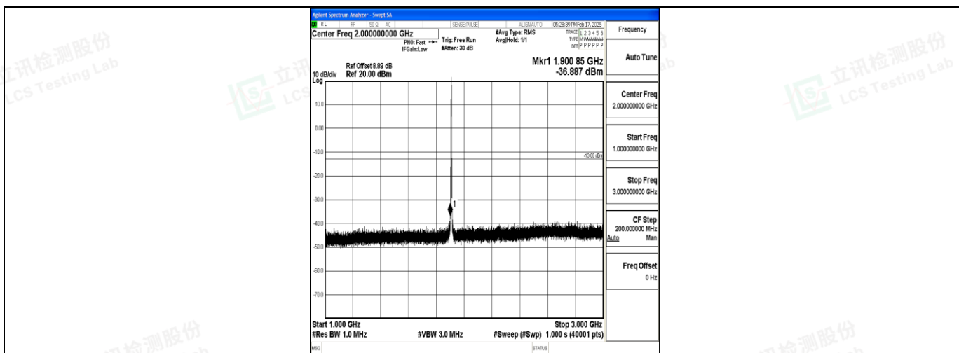
Band2_3MHz_16QAM_19185_1RB#0_1000~3000_1000~3000
