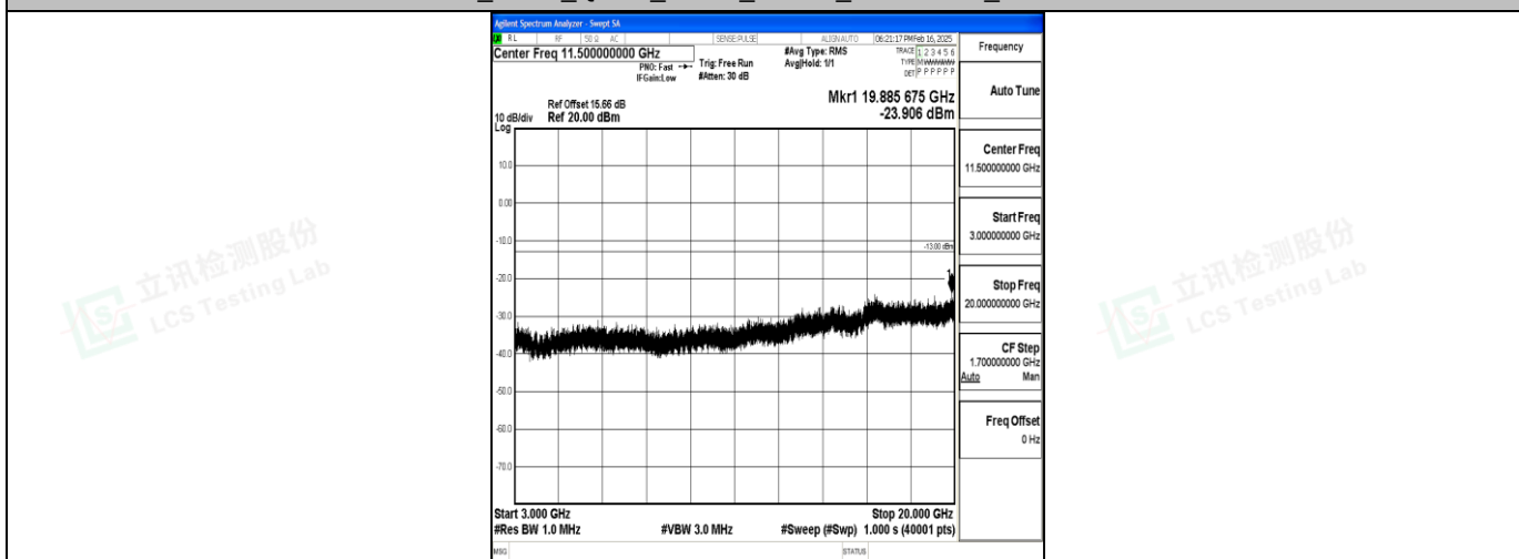
Band2_5MHz_QPSK_19175_1RB#0_3000~20000_3000~20000
