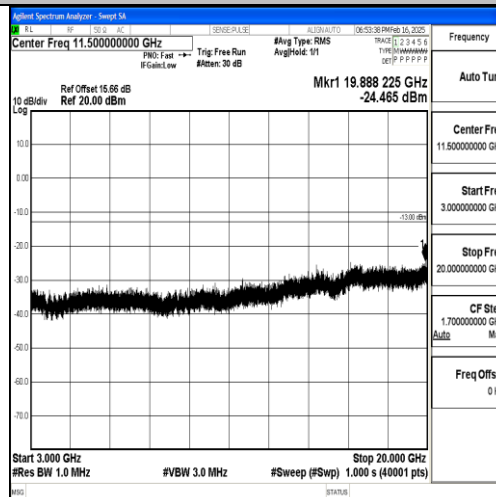
Band2_15MHz_16QAM_18675_1RB#0_3000~20000_3000~20000
