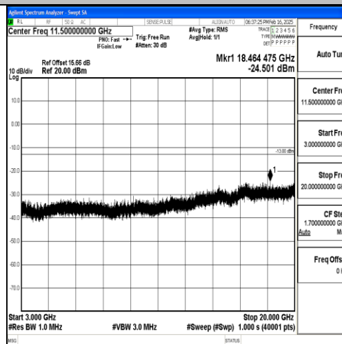
Band2_10MHz_16QAM_18650_1RB#0_3000~20000_3000~20000
