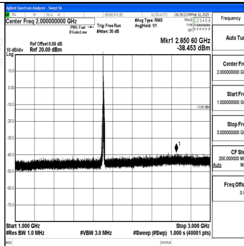
Band2_10MHz_16QAM_19150_1RB#0_1000~3000_1000~3000
