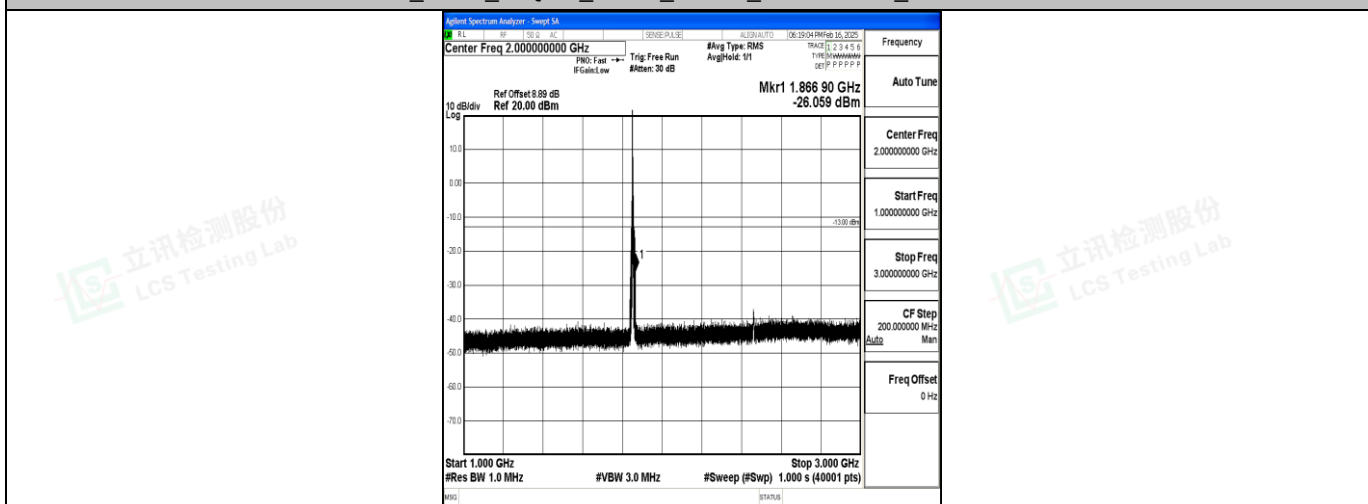
Band2_5MHz_QPSK_18625_1RB#0_1000~3000_1000~3000
