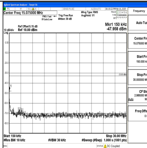
Band2_5MHz_16QAM_18625_1RB#0_0.15~30_0.15~30
