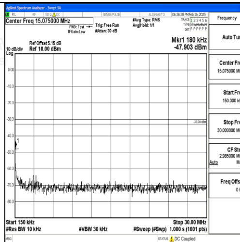
Band2_10MHz_QPSK_18650_1RB#0_0.15~30_0.15~30
