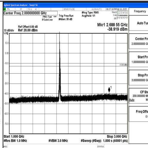
Band2_10MHz_16QAM_18650_1RB#0_1000~3000_1000~3000
