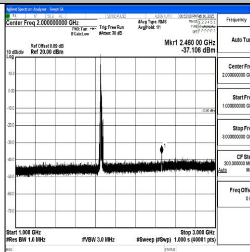
Band2_15MHz_QPSK_18675_1RB#0_1000~3000_1000~3000
