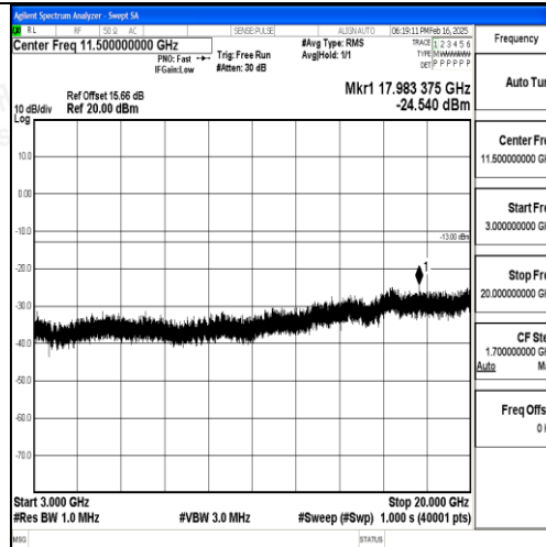
Band2_5MHz_QPSK_18625_1RB#0_3000~20000_3000~20000
