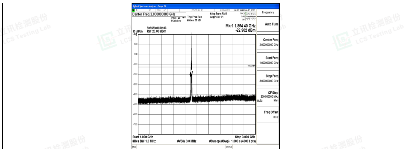
Band2_5MHz_16QAM_19175_1RB#0_1000~3000_1000~3000
