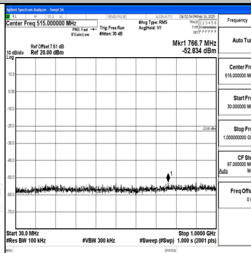
Band2_15MHz_QPSK_18675_1RB#0_30~1000_30~1000
