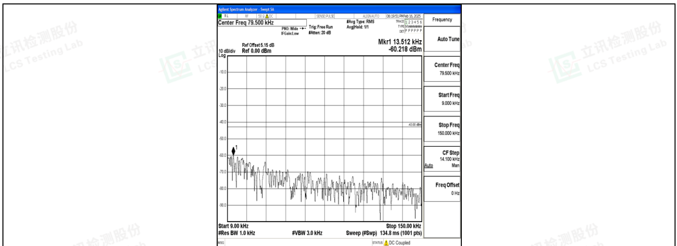
Band2_5MHz_QPSK_18900_1RB#0_0.009~0.15_0.009~0.15
