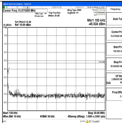
Band2_10MHz_16QAM_18900_1RB#0_0.15~30_0.15~30
