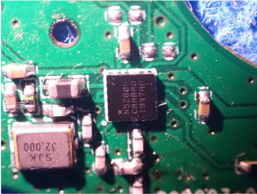
INTERNAL VIEW-1 OF EUT(K11)
