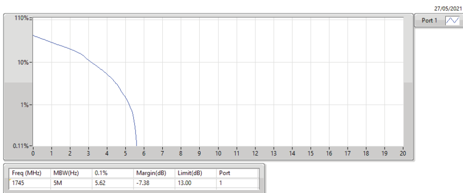
Band 66_LTE_1.4MHz_Nss1,16QAM_1TX 1745MHz_16QAM_RB 3,#RB M
