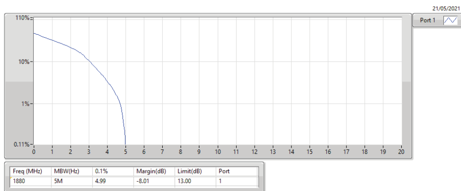
Band 2_LTE_1.4MHz_Nss1,16QAM_1TX 1880MHz_16QAM_RB 3,#RB M
