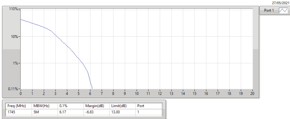
Band 66_LTE_1.4MHz_Nss1,16QAM_1TX 1745MHz_16QAM_RB 6,#RB 0
