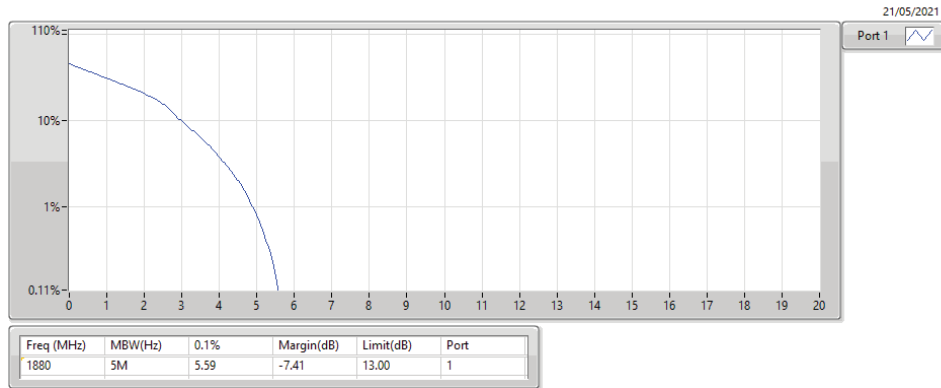
Band 2_LTE_1.4MHz_Nss1,16QAM_1TX 1880MHz_16QAM_RB 6,#RB 0
