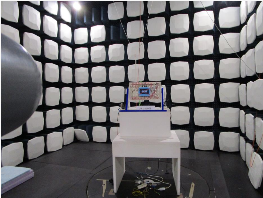
Photograph 5: EUT test setup in the fully anechoic chamber, overview
