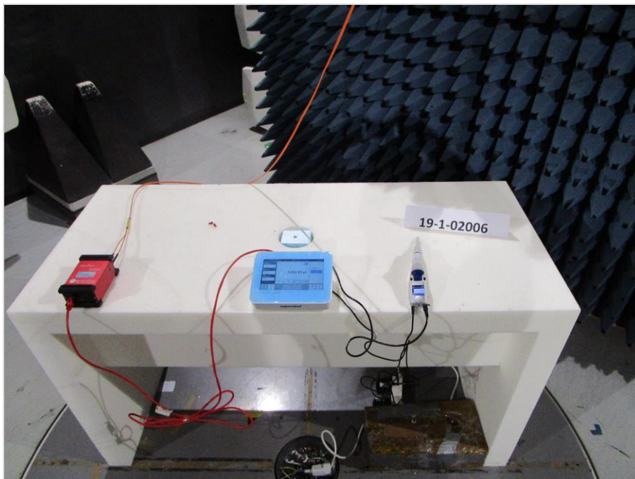
Photograph 2: EUT test setup in the semi anechoic chamber, close up view
