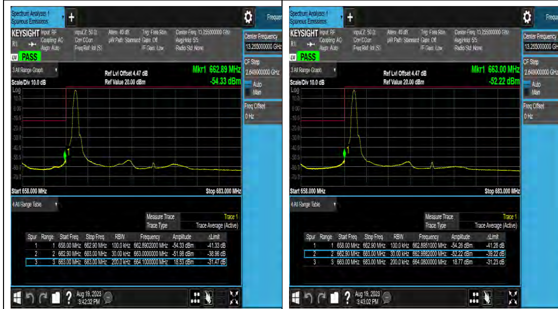
Band71_20MHz_64QAM_133222_1RB#0
