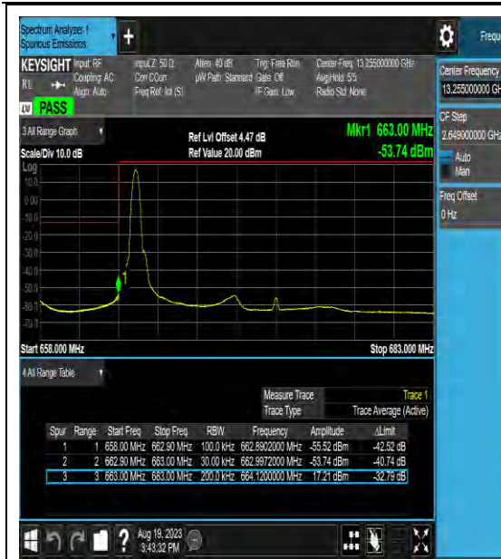
Band71_20MHz_16QAM_133222_1RB#99
