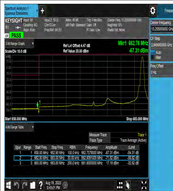
Band71_20MHz_16QAM_133222_100RB#0
