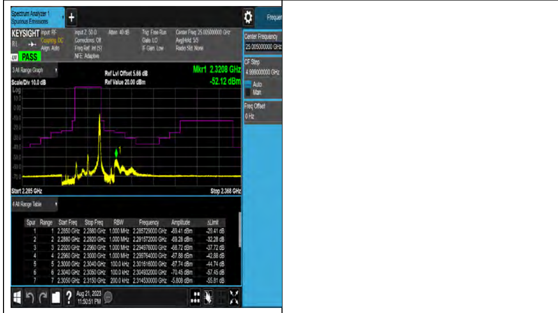
Band40_10MHz_16QAM_38750_1RB#49
