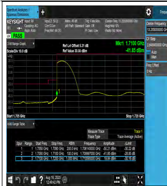
Band4_10MHz_16QAM_20000_1RB#49
