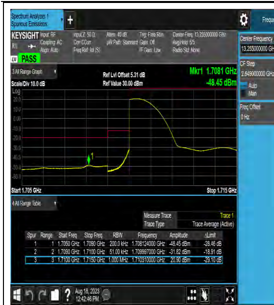
Band4_5MHz_64QAM_19975_1RB#0
