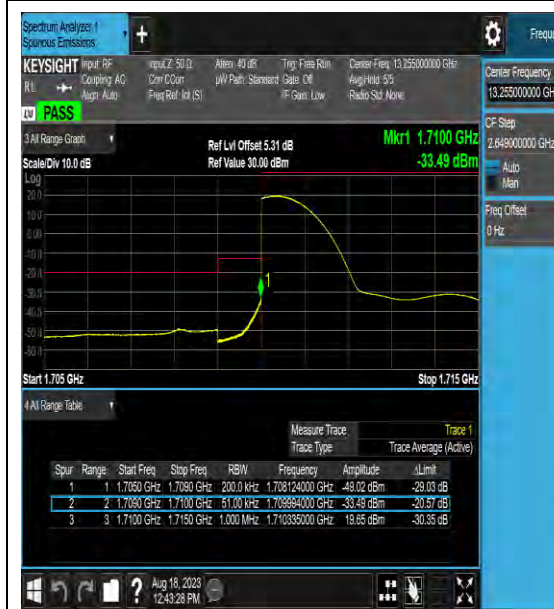
Band4_5MHz_16QAM_19975_1RB#24
