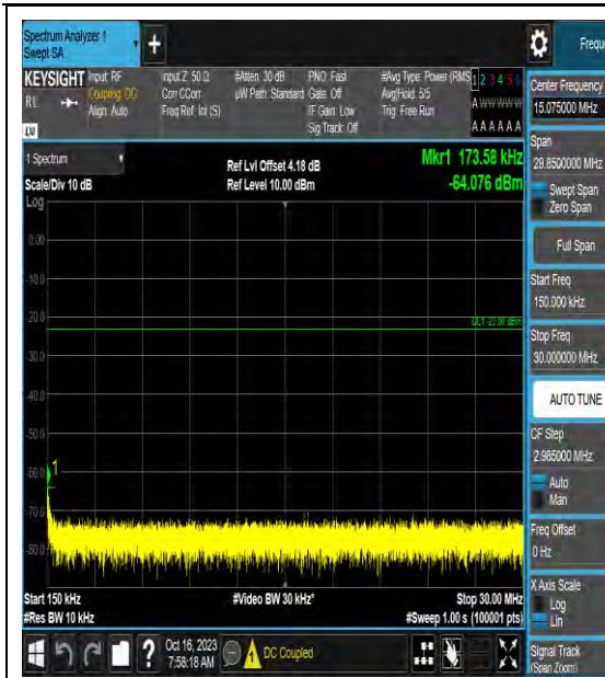
Band26_15MHz_16QAM_26965_1RB#0_1000~3000_1000~3000
