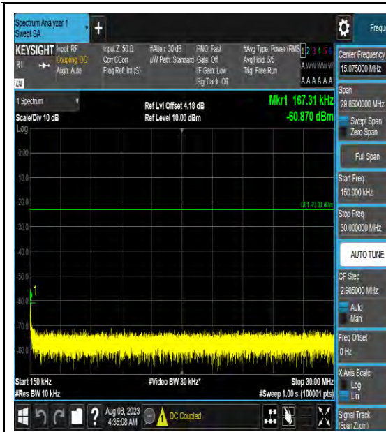
Band12_10MHz_QPSK_23060_1RB#0_1000~3000_1000~3000
