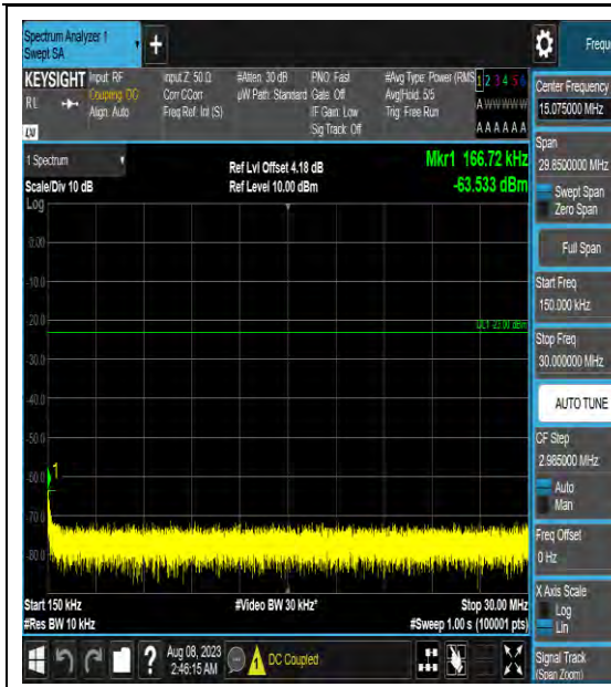
Band12_1.4MHz_16QAM_23173_1RB#0_1000~3000_1000~3000
