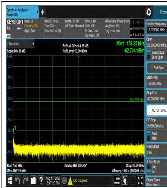
Band2_15MHz_16QAM_19125_1RB#0_1000~3000_1000~3000
