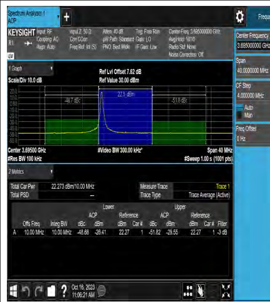
Band48-10MHz-16QAM-56690-1RB#49-PASS
