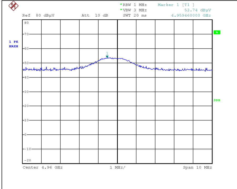
Spurious – Peak
