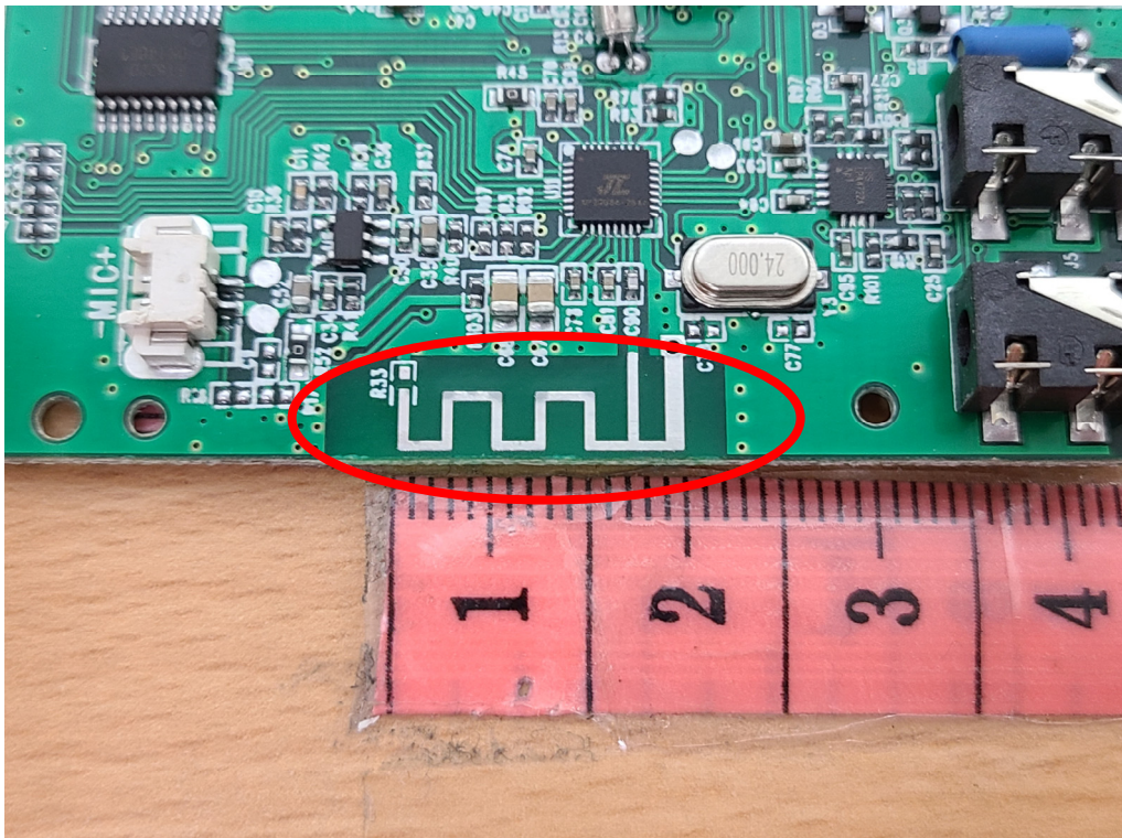
FMT Antenna
