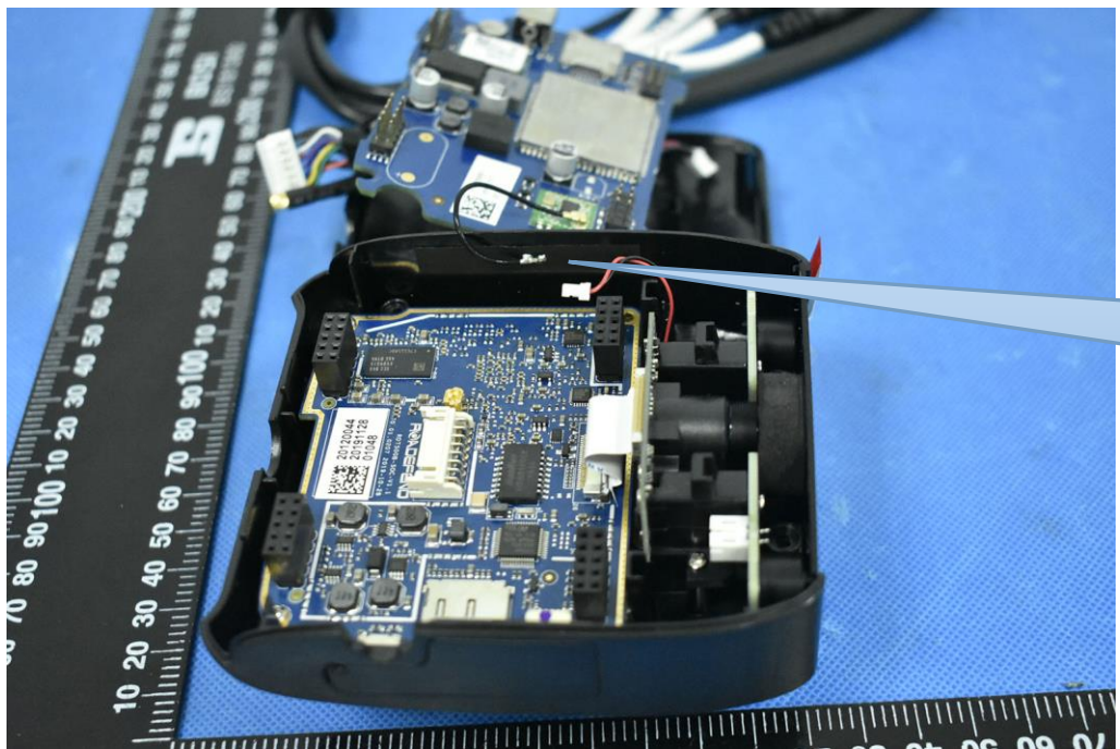
WIFI antenna location
