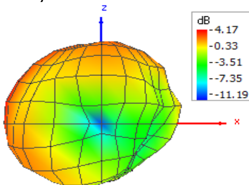
Theta = 90, Phi = 270
