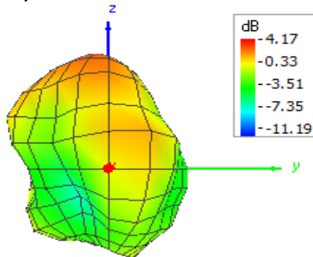
Theta = 90, Phi = 0
