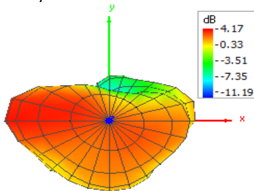
Theta = 0, Phi = 0
