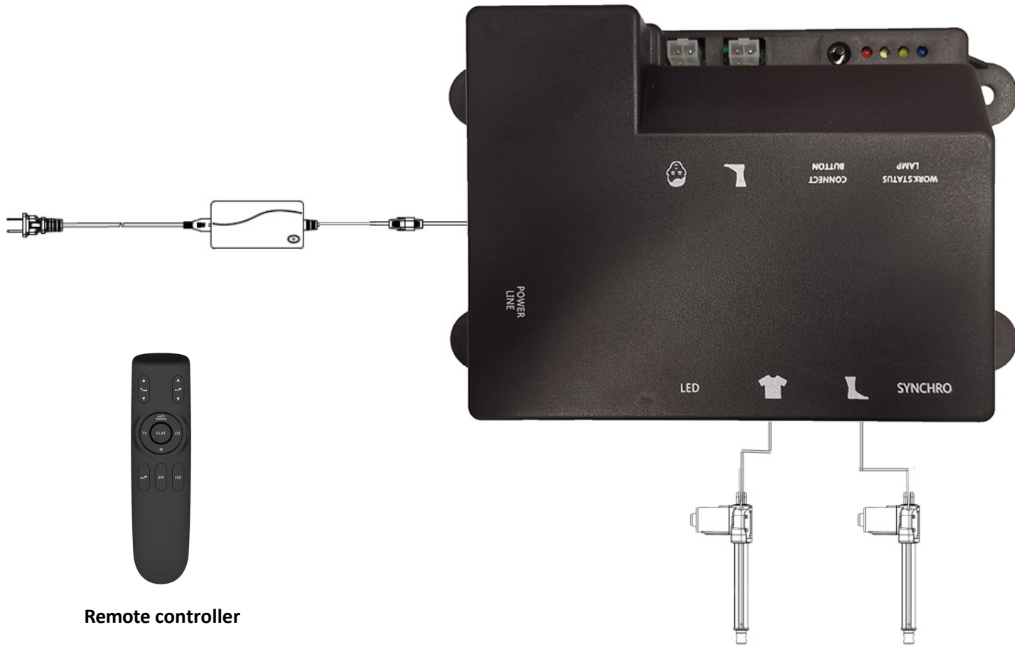
Control box
