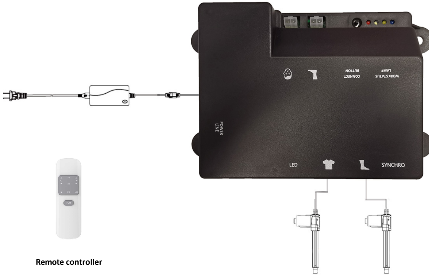
Control box
