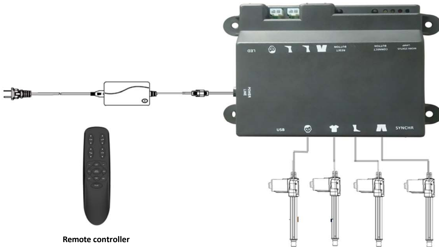
Control box
