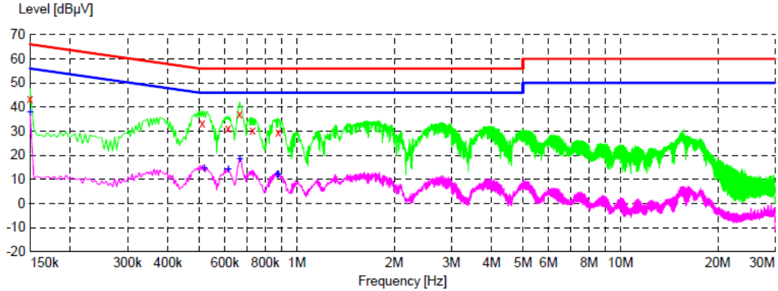
Line Conducted Emission Test Line 1-L
