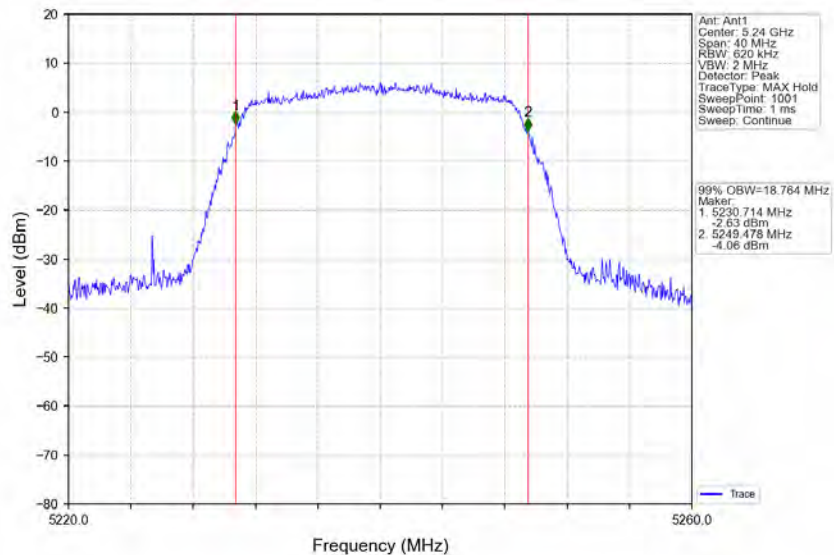
802.11ac(VHT20)_HCH_5240MHz_Ant1_NTNV
