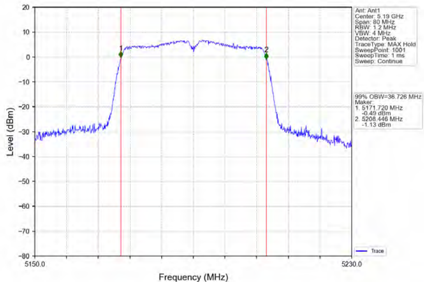
802.11ac(VHT40)_LCH_5190MHz_Ant1_NTNV
