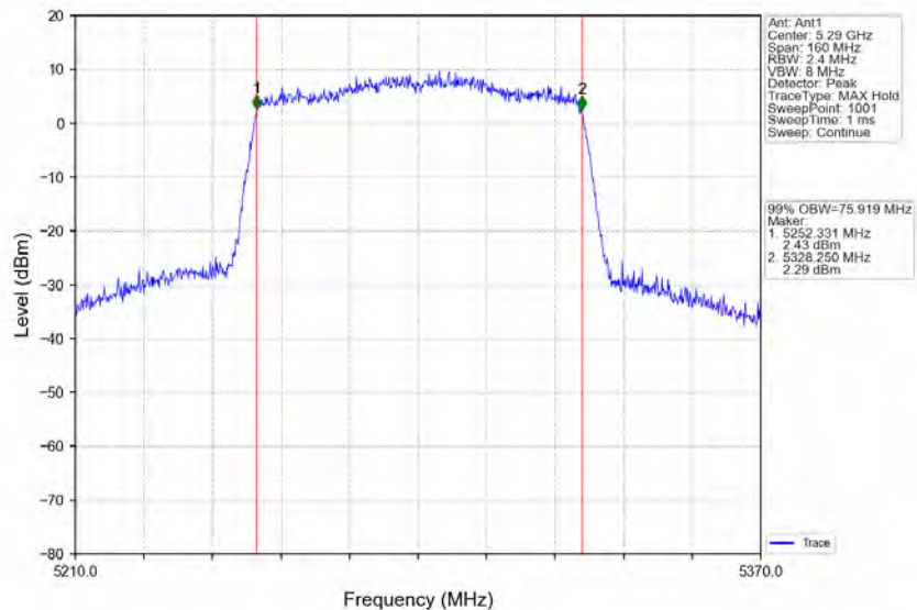
802.11ac(VHT80)_MCH_5290MHz_Ant1_NTNV
