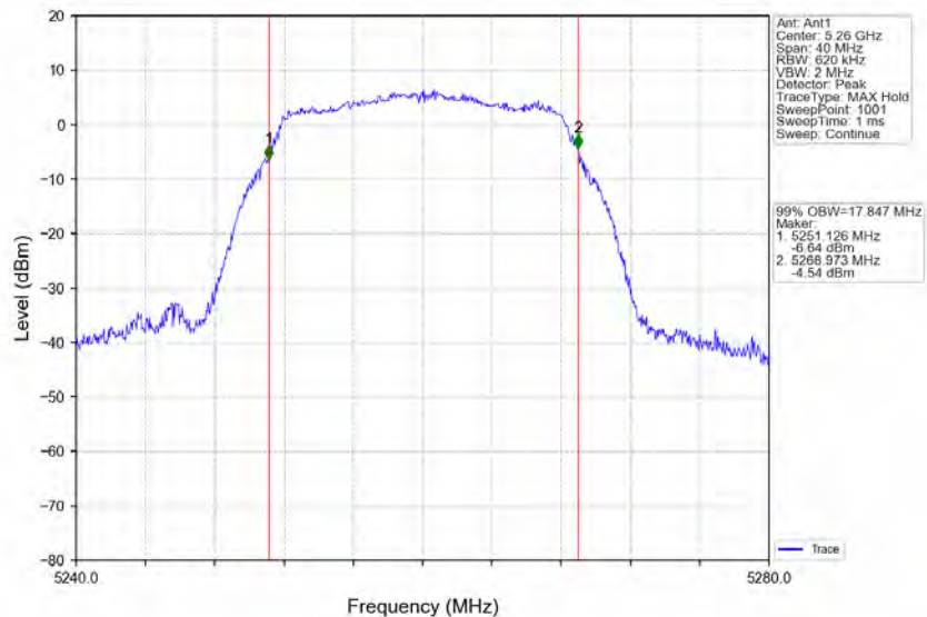
802.11a_LCH_5260MHz_Ant1_NTNV
