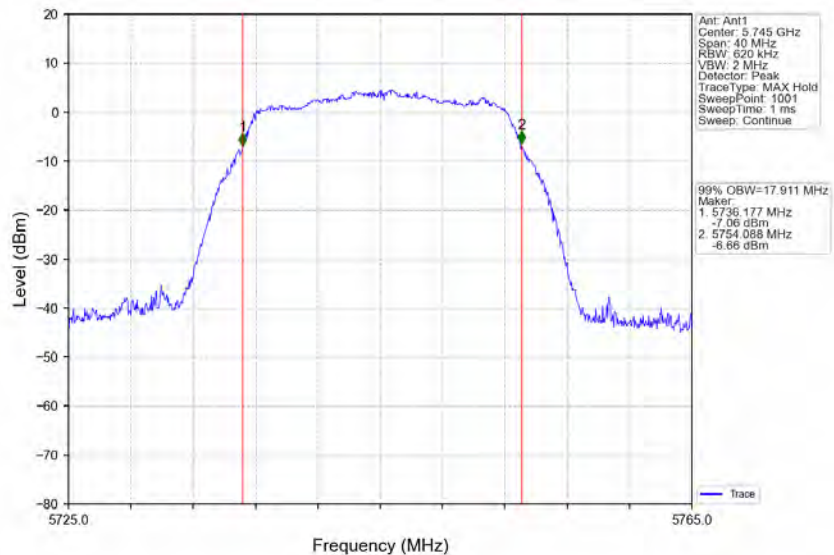
802.11a_LCH_5745MHz_Ant1_NTNV
