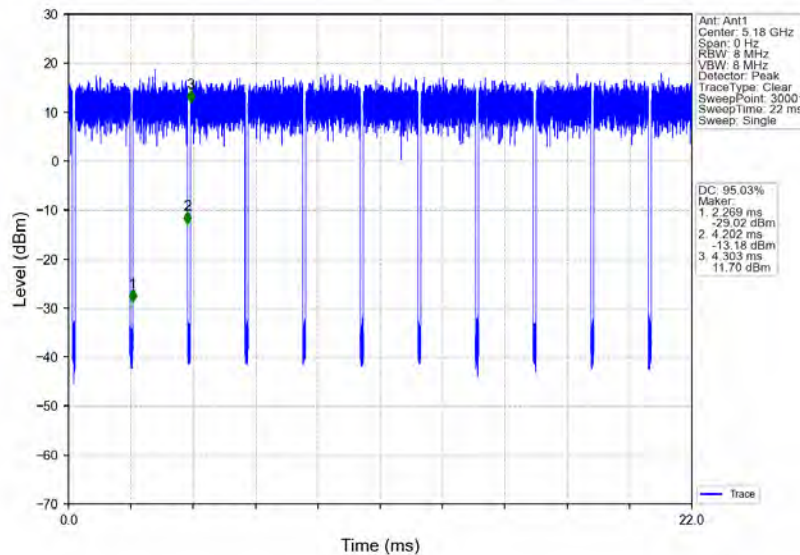
802.11ac(VHT20)_LCH_5180MHz_Ant1_NTNV
