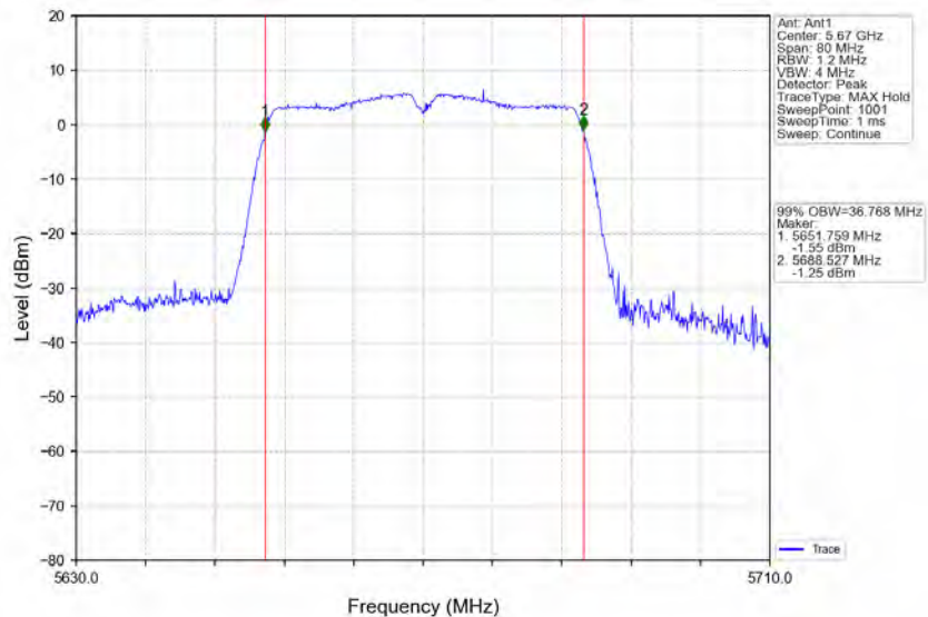
802.11ac(VHT40)_HCH_5670MHz_Ant1_NTNV
