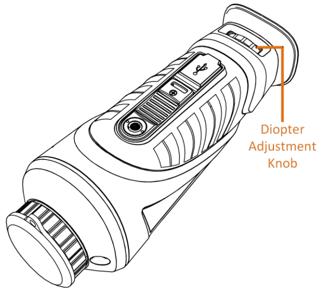
Figure 3-2 Adjust Diopter
