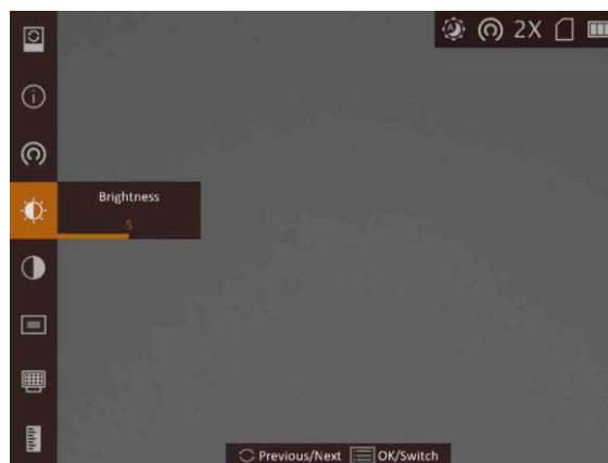
Figure 2-1 Menu Interface
