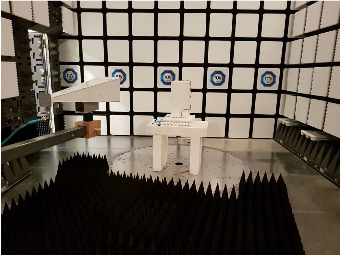
Figure 6 – Radiated Emissions Setup 4GHz to 18GHz Spurious Scans & Band-Edge Measurements
