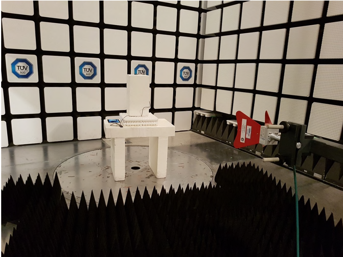
Figure 5 – Radiated Emissions Setup 1GHz to 4GHz Spurious Scans
