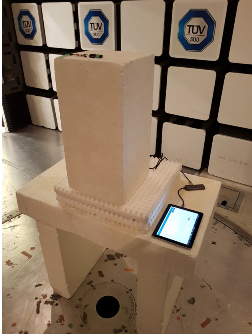
Figure 2 – Radiated Emissions Setup Z-Axis
