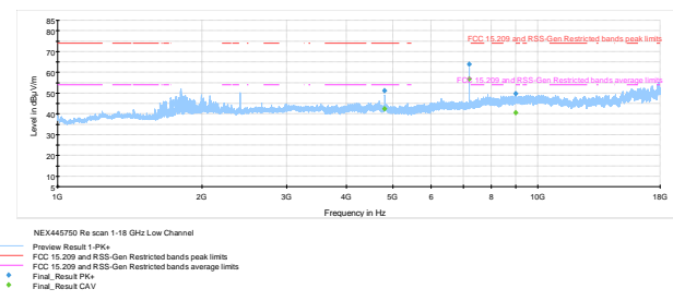
Figure 8.6-9: Radiated spurious emissions on Low channel
