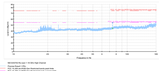
Figure 8.6-11: Radiated spurious emissions on High channel
