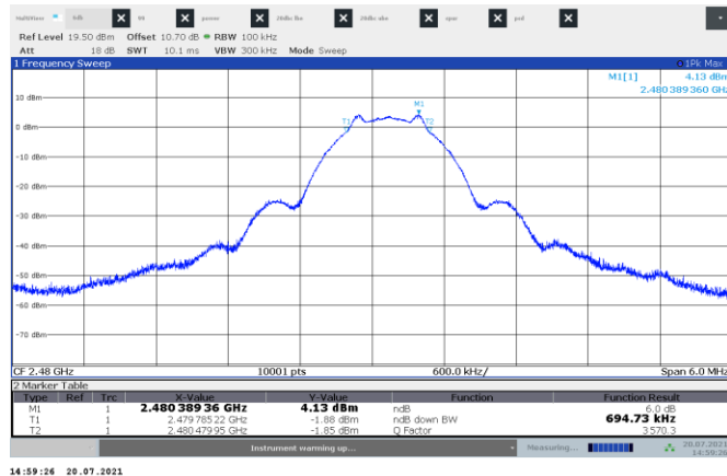
Figure 8.4-3: 6 dB bandwidth High channel
