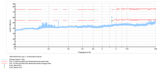
Figure 8.6-10: Radiated spurious emissions on Mid channel
