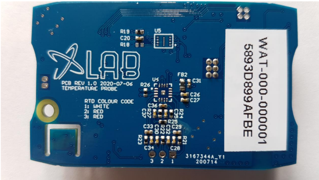
AT-105 Circuit Card Bottom
