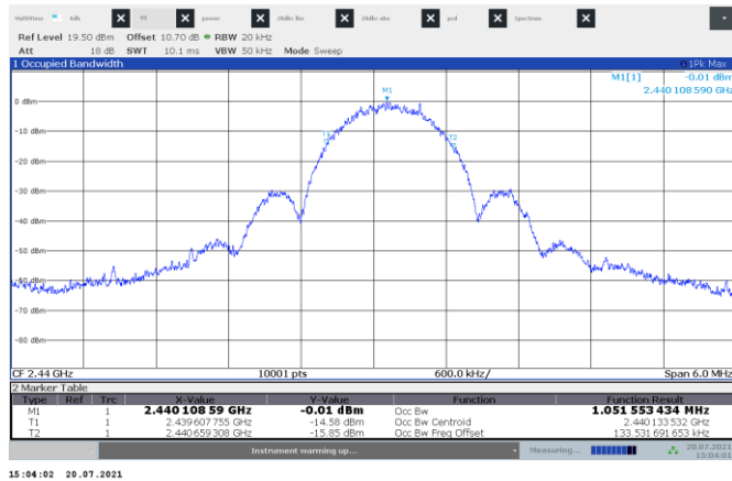
Figure 7.4-5: 99% occupied bandwidth Mid channel
