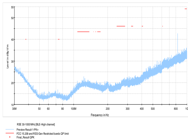
Figure 7.6-10: Radiated spurious emissions on high channel
