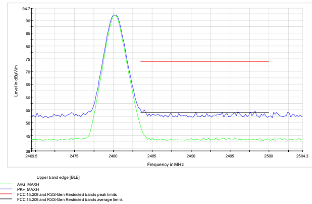
Figure 7.6-2: Band edge radiated spurious emissions at 2483.5 MHz
