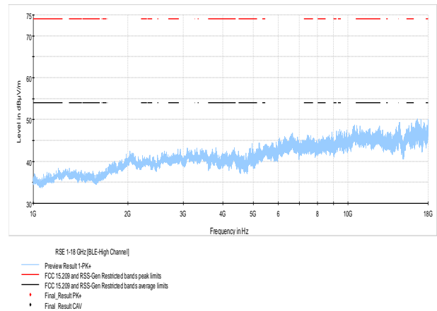
Figure 7.6-13: Radiated spurious emissions on High channel
