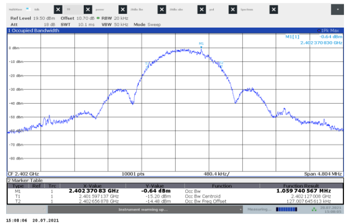
Figure 7.4-4: 99% occupied bandwidth Low channel
