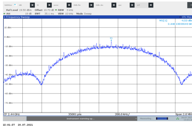
Figure 7.7-2: PSD on mid channel
