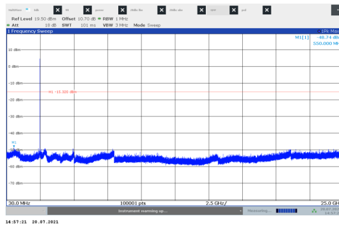
Figure 7.6-7: Conducted spurious emissions on High channel
