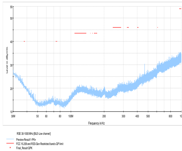
Figure 7.6-8: Radiated spurious emissions on Low channel
