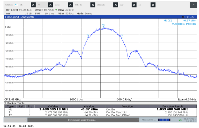
Figure 7.4-6: 99% occupied bandwidth High channel
