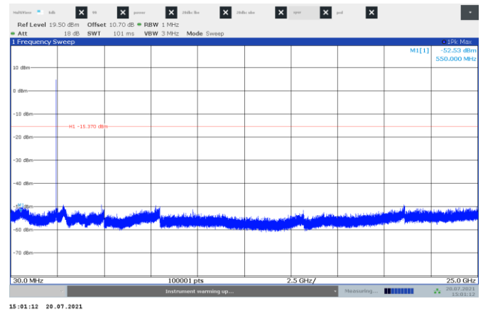
Figure 7.6-6: Conducted spurious emissions on Mid channel
