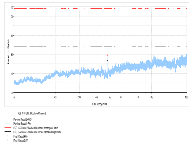
Figure 7.6-11: Radiated spurious emissions on Low channel
