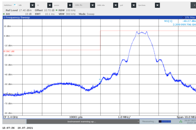
Figure 7.6-3: Band edge conducted emissions at 2400 MHz
