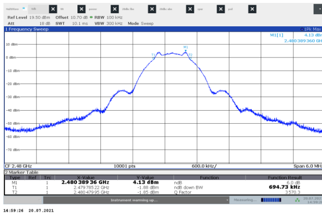
Figure 7.4-3: 6 dB bandwidth High channel
