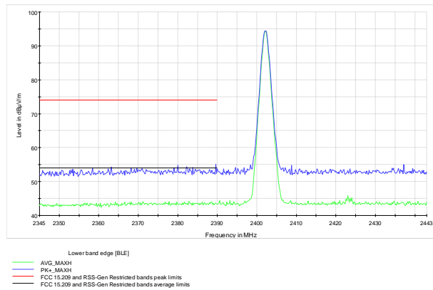
Figure 7.6-1: Band edge radiated spurious emissions at 2390 MHz
