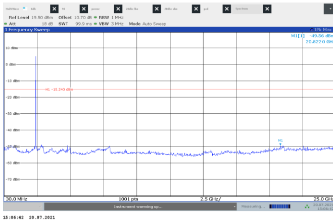
Figure 7.6-5: Conducted spurious emissions on Low channel
