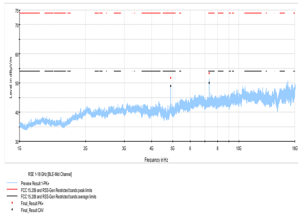
Figure 7.6-12: Radiated spurious emissions on Mid channel
