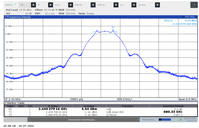
Figure 7.4-2: 6 dB bandwidth Mid channel
