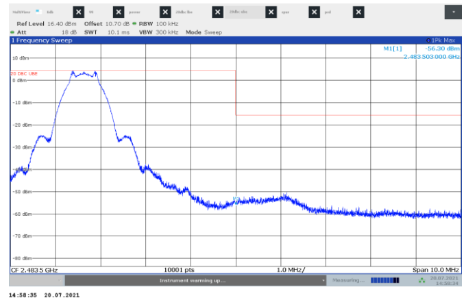
Figure 7.6-4: Band edge conducted emissions at 2483.5 MHz
