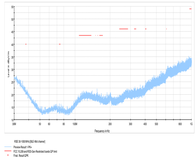
Figure 7.6-9: Radiated spurious emissions on Mid channel
