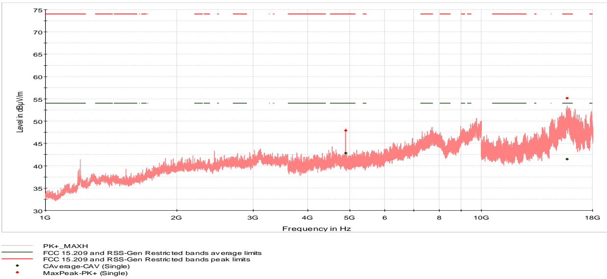
Figure 8.7-14: Radiated spurious (out-of-band) emissions, 1 GHz to 18 GHz, Mid channel
