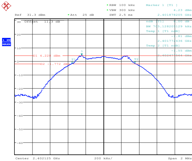
Figure 8.5-1: 6 dB bandwidth on low channel
