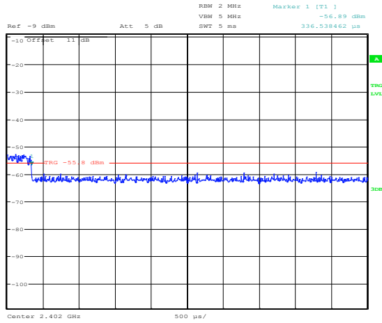
Figure 8.7-8: Pulse width
