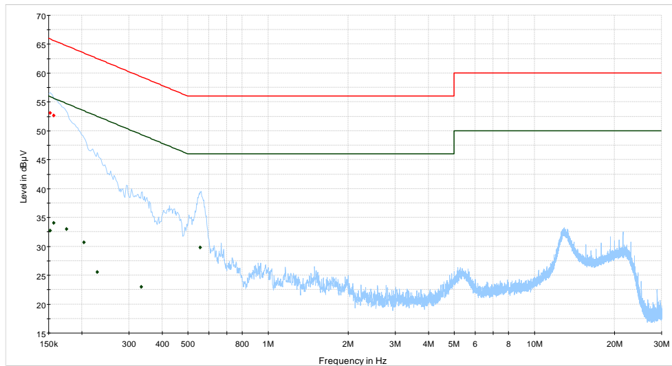
CE 120 VAC 60 Hz Neutral [Charging Mode] — Preview Result 1-PK+ — CISPR 32 Limit - Class B, Mains (QP) — CISPR 32 Limit - Class B, Mains (Avg) ♦ Final_Result QPK ♦ Final_Result CAV
