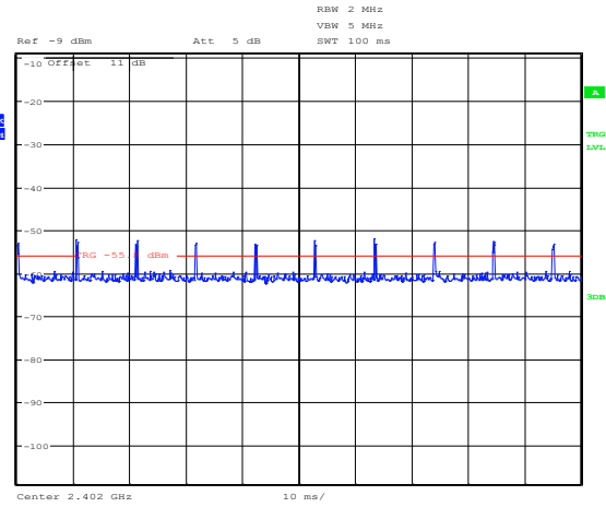
Figure 8.7-9: Pulses per 100 ms
