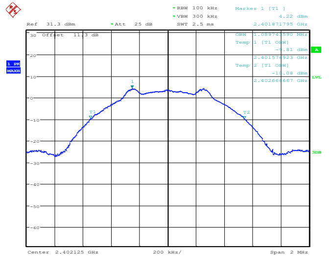
Figure 8.5-4: 99% occupied bandwidth - sample plot
