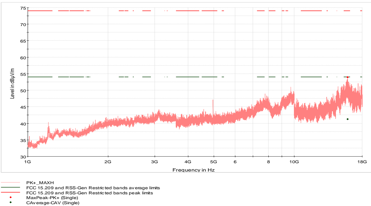
Figure 8.7-15: Radiated spurious (out-of-band) emissions, 1 GHz to 18 GHz, high channel
