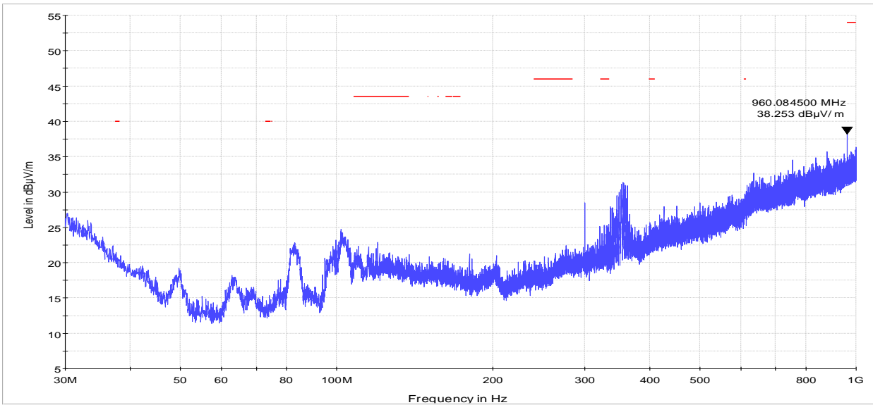
Figure 8.7-11: Radiated spurious (out-of-band) emissions, below 1 GHz, Mid channel
