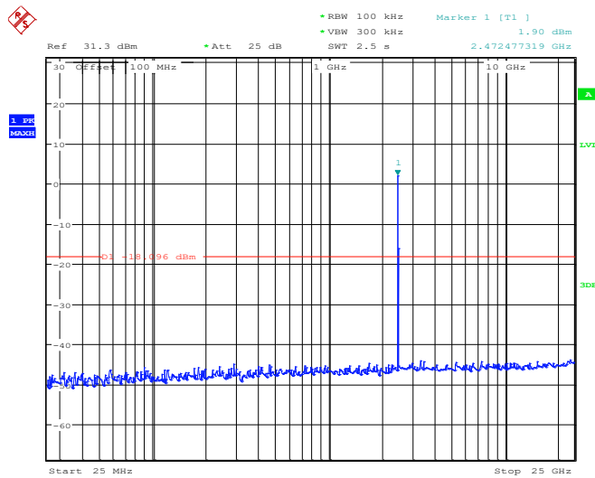
Figure 8.7-3: Conducted spurious (out-of-band) emissions, high channel
