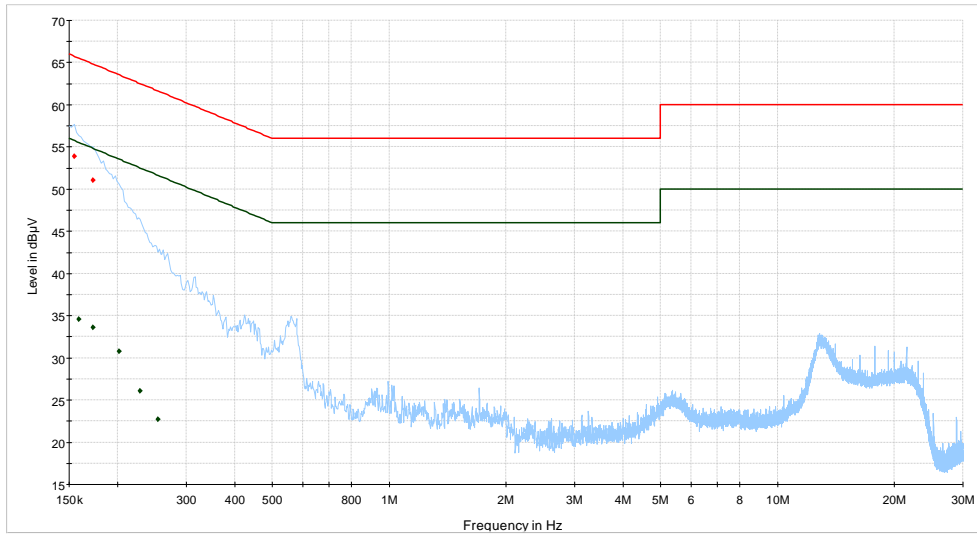
CE 120 VAC 60 Hz Line [Charging Mode] — Preview Result 1-PK+ — CISPR 32 Limit - Class B, Mains (QP) — CISPR 32 Limit - Class B, Mains (Avg) ♦ Final_Result QPK ♦ Final_Result CAV
