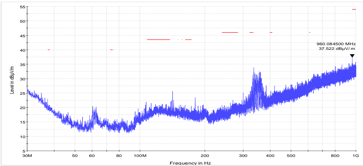
Figure 8.7-10: Radiated spurious (out-of-band) emissions, below 1 GHz, Low channel
