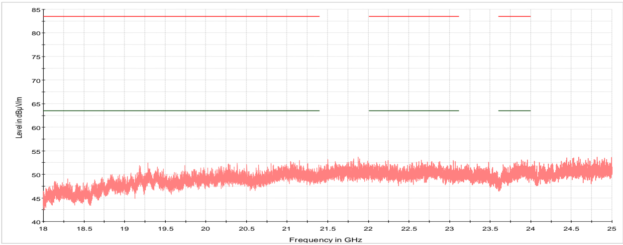
Figure 8.7-18: Radiated spurious (out-of-band) emissions, 18 GHz to 25 GHz, high channel
