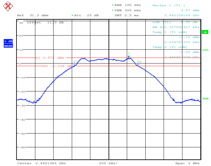
Figure 8.5-2: 6 dB bandwidth on mid channel
