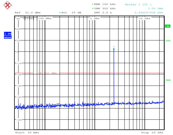
Figure 8.7-2: Conducted spurious (out-of-band) emissions, mid channel
