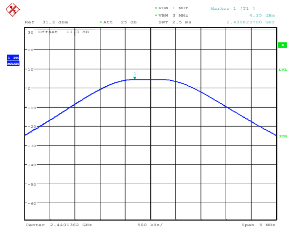
Figure 8.6-2: Output power on mid channel
