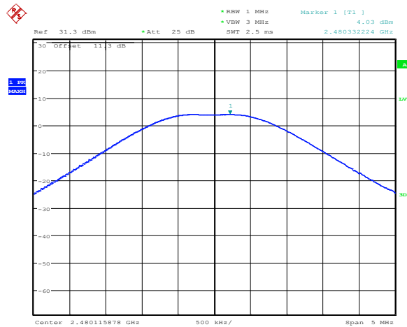
Figure 8.6-3: Output power on high channel
