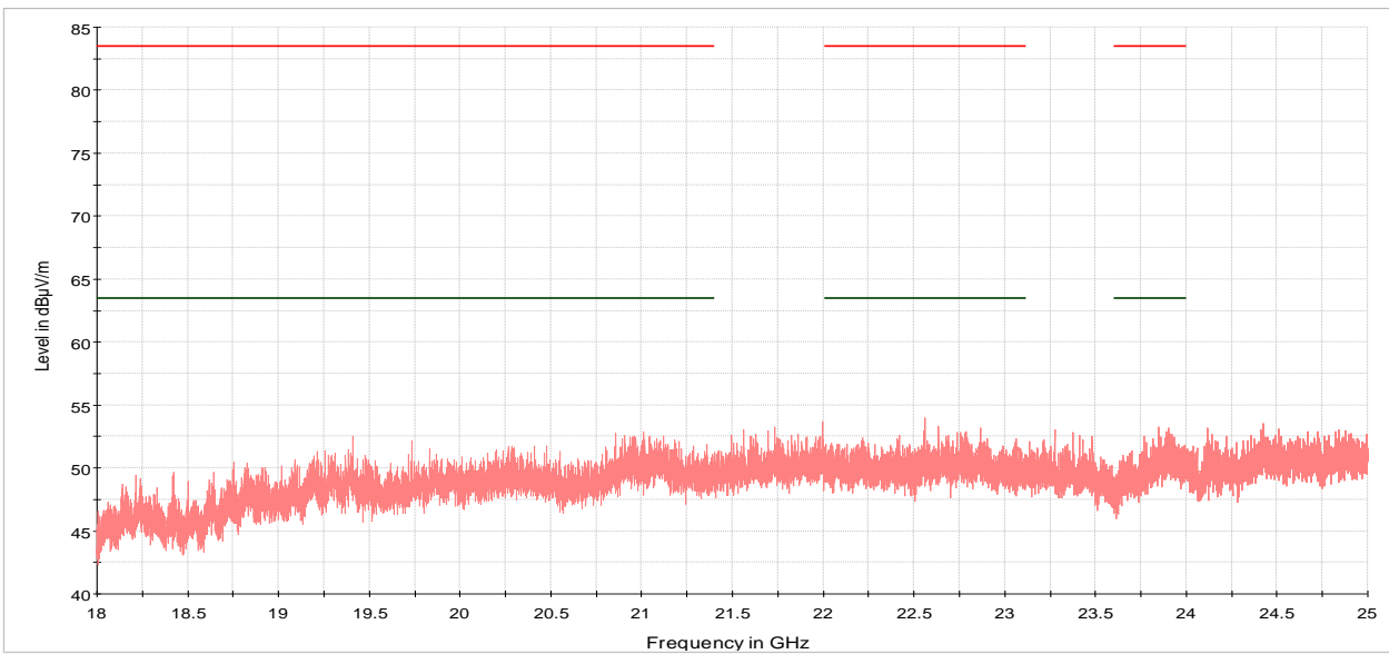
Figure 8.7-16: Radiated spurious (out-of-band) emissions, 18 GHz to 25 GHz, Low channel
