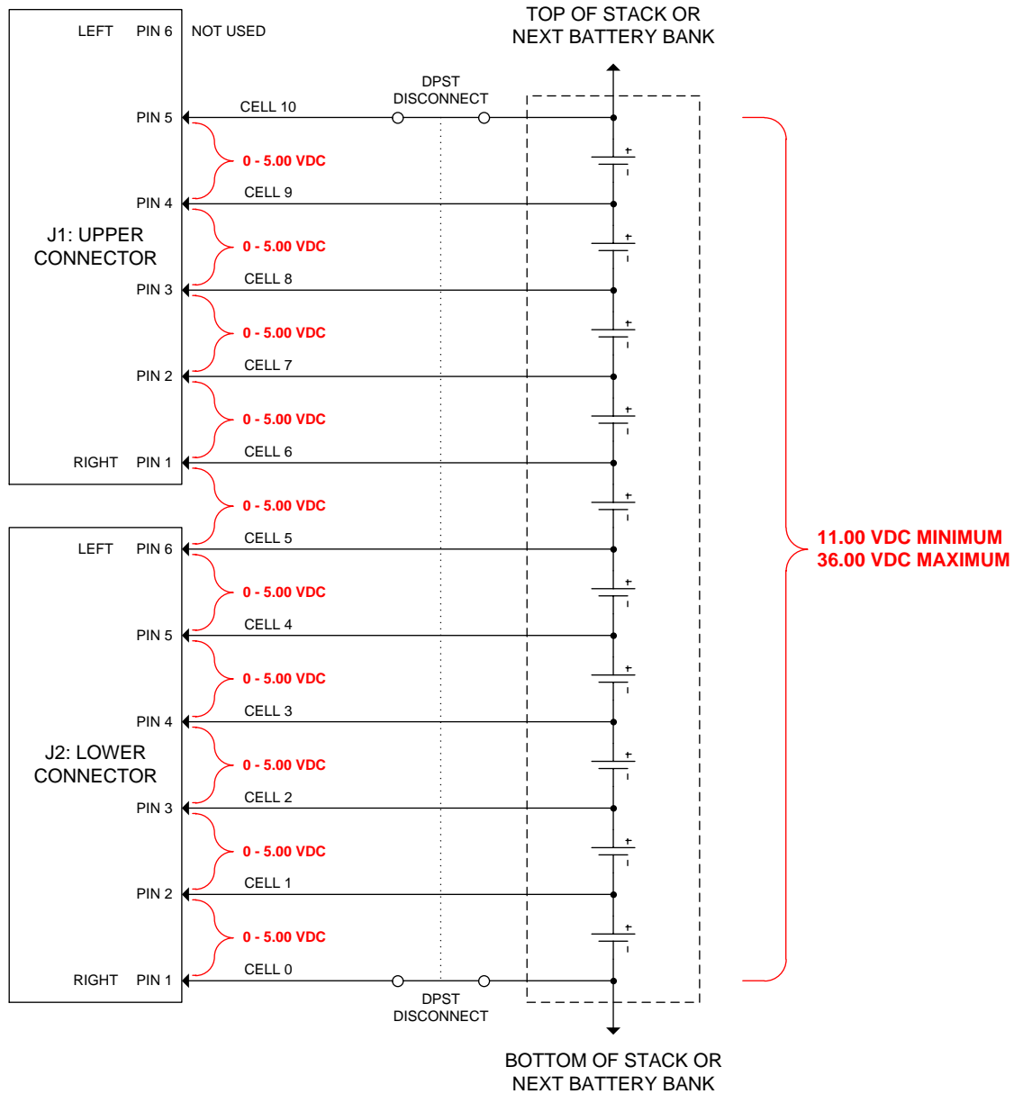
Battery Cell Input Ratings
