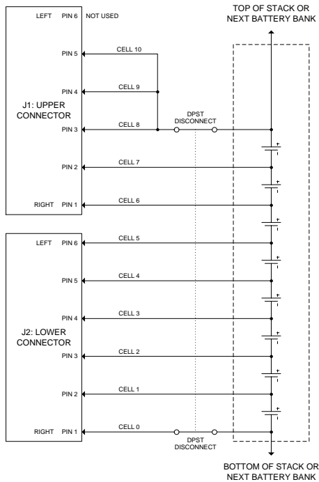
Example 8 Cell Wiring to BMS
