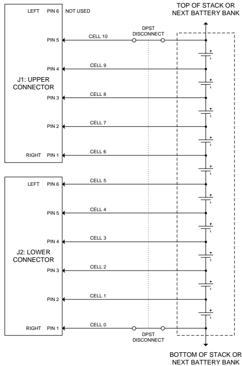
Example 10 Cell Wiring to BMS
