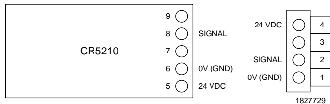
Transducer and BMS Mating Connector Pinouts
