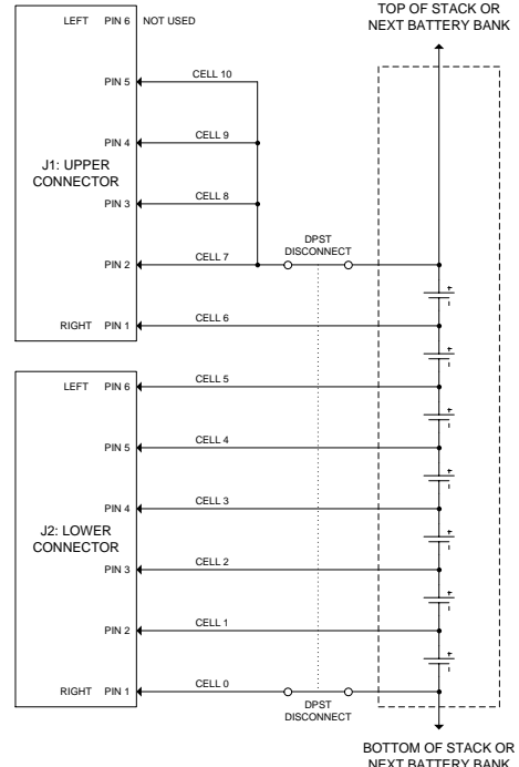
Example 7 Cell Wiring to BMS
