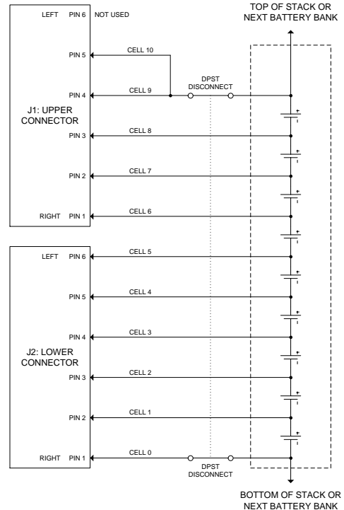
Example 9 Cell Wiring to BMS
