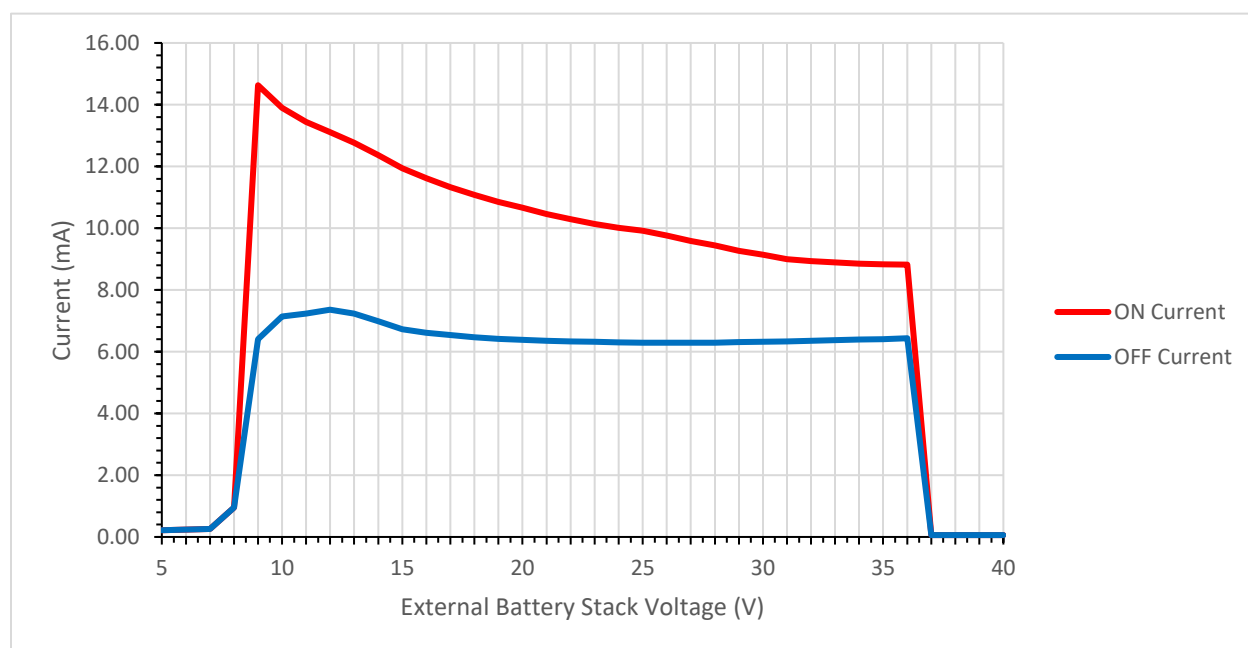
Battery Stack Load Current vs. Battery Stack Voltage
