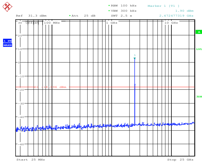
Figure 8.7-3: Conducted spurious (out-of-band) emissions, high channel
