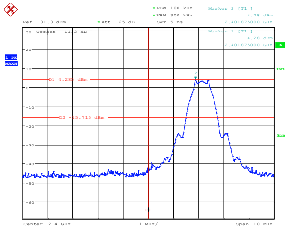
Figure 8.7-4: Conducted spurious (out-of-band) emissions Lower band, low channel)
