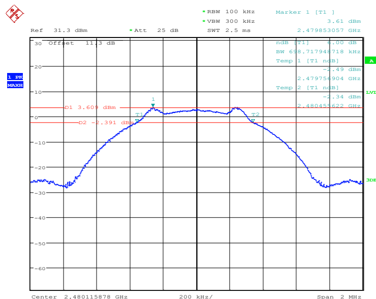
Figure 8.5-3: 6 dB bandwidth on high channel
