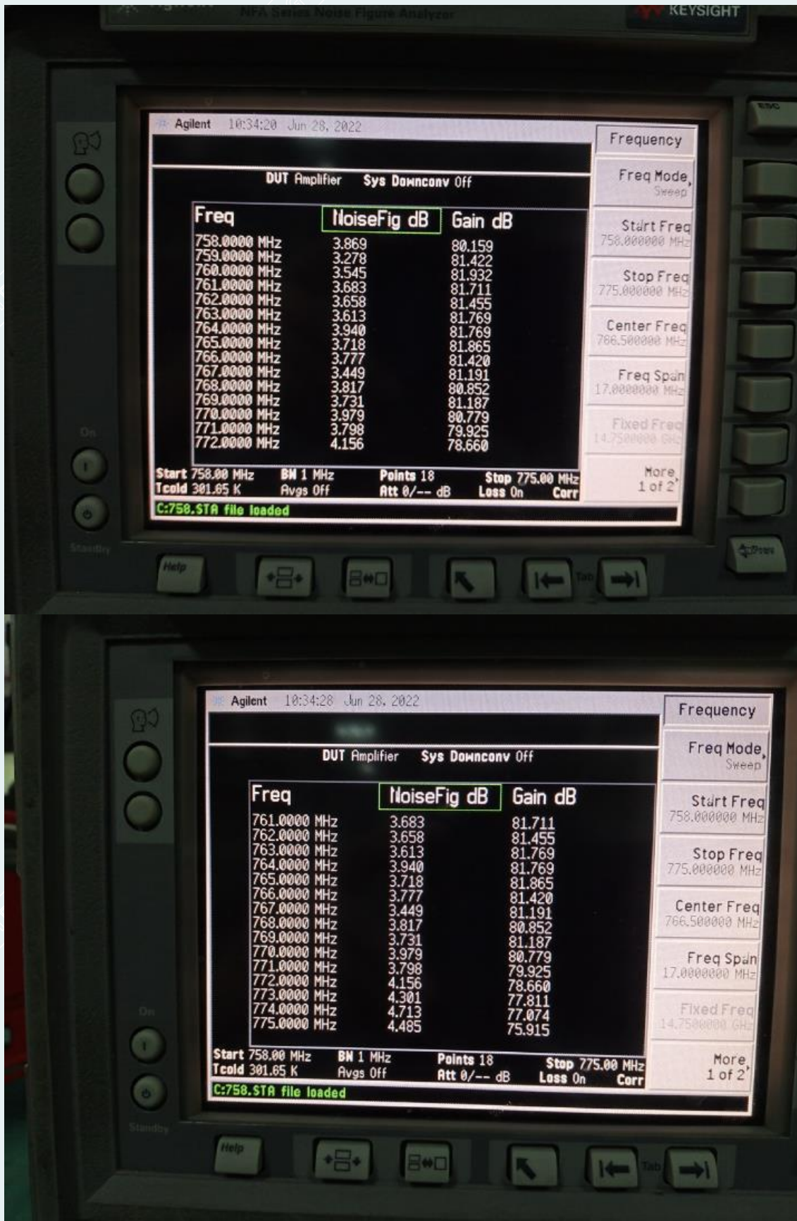
Downlink: 758MHz~775MHz
