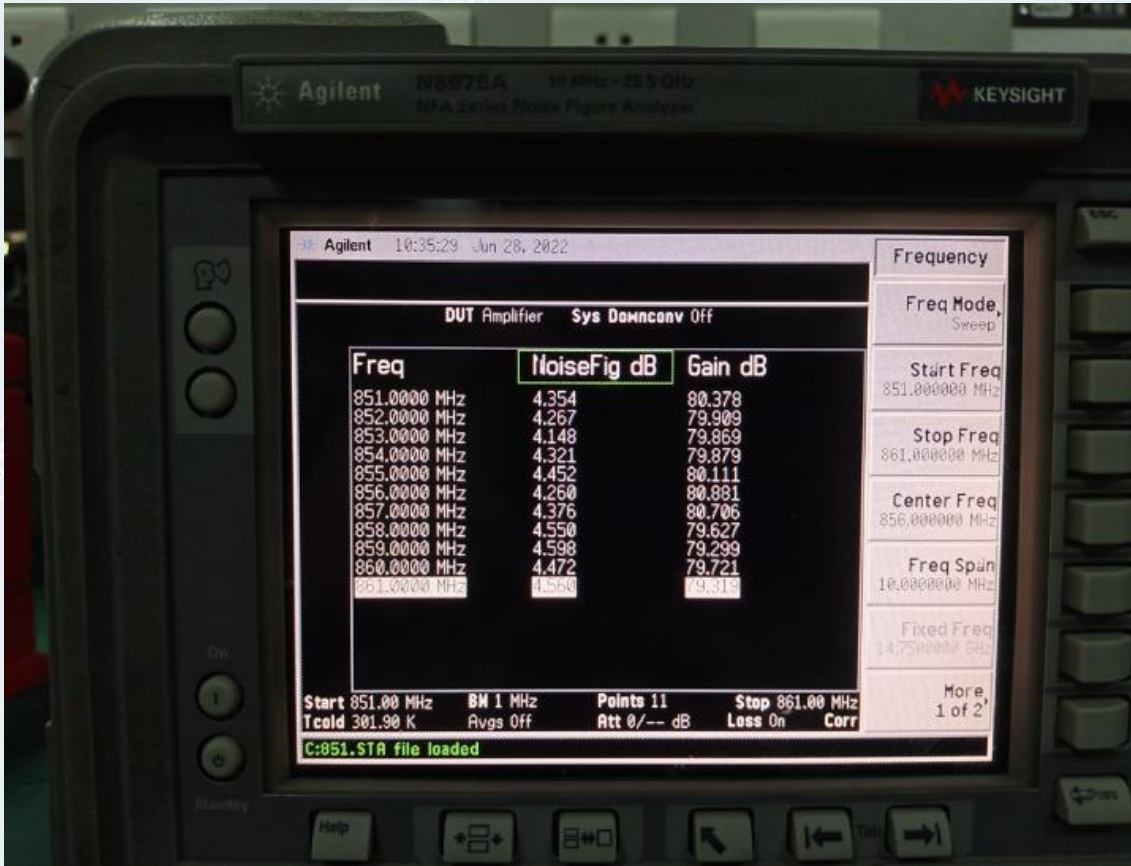
Downlink: 851MHz~861MHz
