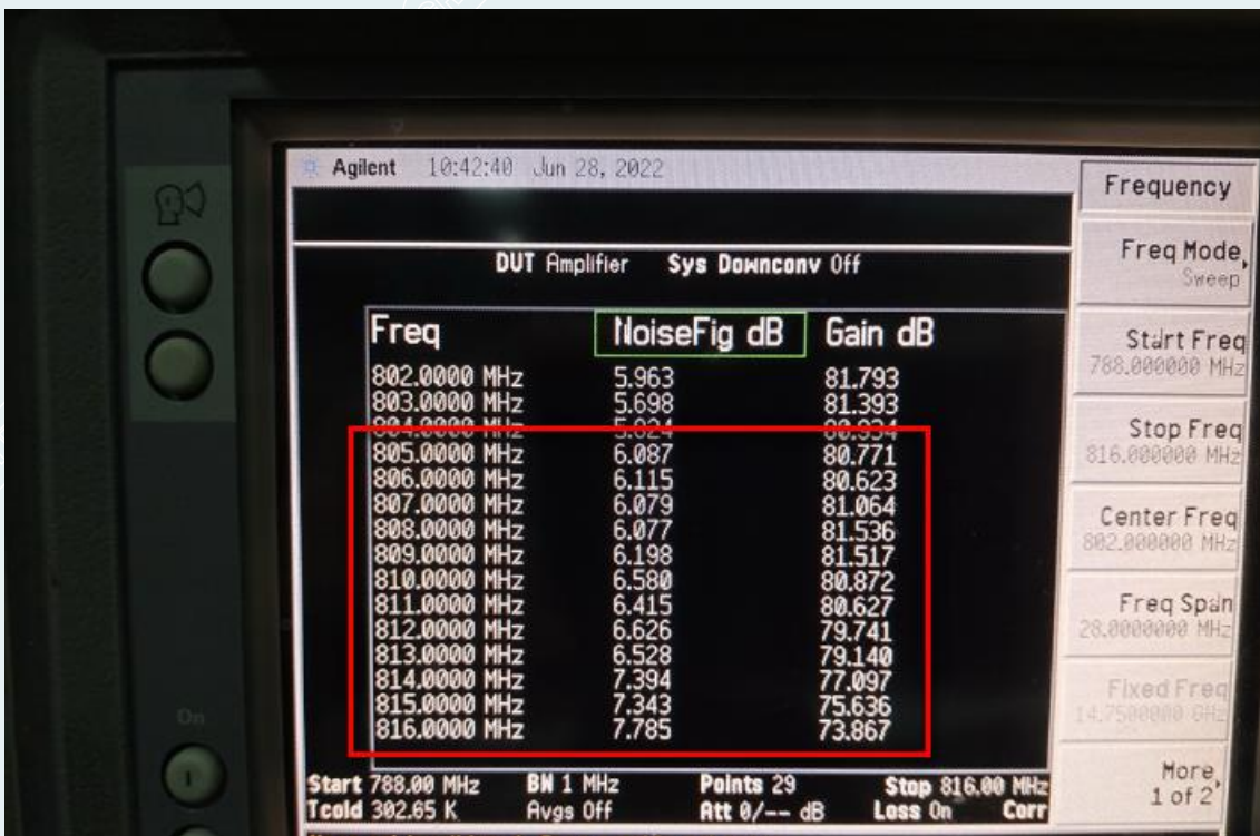
Uplink: 805MHz~816MHz
