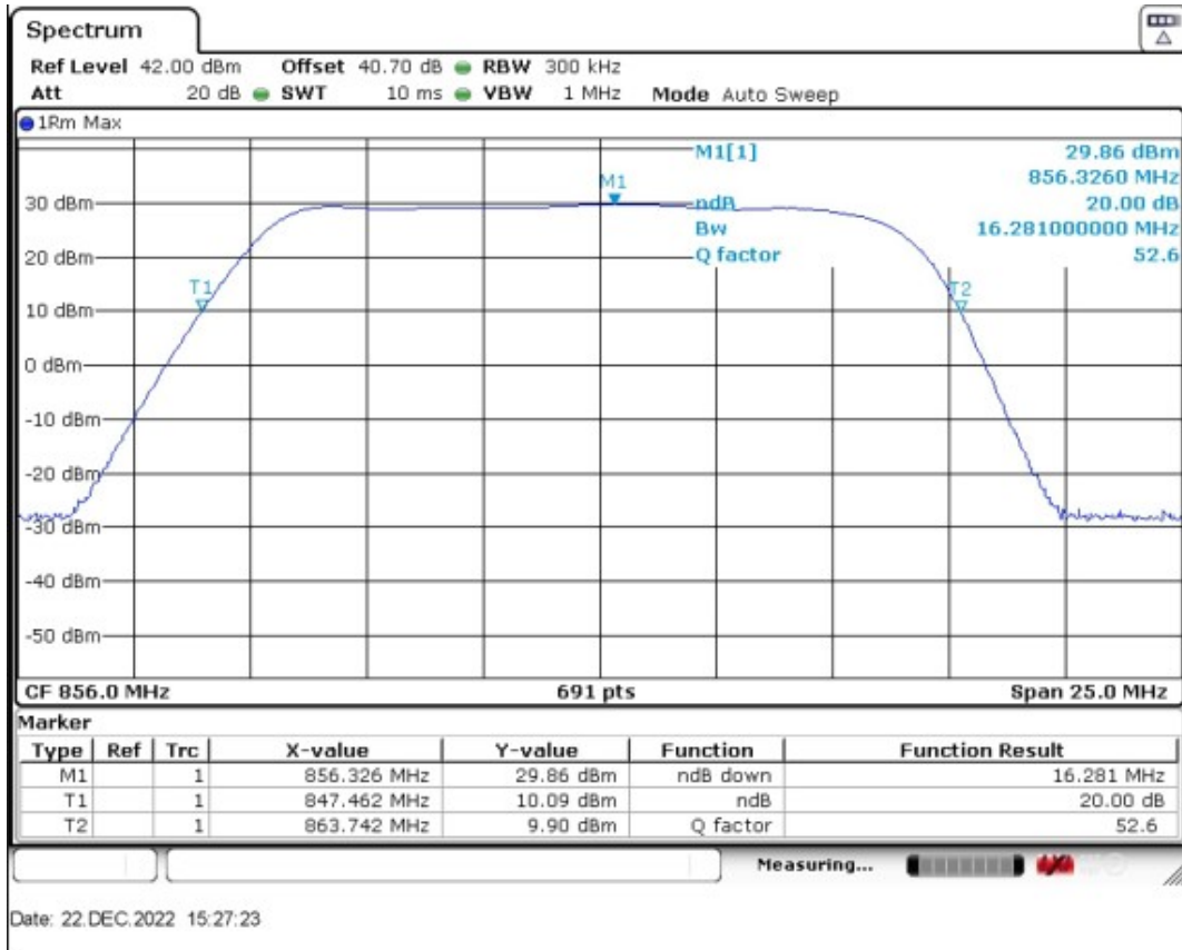
Downlink: 851MHz~861MHz
