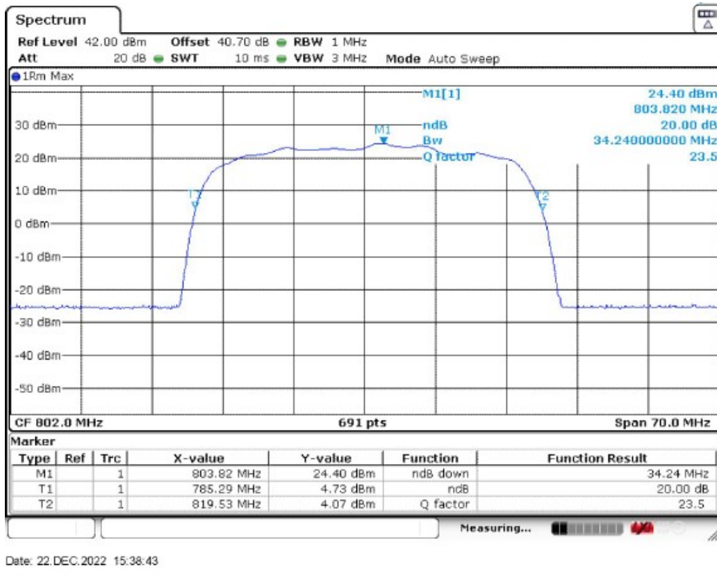
Uplink: 788MHz~816MHz
