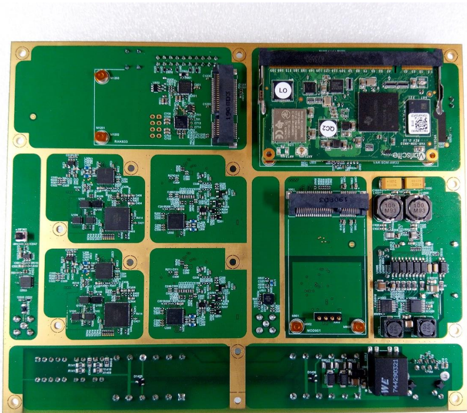
Bottom side of the PCB Main Board without shields and labels
