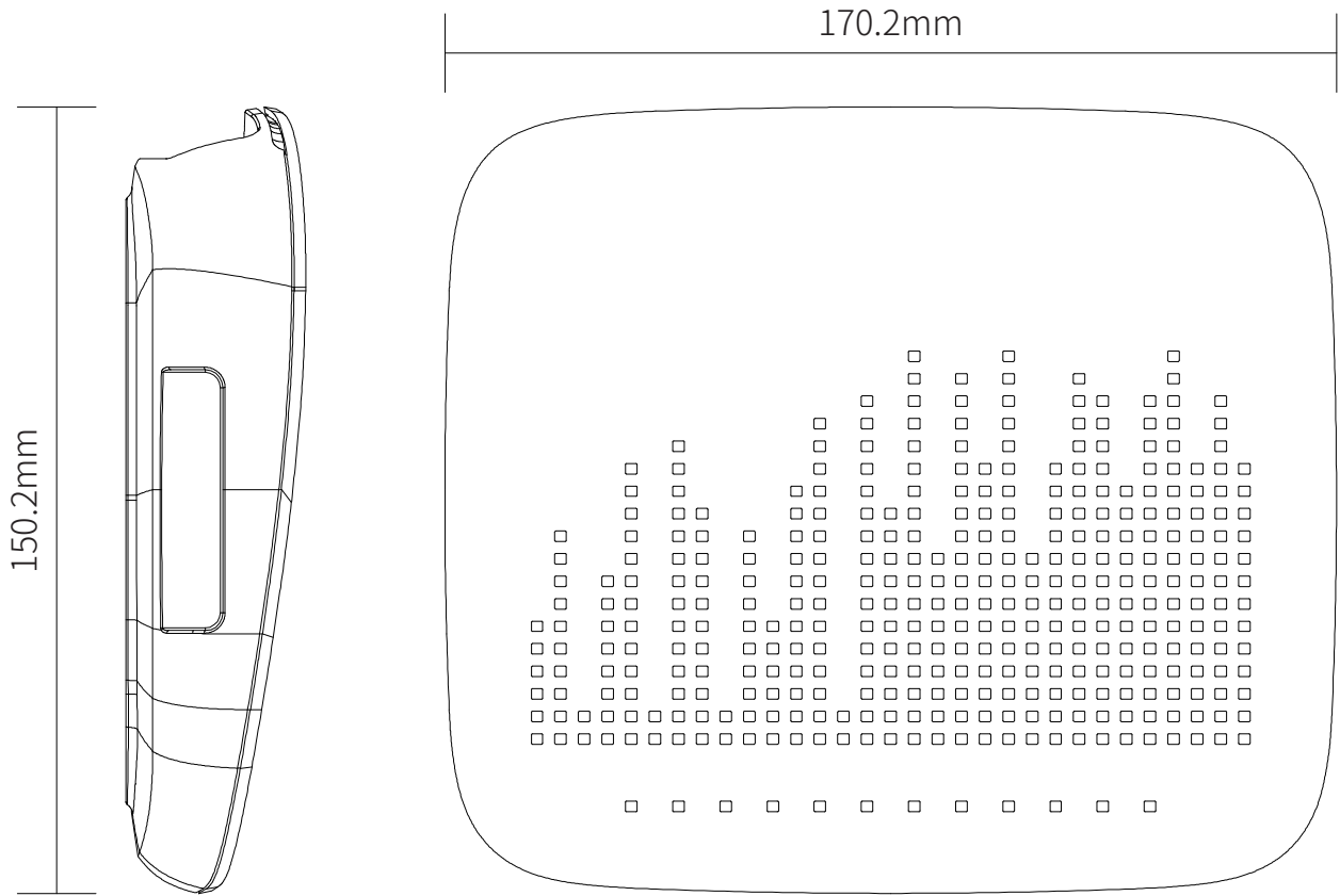
Left view
