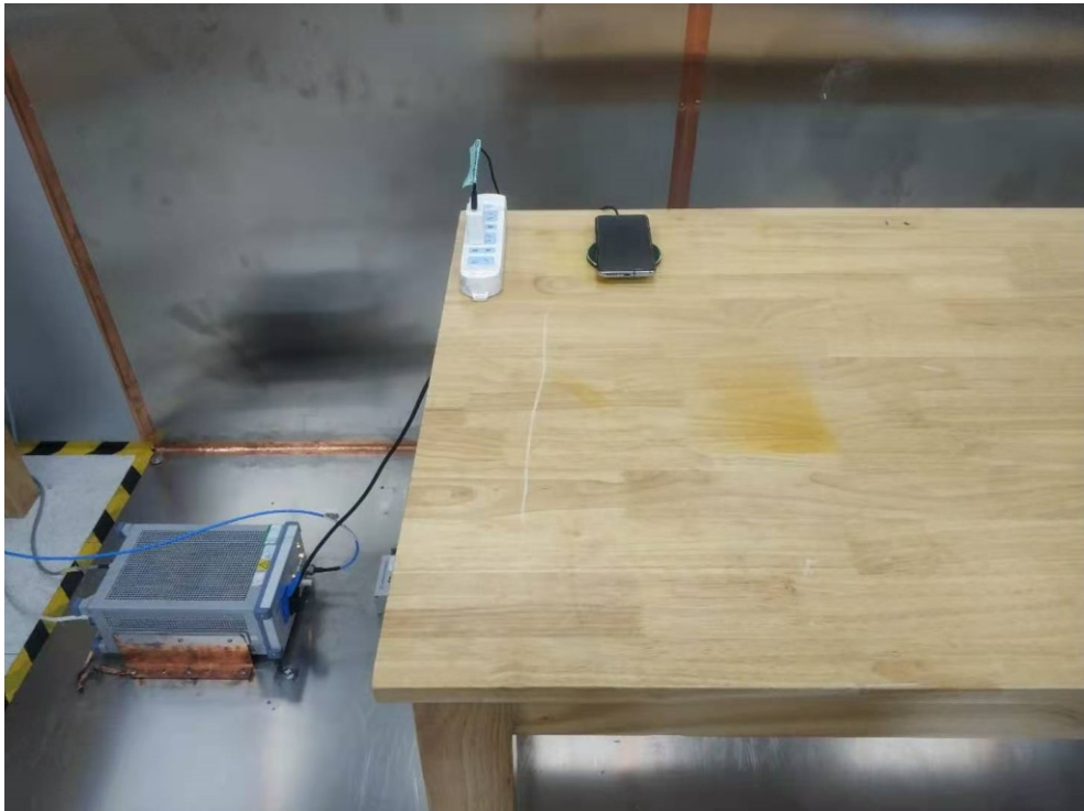
Photograph 3: Set-up photo for AC Conducted Emission, 150KHz-30MHz
